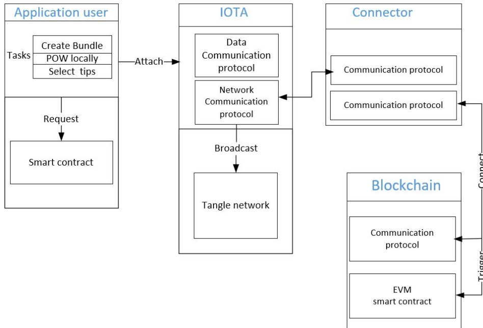
Fig. 4.2 Functional architecture
