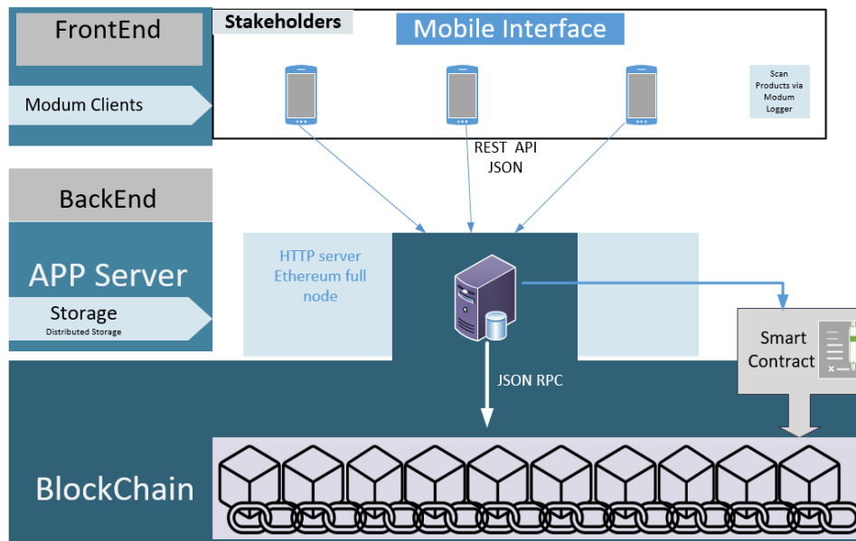
Fig. 3.5 Modum architecture
