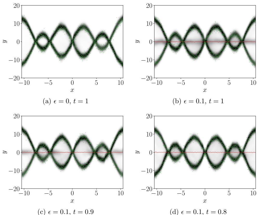
Figure 6.5: Ensemble predictive distribution obtained minimizing different free energy criteria. The samples from the ID measure are represented as green dots, while data points sampled from the OOD component are in red. The optimized predictive distributions are displayed in shades of gray. In (a), we plot the predictive distribution associated to (m, 1) -robust Bayesian learning obtained minimizing the m -free energy criterion \mathcal{J}^m of [3] with m = 20 by using only samples from the ID measure (i.e., there are no outliers). In (b), we show the predictive distribution obtained by minimizing the same criterion when using samples from the ID measure and OOD measure with a contamination ratio \epsilon = 0.1 . In (c) and (d) we consider the same scenario as in (b), but we consider the proposed (m, t) -robust Bayesian based on the robust m -free energy criterion \mathcal{J}_t^m with m = 20 , when setting t = 0.9 and t = 0.8 , respectively.
