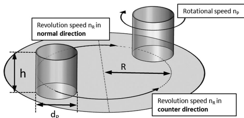
Figure 1.6: Schematic representation of a planetary ball mill. From [57].
