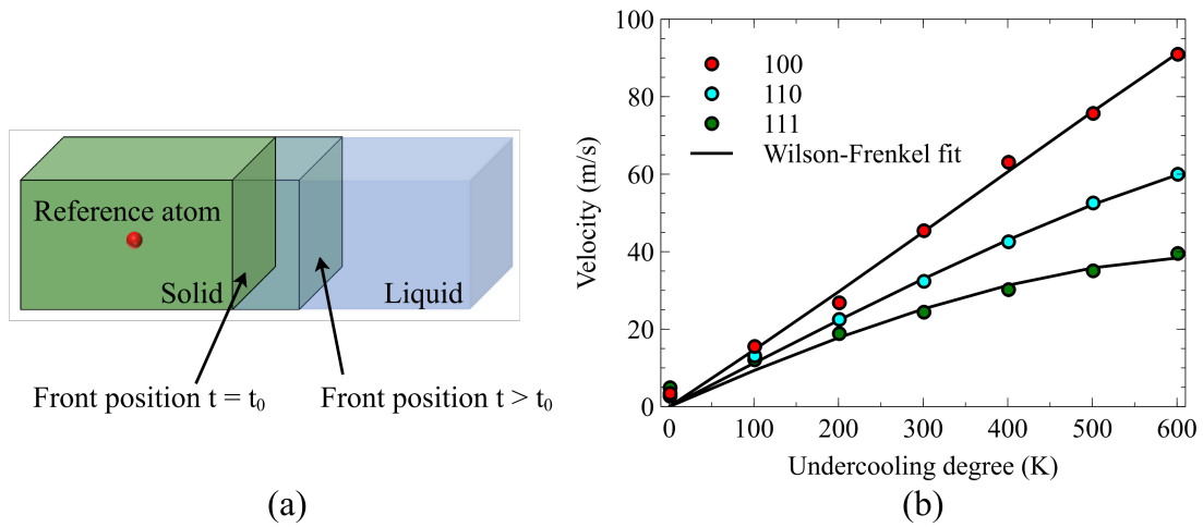
Figure 2.9: (a) Schematic representation of the system. (b) Solid/liquid interface velocity of the three orientations (100), (110), and (111) as a function of the degree of undercooling.
