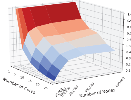
E1C-FastBC algorithm
