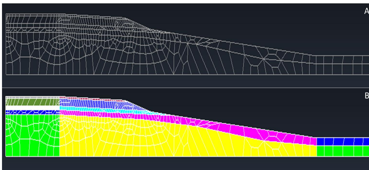
Figure 6-4. A) Modeling of the Baie-Comeau slope. B) Integration of the different sedimentary layers (seismic units 3 to 5 and the basement) with their geomechanical characteristics.
