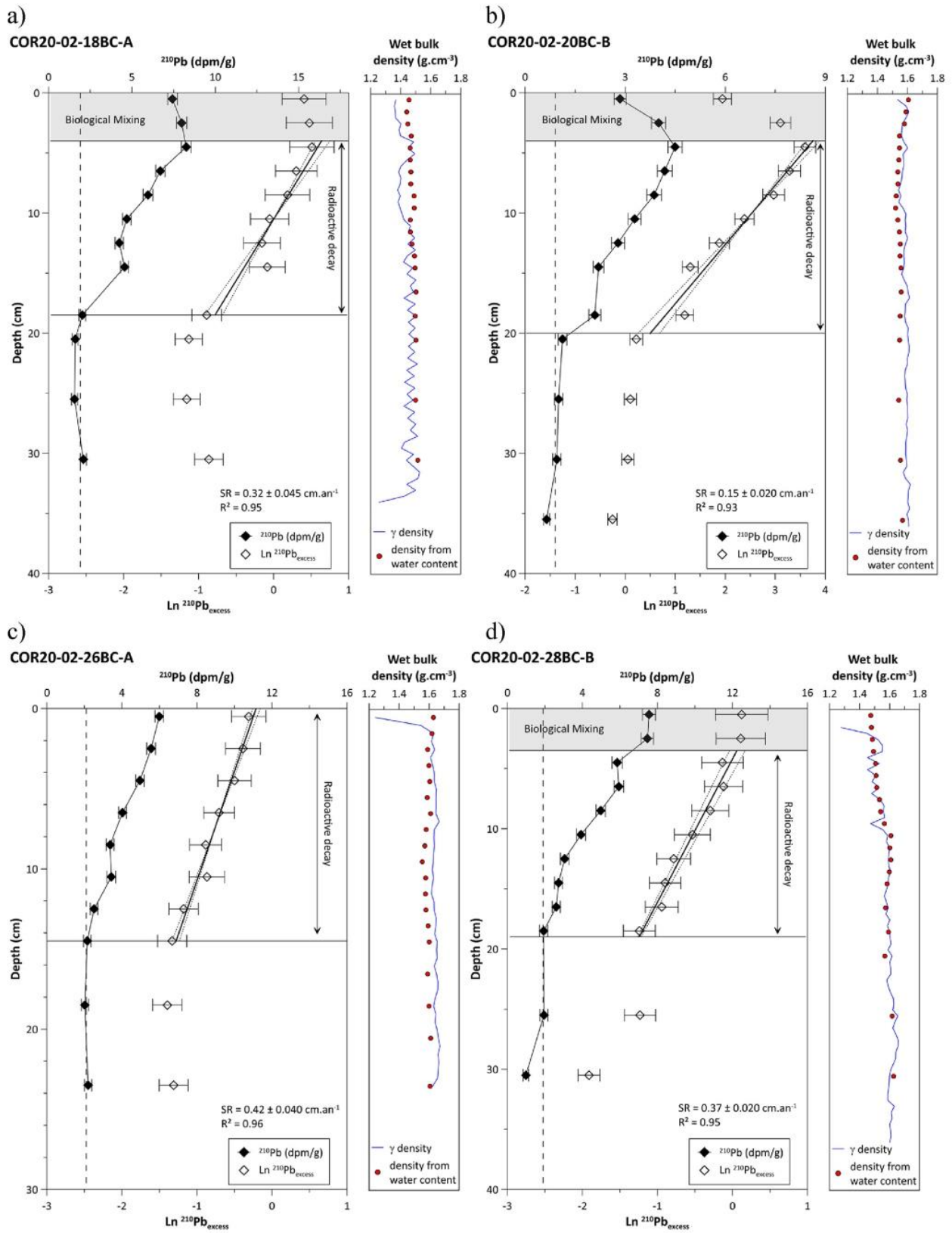
Fig. 8. Sedimentation rates (SR) calculated with the ^{210}\text{Pb} activity in cores COR20-02-18BC-A (SR = 0.32 \text{cm}\cdot\text{yr}^{-1} , a), COR20-02-20BC-B (SR = 0.15 \text{cm}\cdot\text{yr}^{-1} , b), COR20-02-26BC-A (SR = 0.42 \text{cm}\cdot\text{yr}^{-1} , c) and COR20-02-28BC-B (SR = 0.37 \text{cm}\cdot\text{yr}^{-1} , d). SR are calculated from the slope of \text{Ln}(^{210}\text{Pb}_{\text{excess}}) in the radioactive zone by excluding the biological mixing.
