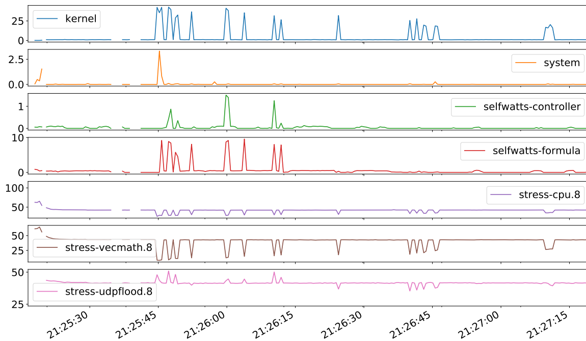
Fig. 4.4 Power estimations per VM for PARALLEL phase
