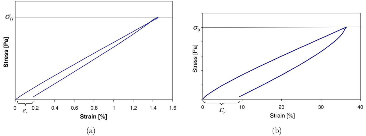
Figure 1.36: Measured stress-strain curves. (a) Assumed elastic behavior, \varepsilon_r < 0.2\% . (b) Assumed inelastic behavior, \varepsilon_r > 0.2\% [29].
