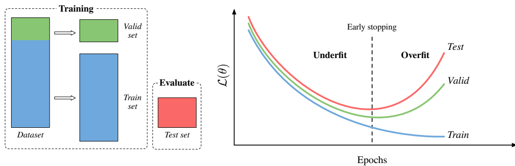
Figure 8: Separation of the dataset and typical evolution of the corresponding losses on each subset to avoid overfitting.
