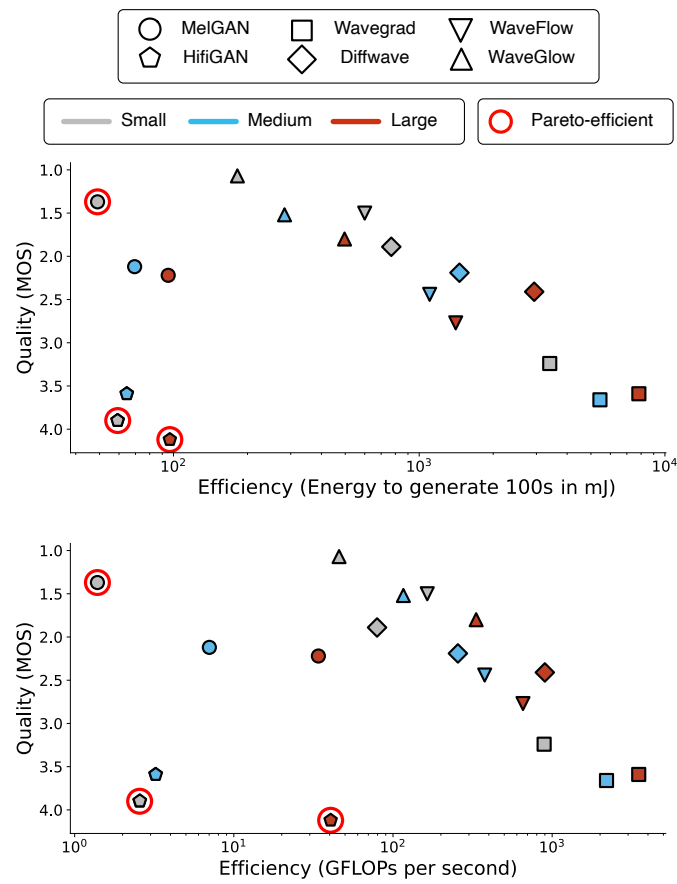
Figure 34: Representation of Pareto Frontier for efficiency vs quality. The objective is to maximize the quality (MOS) and minimize the energy cost of inference (top) and the number of GFLOPs (bottom).
