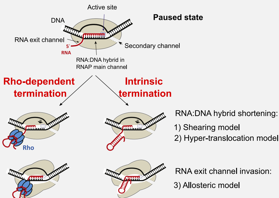
Figure 2-10: Transcription termination in bacteria.
