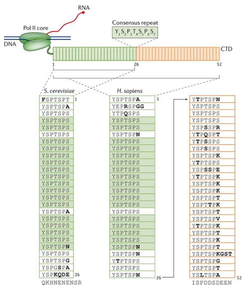
Figure 2-3: The composition and conservation of the CTD.
