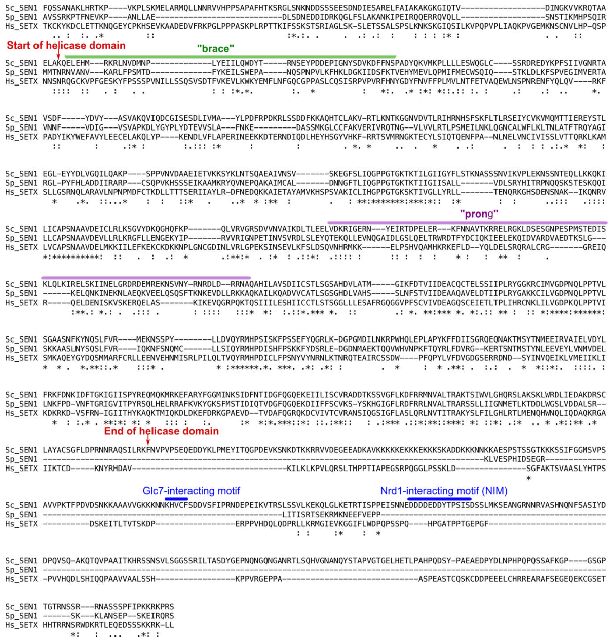
Figure S10: Alignment of the amino acid sequence of Sen1 proteins from different organisms.
