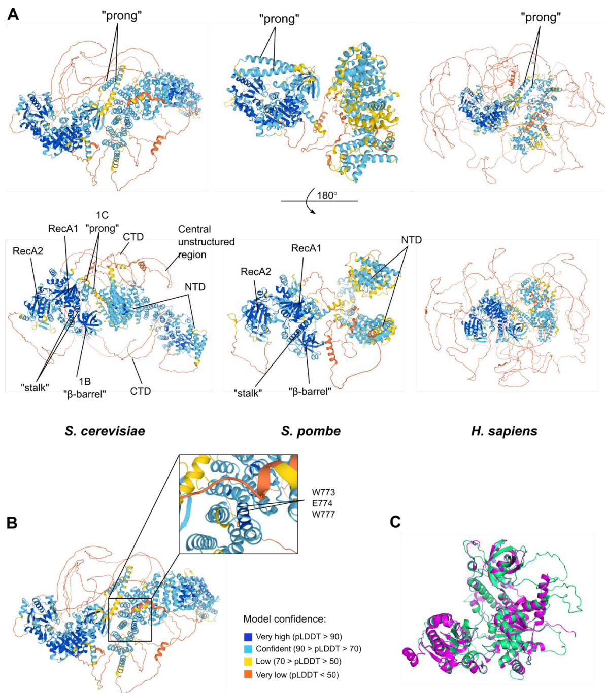
Figure S11: Structure of various Sen1 proteins predicted with AlphaFold .
