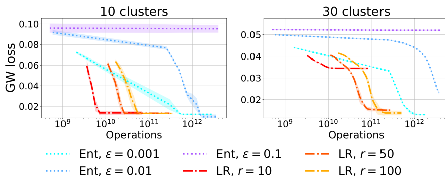
Figure 7.4: We sample n = m = 5000 points from two anisotropic Gaussian blobs, respectively in 10 and 15-D, with either 10 or 30 clusters, endowed with the Euclidean distance. We compare our quadratic method LR with the cubic Entropic GW Ent , which requires instantiating matrices A and B . We vary both r (our method) and \varepsilon (entropic). Our method obtains similar GW loss, while being orders of magnitude faster. Note the gap in performance between r = 10 and r = 50 when the input measures have 30 clusters: the GW loss decreases as the rank r increases until it reaches the number of clusters in the data.
