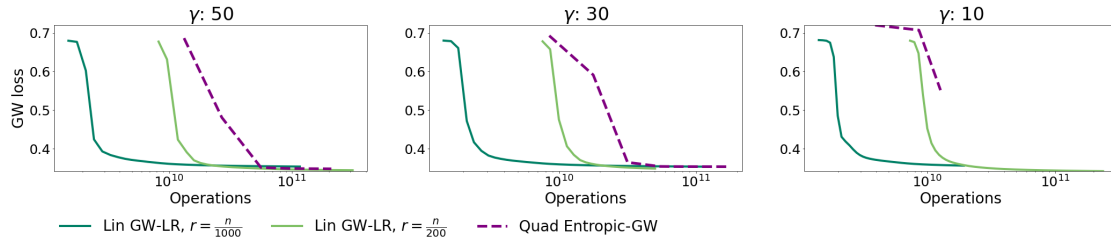
Figure 7.10: Here n = m = 10000 , and the ground cost considered is the squared Euclidean distance. Note that for in that case we have an exact low-rank factorization of the cost. Therefore we compare only Quad Entropic-GW and Lin GW-LR . We plot the time-accuracy tradeoff when varying \gamma for multiple ranks r . \varepsilon = 1/\gamma for Quad Entropic-GW and \varepsilon = 0 for Lin GW-LR .
