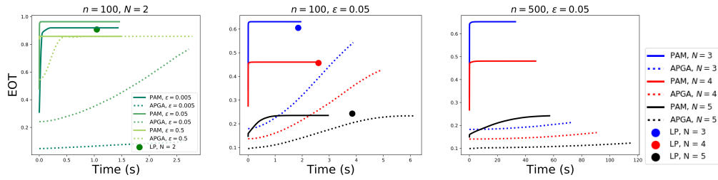
Figure 8.3: Comparison of the time-accuracy tradeoffs between the different proposed algorithms. Left: we consider the case where the number of days is N = 2 , the size of support for both measures is n = m = 100 and we vary \varepsilon from 0.005 to 0.5. Middle: we fix n = m = 100 and the regularization \varepsilon = 0.05 and we vary the number of days N from 3 to 5. Right: the setting considered is the same as in the figure in the middle, however we increase the sample size such that n = m = 500 . Note that in that case, LP is too costly to be computed.
