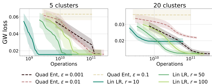
Figure 7.7: Setting as in Fig. 7.4, with n = m = 10000 samples from anisotropic Gaussian blobs of 5 or 20 clusters, endowed with the squared Eucl. distance. We compare Lin LR and Quad Ent using exact factorizations of A and B .
