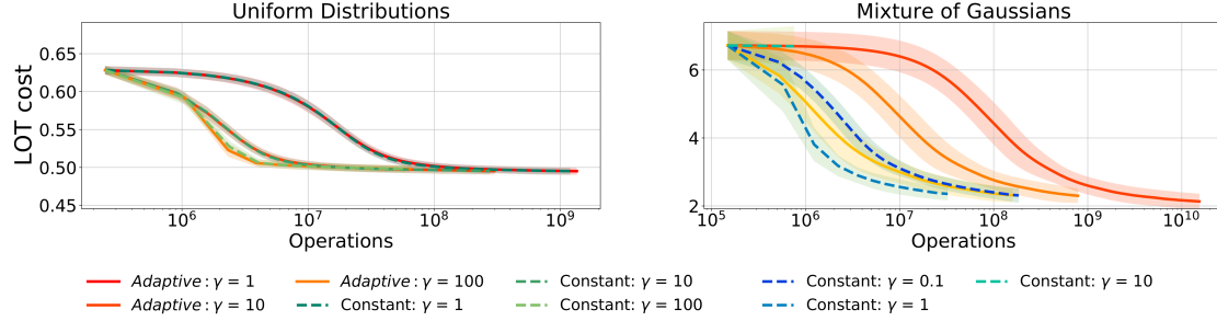
Figure 6.5: In this experiment, we compare two strategies for the choice of the step-size in the MD scheme proposed by [3] on two different problems. More precisely, we compare the constant \gamma schedule with the proposed adaptive one and compare them when the distributions are sampled from either uniform distributions ( left ) or mixtures of anisotropic Gaussians ( right ). We show that the range of admissible \gamma when considering a constant schedule varies from one problem to another. Indeed, in the right plot, we observe that the algorithm converges only when \gamma \leq 1 , while in the left plot, the algorithm manages to converge for \gamma \leq 100 . We also observe that our adaptive strategy allows to have a consistent choice of admissible values for \gamma whatever the problem considered. It is worth noticing that whatever the \gamma chosen, the algorithm converges towards the same value, however the larger \gamma is chosen in its admissible range, the faster the algorithm converges.
