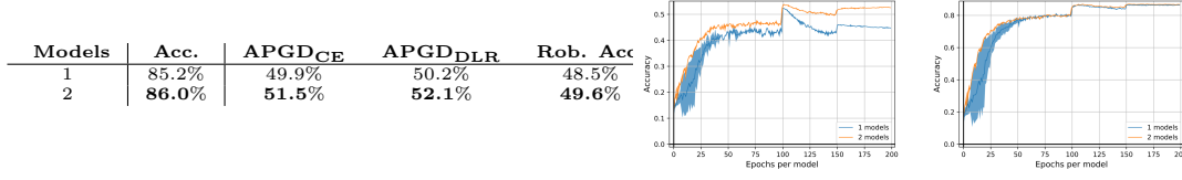
Figure 9.5: On left: Comparison of our algorithm with a standard adversarial training (one model) on WideResNet28x10. We reported the results for the model with the best robust accuracy obtained over two independent runs because adversarial training might be unstable. Standard and Robust accuracy (respectively in the middle and on right) on CIFAR-10 test images in function of the number of epochs per classifier with 1 and 2 WideResNet28x10 models. The performed attack is PGD with 20 iterations and \varepsilon = 8/255 .
