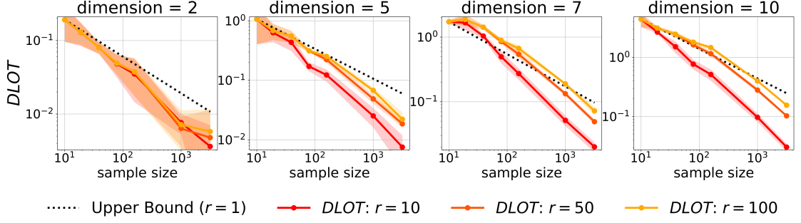
Figure 6.1: In this experiment, we consider a mixture of 10 anisotropic Gaussians supported on \mathbb{R}^d and we plot the value of DLOT_{c,r} between two independent empirical measures associated to this mixture when varying the number of samples n and the dimension d for multiple ranks r . The ground cost considered is the squared Euclidean distance. Note that LOT_r(\mu, \mu) \neq 0 and therefore we use DLOT_{c,r}(\mu, \mu) instead to evaluate the rates. Each point has been obtained by repeating 10 times the experiment. We compare the empirical rates obtained with the theoretical one derived in Proposition 6.4.2 for r = 1 . We observe that our theoretical results match the empirical ones and, as expected, the rates do not depend on d .
