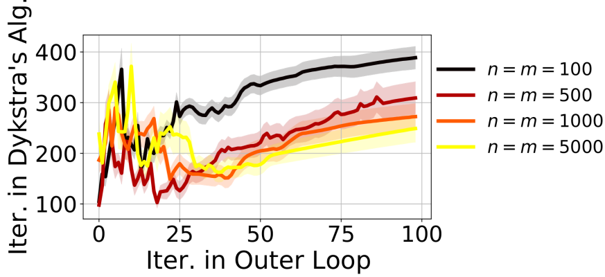
Figure 7.2: We consider samples of a mixture of 10 anisotropic Gaussians in resp. 10 and 15-D endowed with the squared Eucl. metric. The number of iterations of Dykstra’s algorithm required to reach a precision of \delta = 1e - 3 along the iterations of the Algo. 12 is not impacted significantly by varying n , the sample size.
