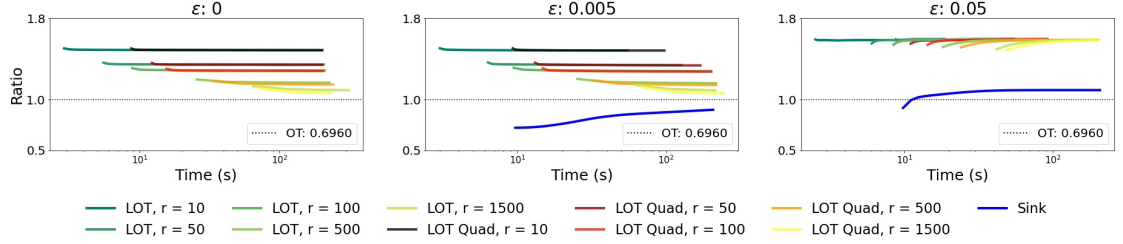
Figure 5.9: Comparison of the time-accuracy tradeoff for different methods for estimating the OT or its regularized version between two mixture of gaussians in 10D.
