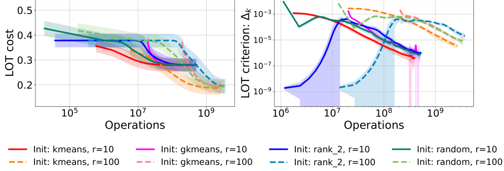
Figure 6.4: In this experiment, we consider the NewsGroup20 dataset [213] constituted of texts and we embed them into distributions in 50D using the same pre-processing steps as in [214]. We compare different initialization when applying the algorithm of [3] to compare random texts viewed as distributions for multiple choices of rank r . The ground cost considered in the squared Euclidean distance. We repeat the experiments 50 times by sampling randomly multiple problems of similar size ( \simeq 250 samples). We normalize the cost matrix by its maximum value in order to have comparable LOT cost. We consider 4 different initialization: the one using k -means algorithm (6.9), the one using the generalized k -means (6.10), the rank-2 initialization [3] and a random initialization where Q , R and g are drawn from Gaussians. We compare both the cost value and the criterion value ( \Delta_k ) along the iterations of the MD scheme. Note that the curves obtained do not start at the same point in time as we start plotting the curves after obtaining the initial point which in some case requires more algebraic operations (e.g. kmeans methods). First we observe that whatever the initialization considered, the algorithm converges toward the same value. In addition, we observe that both k -means and general k -means are able to initialize well the algorithm by avoiding bad local minima at initialization while the two other initialization are close to spurious local minima at initialization.
