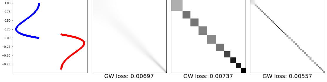
Figure 7.14: We compare the couplings obtained when the ground truth is the identity matrix in the same setting as in Figure 7.10. Here the comparison is done when \gamma = 250 . Left : illustration of the dataset considered. Middle left : we show the coupling as well as the GW loss obtained by Quad Entropic-GW . Middle right, right : we show the couplings and the GW losses obtained by Lin GW-LR when the rank is respectively r = 10 and r = 100 .
