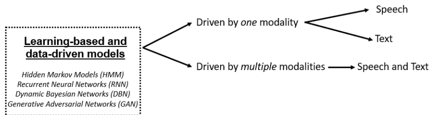
Figure 1.3 Learning-based approaches
