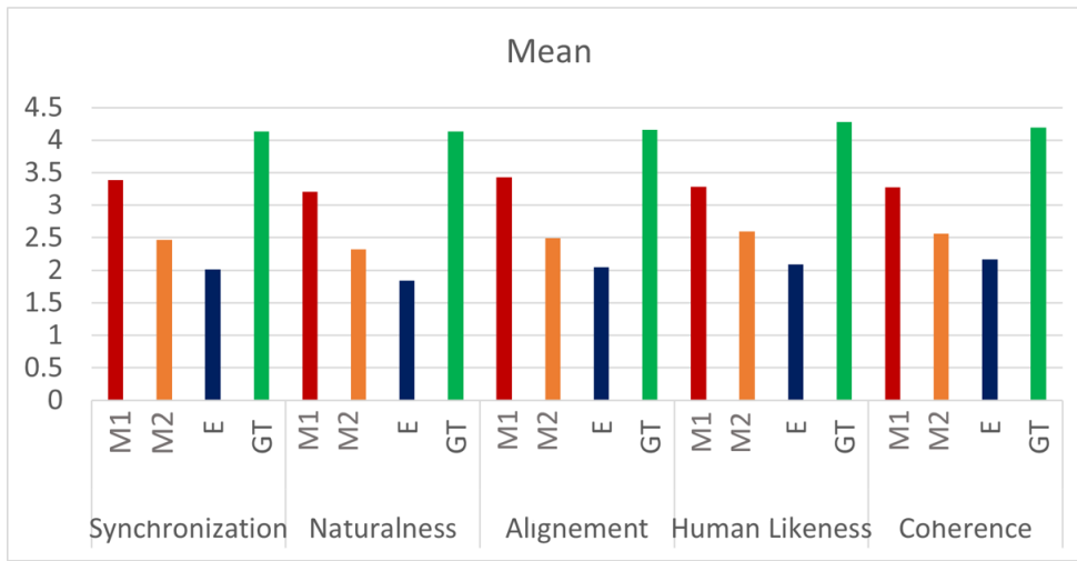
Figure 5.6 Subjective evaluation results obtained on the SpeakerDependent ( SD ) set to assess the naturalness , human-likeness , and coherence of the predicted gestures, as well as the synchronization and alignment of the gestures with the speech. The assessment was conducted for the 4 conditions: Model 2 denoted by M2 , Model 1 baseline denoted by M1 , the ground truth GT , and the error condition E
