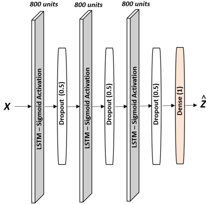
Figure 7.3 Classifier Architecture
