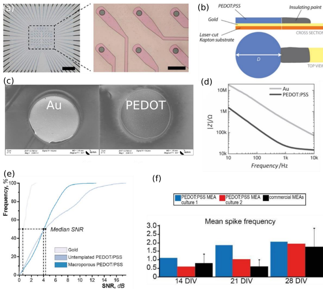
Figure 1.15 PEDOT:PSS MEAs. a) PEDOT:PSS based microelectrode array for simultaneous electrical and optical measurements of primary neuron cultures. Scale bars: left, 1cm; right: 100 μm. Adapted from [771] b) schematic showing the coating of PEDOT:PSS on top of flexible Kapton electrode [72]. c) SEM images showing coated PEDOT:PSS on top of bare gold microelectrode. Left: bare gold (Au) before coating, right: after coating PEDOT:PSS. d) Impedance modulus as function of frequency for gold and PEDOT:PSS electrode showing the notable lower impedance for PEDOT:PSS electrode [56]. e) Cumulative frequency plot showing the distribution of SNR for gold, PEDOT:PSS and macroporous PEDOT:PSS microelectrodes showing superior SNR values for PEDOT [64]. f) Mean spike frequency for two PEDOT:PSS base MEA (blue and red) and commercial TiN based MEA (black) at 14, 21 and 28 day in vitro (DIV) showing higher firing rate of the PEDOT:PSS MEA in comparison to the commercial one reassuring proper maturation of the neural network [57].
