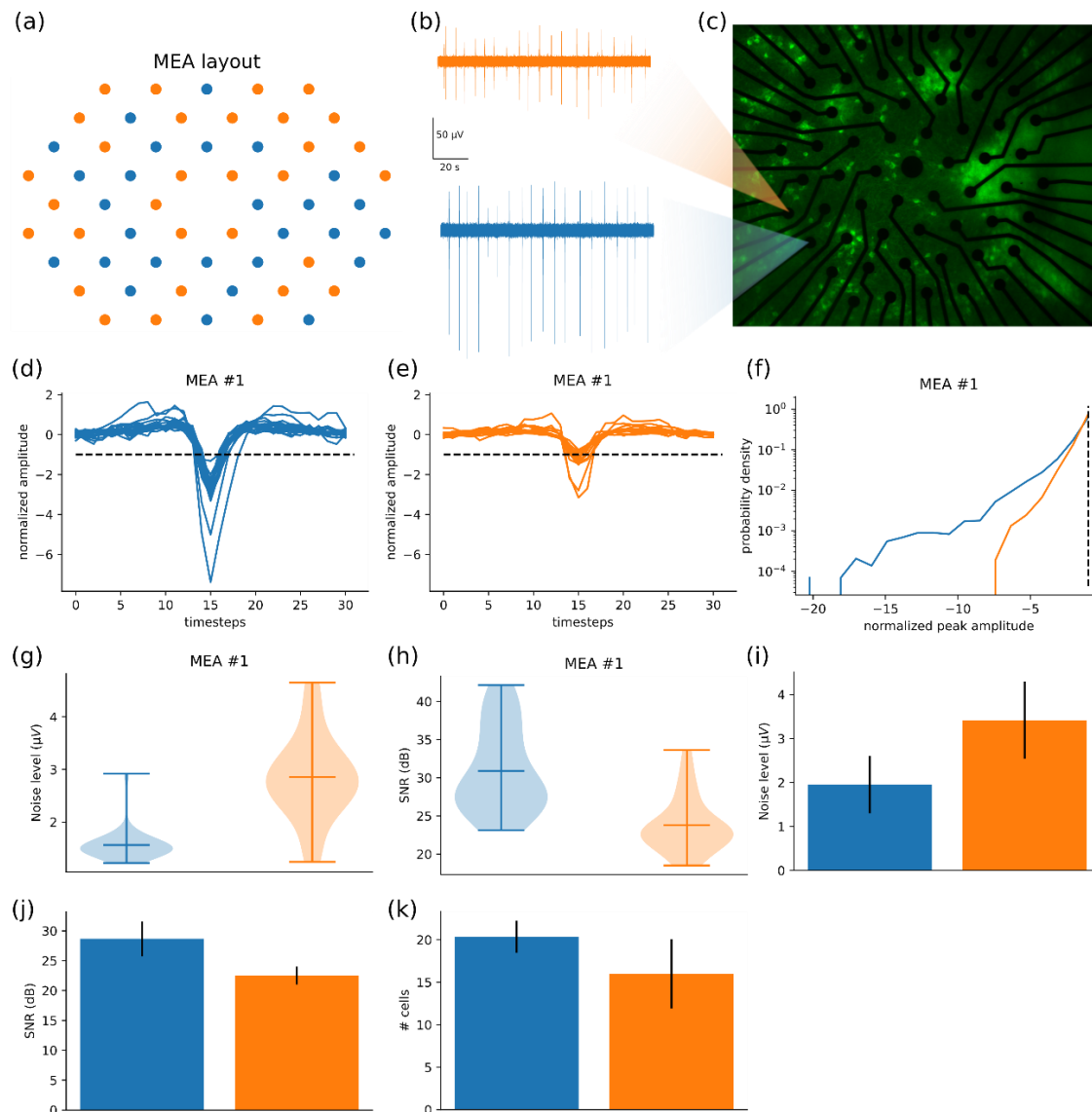
Figure 3.5 Effect of PEDOT coating on cell detection. (a) The layout of the MEA, and the patterning of the coated vs non-coated channels. (b) Time series showing spontaneous burst-spike activities of a neural culture at DIV21 from a gold electrode and coated ePEDOT electrode on the same MEA number 1.(c) Live-imaging of primary cortical neurons on top of the MEA, after 21 days in vitro (DIV21).Note that only live neurons are detected by the fluorescent probe we used. (d) Canonical waveforms obtained for spiking neurons, over coated channels, and. (e) non-coated channels of MEA number 1. (f) Probability density of the normalized peak amplitudes over all channels of MEA number 1, sorted by types (coated vs non-coated). (g) Violin plot chart showing the noise levels obtained over all channels of MEA number 1, sorted by types (coated vs non coated). (h) Violin plot chart showing the Signal to Noise ratio (SNR) over all channels of MEA number 1, sorted by types (coated vs non coated). Histograms showing the (i) noise levels and (j) SNR values obtained over all channels averaged over three different MEAs, sorted by types (coated vs non coated). Error bars show standard deviations (k) Histogram showing the number of cells detected after spike sorting whose template peaks are on coated or non-coated channels averaged three different MEAs (three different cell cultures). Error bars show standard deviations.
