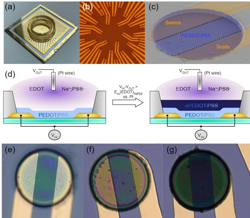
Figure 5.1 Electropolymerization technique for OECTs. (a) OEECT glass chip. (b) Microscopic image of the array of 30 OEECTs. (c) Colorized SEM image for a PEDOT:PSS OEECT. (d) Schematic representation showing the experimental setup to perform potentiostatic electropolymerization of EDOT on top of spin-coated PEDOT:PSS OEECT. (e-g) Microscopic images (from left to right) of spin-coated PEDOT:PSS OEECT, spin-coated and electropolymerized PEDOT at 0.6 V, spin-coated and electropolymerized PEDOT at 0.7 V. [Figure published in Ghazal et al. Adv Electron Mater 8(3), 2100891 (2022)].
