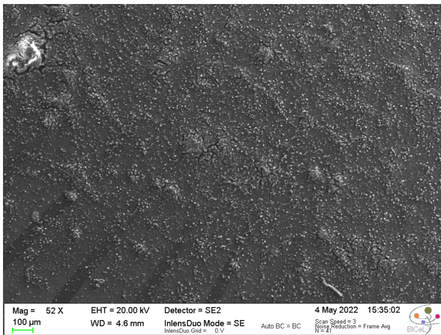
Figure 6.17 SEM image of dense neural network cultured on top of the OEET array for in vitro electrical recordings
