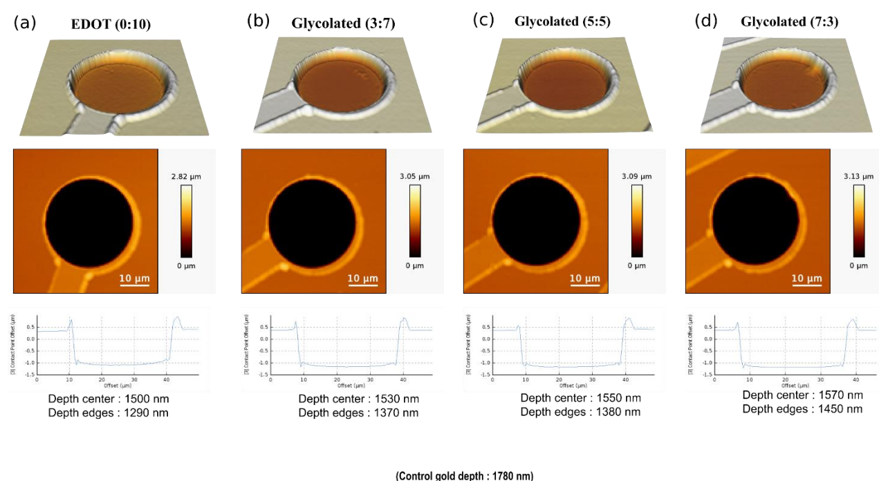
Figure 4.3 (a) Topography and profilometry experiments of a micro-electrode coated with (a) ePEDOT, (b) glycolated ePEDOT (3:7), (c) glycolated ePEDOT (5:5) and glycolated ePEDOT (7:3) at 1.4 V DC for 8 seconds, recorded by Atomic Force Microscopy (AFM) in Phosphate Buffer Saline (PBS). Control depth of gold microelectrode: 1780 nm. This control will be used to calculate the thickness of each material (Table 4.2).
