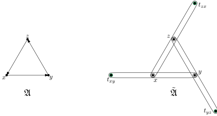
Figure 4.3: An example of Construction 8.
