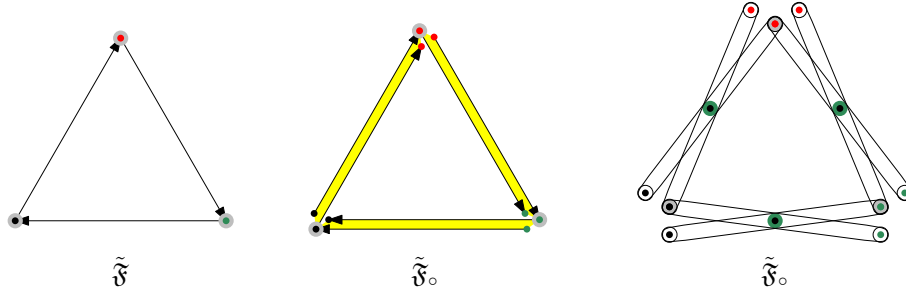
Figure 4.11: Suppose that \mathfrak{F} is a triangle ( e.g. \mathfrak{C}_3 ). Its \tilde{\mathbf{D}} -image \tilde{\mathfrak{F}} is as on the left. There are two ways to represent the structure \tilde{\mathfrak{F}}_{\circ} : as in the middle and as on the right. In the middle, yellow zones between two arcs highlight pairs of duplicated \tilde{\mathbf{R}} -tuples, and, for convenience, \mathbf{T} -vertices are not displayed in the middle. However, the figure on the right contains \mathbf{T} -vertices, they are denoted by green disks. The relation \text{Old} is marked on both figures with grey disks. Red, green and black dots inside white circles represent \tilde{\sigma}_{\mathbf{V}} -coloured \mathbf{V} -vertices.
