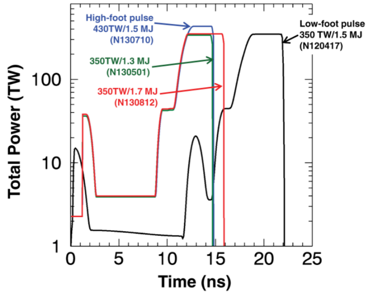
Figure 1.8: Profile of laser power delivered in the hohlraum during a low-foot pulse (black) and three high-foot pulses (red, green and blue). The high-foot pulses are shorter, and deliver more power at the beginning of the pulse (before 10 ns in the graph). Image credit: Park et al. [2014]
