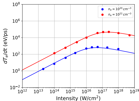
Figure 4.1: Heating rate for both plasmas described in eq. (4.5) and eq. (4.6) at different intensities measured at early time to ensure that EVDs have not yet transitioned to non-Maxwellian which is the hypothesis of the parametrized model developed in chapter 3. The coefficients of the model are those adjusted in chapter 3 by CMDSs at Z = 1 and one can see that the agreement is excellent even for Z = 10 .
