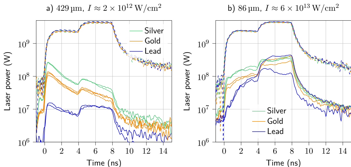
Figure 6.5: Power incident (dashed) and reflected (solid) versus time for silver, gold and lead target, for the staircase pulse shape, and a 429\ \mu\text{m} focal spot (left) and a 86\ \mu\text{m} focal spot (right). The values on top of the graphs give the magnitude of the intensity reached during each shot. For each shot, the corresponding reflected power is the solid line of the same color. Multiple shots are shown for each material, to show repeatability. The first half of the pulse is identical to the 10 J single step pulse, so it follows that the reflected power is the same as in Fig. 6.2. In the second half of the pulse and for the 429\ \mu\text{m} focal spot, the reflectivity does not seem to change behaviour, and still seem to decrease with the same slope. Since the incident power doubles at mid-pulse, the reflected power also doubles. For the 86\ \mu\text{m} focal spot, the behaviour of the reflected power is reminiscent of the behaviour during the long pulse, which was shown in Fig. 6.3, where the reflected power reaches a steady value.
