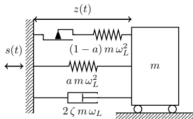
FIGURE 3.4: Elasto-plastic mechanical oscillator with kinematic hardening, with parameters f_L = 5 Hz and \zeta = 2\% . The yield limit is Y = 5 \cdot 10^{-3} m and the post-yield stiffness is 20% of the elastic stiffness, hence a = 0.2 .
