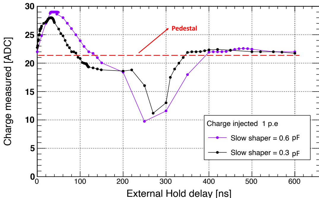
Figure 3.29: Measured charge as a function of the external Hold Delay for 1 p.e injected charge for two slow shaper settings.
