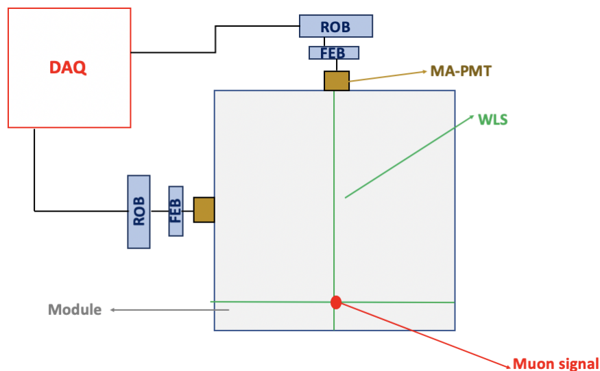
Figure 3.46: XY Coincences projection in a layer. A signal is observed in a strip channel oriented in the Y direction (left card). This signal propagates in a wavelength shifting fiber and is read by the MA-PMT. The same procedure is identified for another signal in the X direction (right card). Each signal is identified by its charge, time and position.
