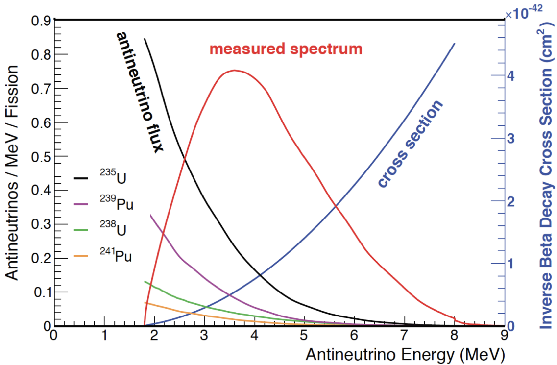
Figure 2.4: The observable electron antineutrino spectrum (red line) is a product of the antineutrino flux from reactor and the cross section of inverse beta decay (blue line). The contributions of four fission isotopes to the antineutrino flux are shown [104].
