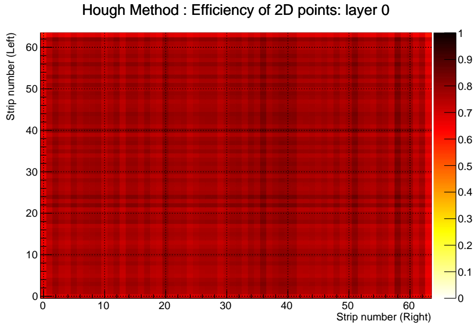
Figure 4.24: The MT detection efficiencies of 2D points provided by the Hough Method for the layer 0 using simulation data.
