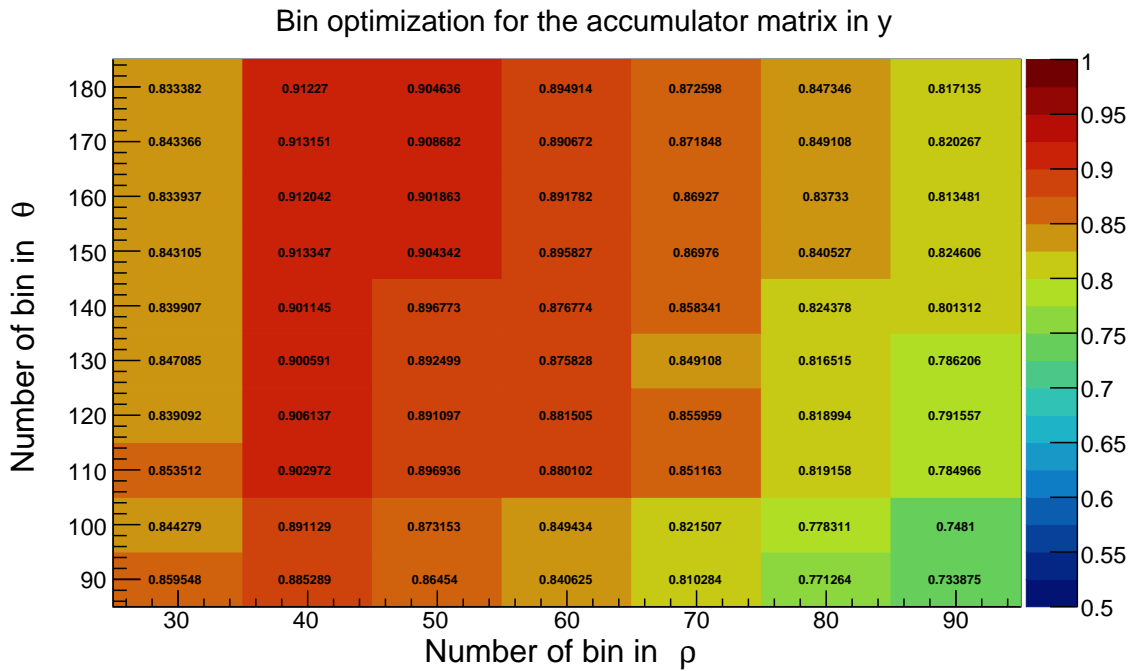
Figure 4.21: Binning accumulator matrix for YZ projection. The best pixel for YZ is found in (40,150) which corresponds to a bin size of (4.9 cm , 0.93°), where around 91% of the tracks were reconstructed.
