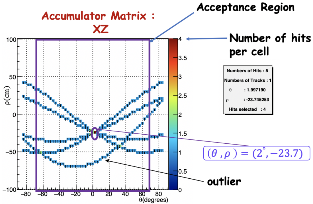
Figure 4.12: Accumulator matrix of the Hough transform using the sample of channels triggered in the XZ projection of Fig.4.11. In the horizontal axis ( \theta_x ) varies between (-90^\circ, 90^\circ) , an angular acceptance region is defined in the interval (-70^\circ, 70^\circ) . This is imposed by the condition of having hits in at least 3 MT layers. For the vertical axis ( \rho_x ) varies between (-100\text{cm}, 100\text{cm}) . The value of \rho is given by the geometry of the detector. In this accumulator matrix, five sinusoidal curves are represented. The maximum number of hits per cell varies between 0 and 4. In most cases the sinusoidal curves do not cross. In four cases two sinusoidal curves intersect. The accumulator matrix shows that in the cell (2^\circ, -23.7\text{ cm}) four hits are collinear which corresponds to four sinusoidal curves intersecting. An outlier is recorded in layer 2.
