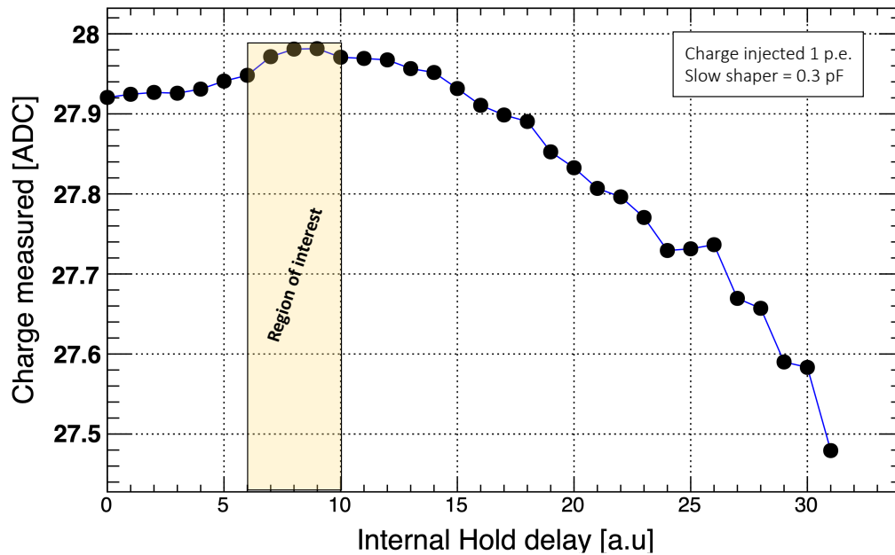
Figure 3.31: Measured charge as a function of the internal Hold Delay for 1 p.e injected charge for a slow shaper of 0.3 pF.
