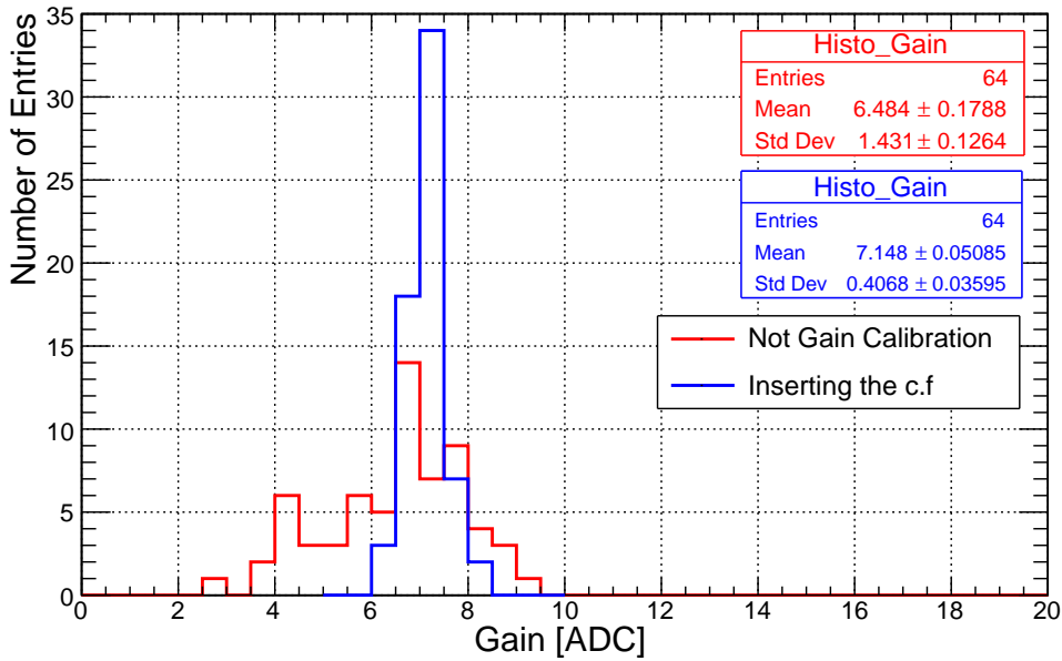
Figure 3.26: Gain distribution before and after inserting the amplification factors for the C2R.
