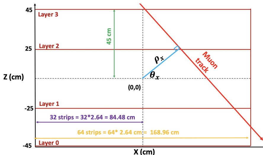
Figure 4.10: Cartesian space definition of the MT for the XZ projection.
