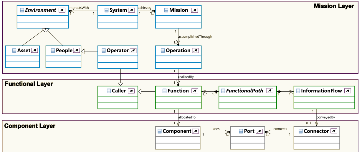
Figure 4.5: Three-layered System Meta-model.
