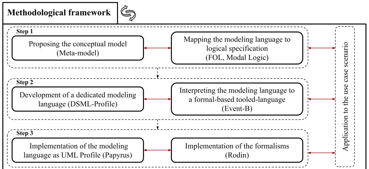
Figure 3.7: Methodological Framework.
