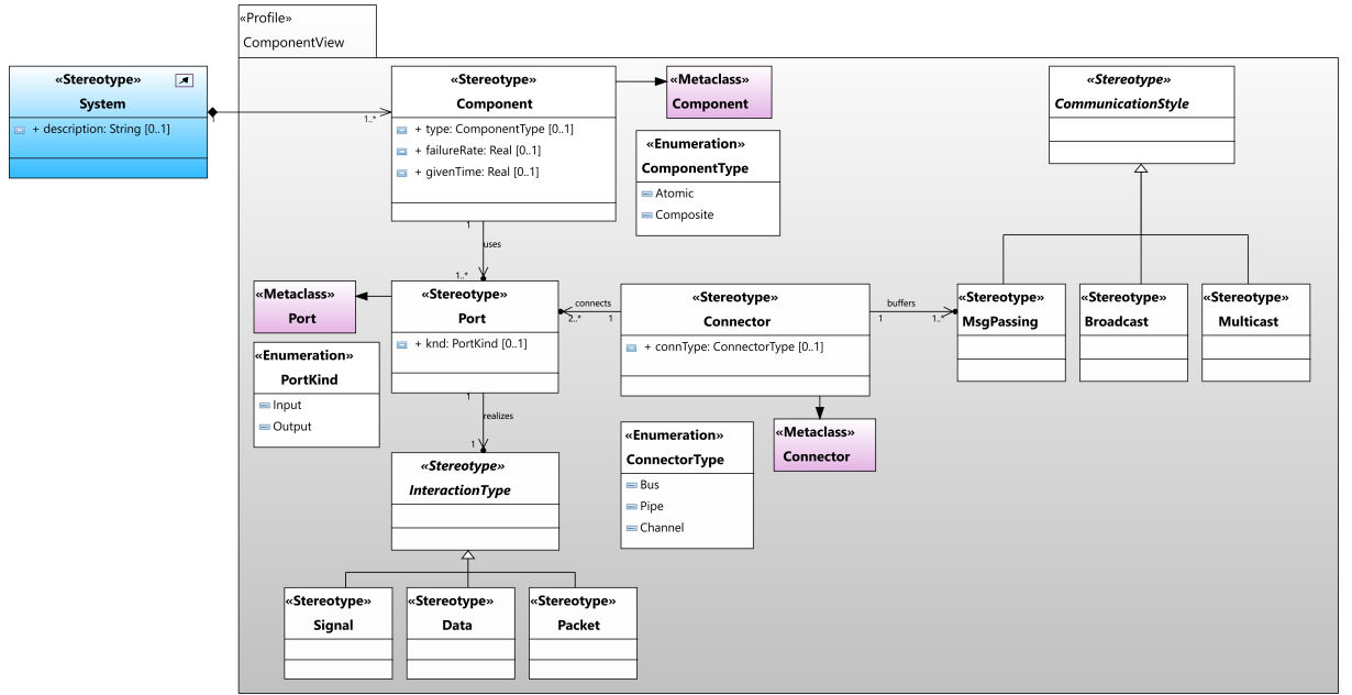
Figure 4.8: Component-layer System UML Profile.
