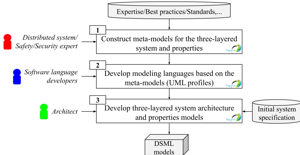
Figure 4.14: Tool Support for Modeling.
