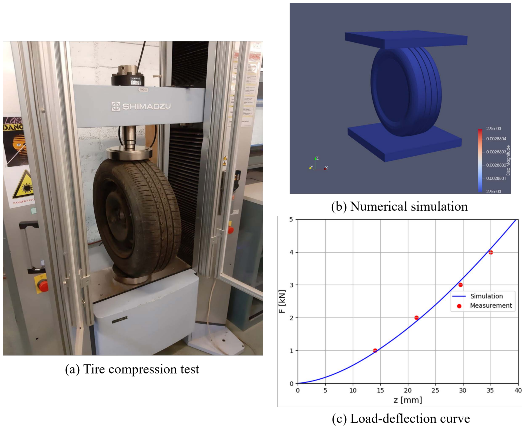
Figure 5.3: Comparisons between measured and calculated tire deflections
