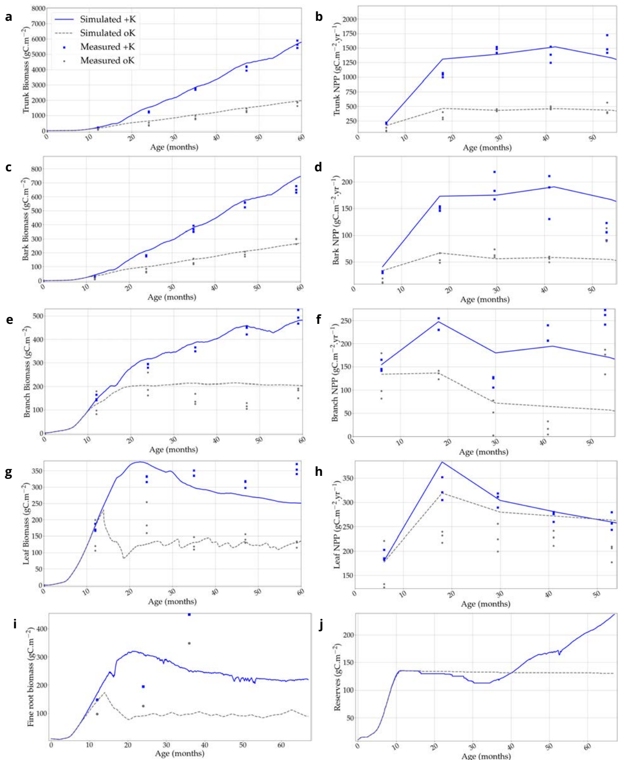
Figure 2: Simulated biomass of the different organs in two contrasted K availability scenarios (no K fertilisation, oK , and full K fertilisation, +K ): a) trunk, c) Bark, e) Branches, g) Leaves, i) Fine roots and j) Reserves. On the right column, the respective measured and simulated annual NPP of each organ: b) trunk, d) Bark, f) Branches, h) Leaves.
