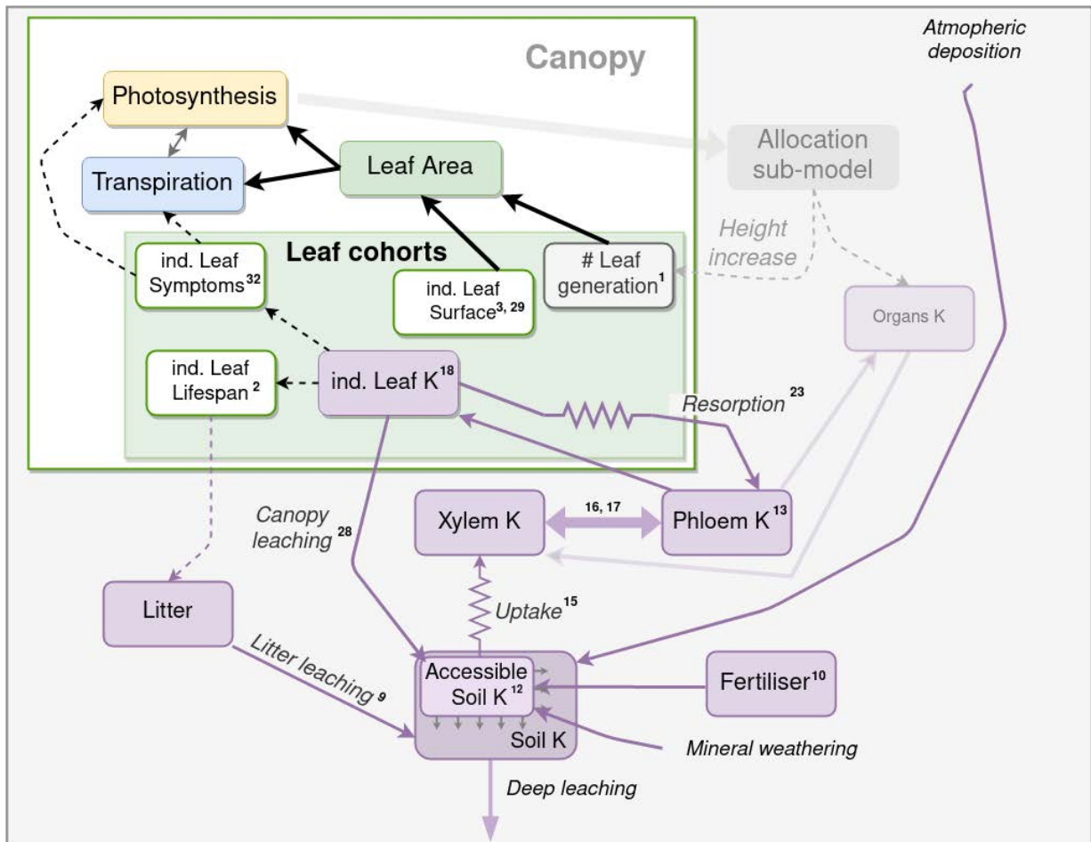
Figure 1: Schematic representation of the soil and plant parts of the K cycle, and their links with the leaf cohort model and other sub-models. Purple boxes are K state variables, and purple arrows are K fluxes. K fluxes simulated with a simple Ohm's law form are represented with resistance symbols. Black arrows represent a functional link a variable has on another variable or process. The numbers in exponent correspond to the number of the equation in the text.
