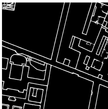
FIGURE 3.5: BDCN*
