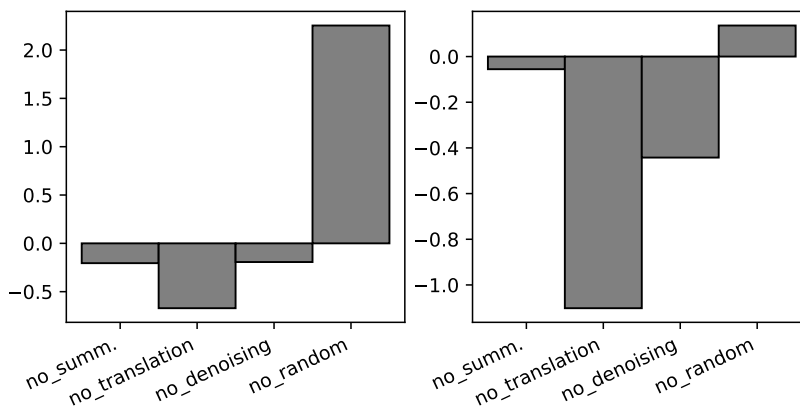
Figure 4.1 – Relative improvement in Pearson correlation compared to a dataset covering all sources. Left: TAC. Right: WMT.
