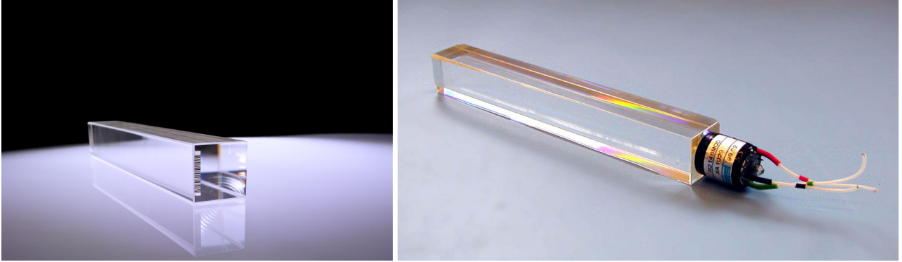
Figure 2.6: Picture of the ECAL PBWO_4 crystal. The right-hand side shows the photodetector on one of the crystals used in the ECAL endcap.
