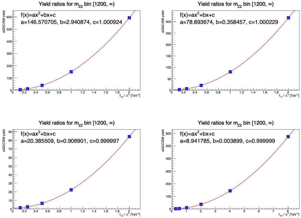
Figure 4.17: Yield ratios for a few values of the operator couplings obtained from the reweighing and the fitted quadratic interpolation for each of the mass bins used in the statistical analysis. The last bin of the m_{4l} distribution is shown for the f_{T0}/\Lambda^4 (top left), f_{T1}/\Lambda^4 (top right), f_{T2}/\Lambda^4 (bottom left) and f_{T9}/\Lambda^4 (bottom right) operators.
