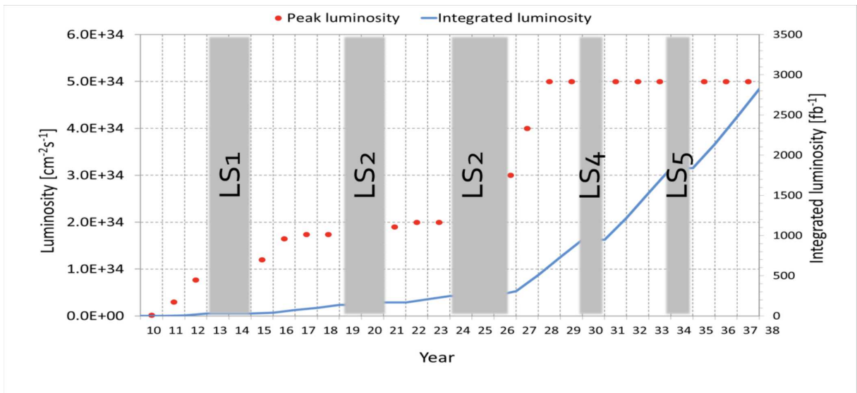
Figure 2.13: Projected LHC performance through 2038, showing preliminary dates for long shutdowns (LS) of the LHC and projected luminosities. Figure is taken from [70].
