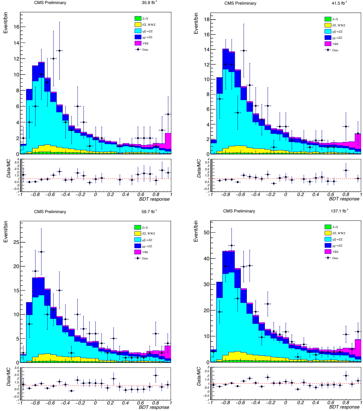
Figure 4.12: BDT output distribution for each contribution after the BDT7 training for the 2016 (top-left), 2017 (top-right) and 2018 (bottom-left) period together with the period-combined distribution (bottom-right). Each contribution is stacked on top of the previous one starting with the Z+X sample. Bottom: comparison between data and MC expectation.
