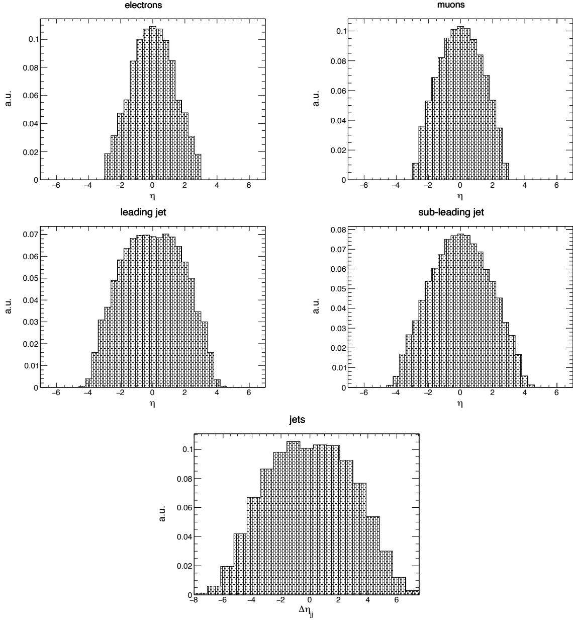
Figure 5.3: Top row: pseudorapidity spectrum of leptons. Middle row: pseudorapidity spectrum of the two leading jets. Bottom: the pseudorapidity difference spectrum between the two leading jets. Distributions for the signal sample, obtained before implementing the lepton-jet cleaning algorithm, are shown. Samples are simulated at 14 TeV c.o.m. energy and the baseline selection was applied.
