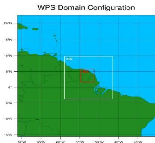
Figure 16: WRF nested domain ways, A large domain, the black square D01, with a resolution of 27 km, then the white one D02 with a horizontal resolution of 9 km the last domain is the red one D03 with a horizontal resolution of 3 km.
