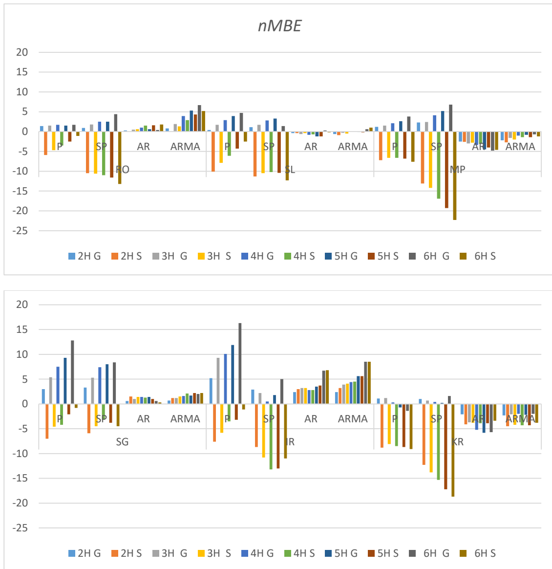
Figure 33: nMBE forecasting errors vs. time Horizon for Ground measurement (G), Satellite-derived data (S) with four statistical models in 2016 according to station.
