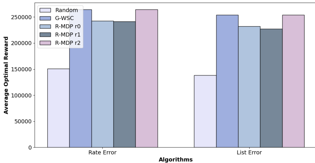
Figure 5.11: Total Reward by Algorithm
