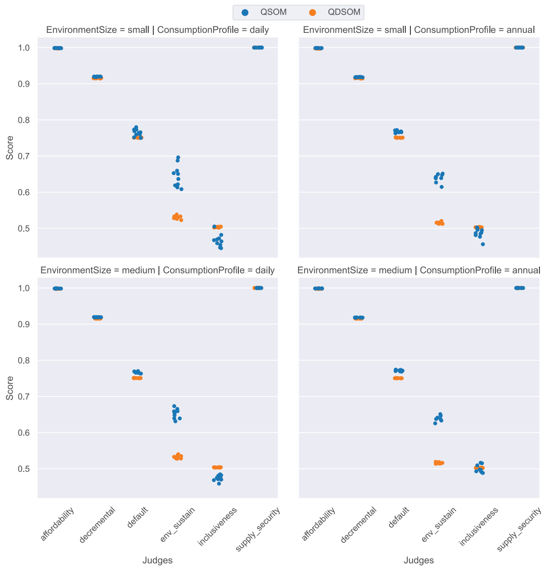
Fig. 5.6.: Results of the learning algorithms on 10 runs for each scenario, when using the LAJIMA agents.
