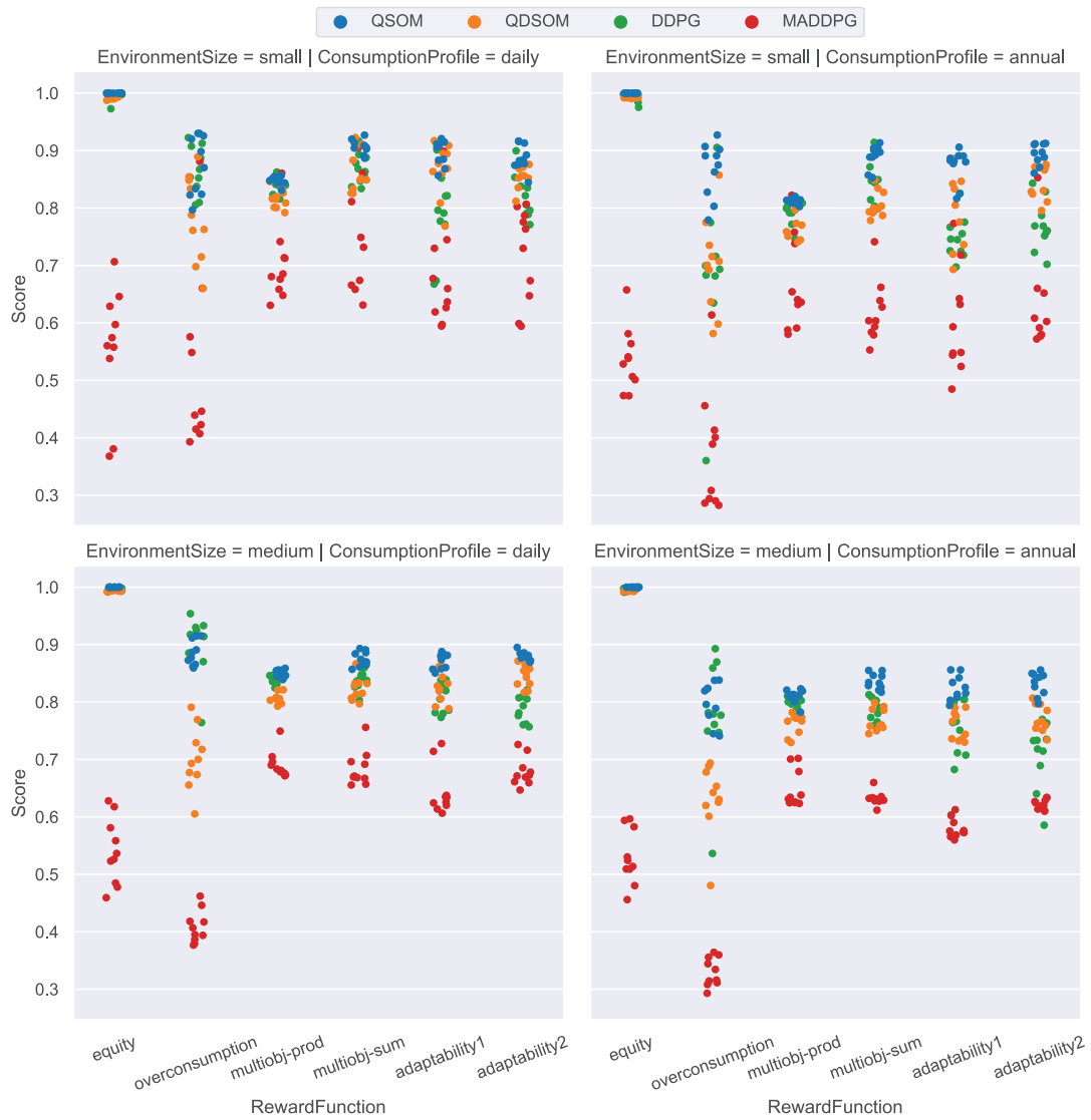
Fig. 4.5.: Distribution of scores per learning algorithm, on every scenario, for 10 runs with each reward function.
