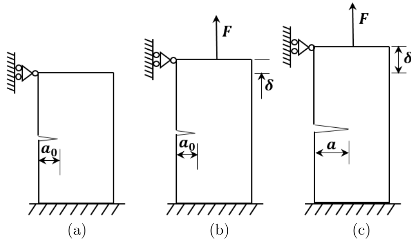
Figure 2.24: Case 1: plate subjected to a constant force, (a) original state, (b) loading state, (c) crack growth.
