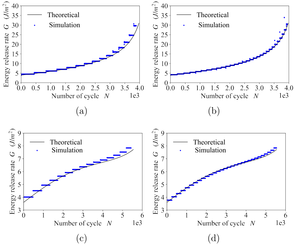
Figure 4.5: Simulations of a symmetric edge cracked plate with square packed samples and comparison with theoretical results of the energy release rate G under stress controlled fatigue loading for particle size (a) d = 2 \text{ mm} and (b) d = 1 \text{ mm} , and under strain controlled fatigue loading for particle size (c) d = 2 \text{ mm} and (d) d = 1 \text{ mm} .
