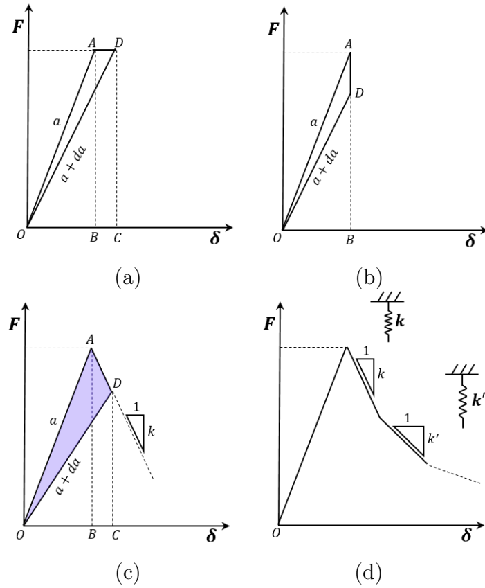
Figure 2.28: Released energy during crack extension: (a) constant force, (b) fixed displacement, (c) elastic constraint and (d) varying elastic constraint.
