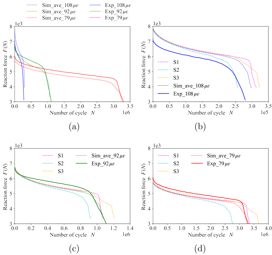
Figure H.1: T-C fatigue tests simulation results, (a) comparison of average simulation results and experimentation [1] with different test strain levels, and reaction force evolution of all three samples with strain levels respectively (b) 108 \mu\epsilon , (c) 92 \mu\epsilon and (d) 79 \mu\epsilon .
