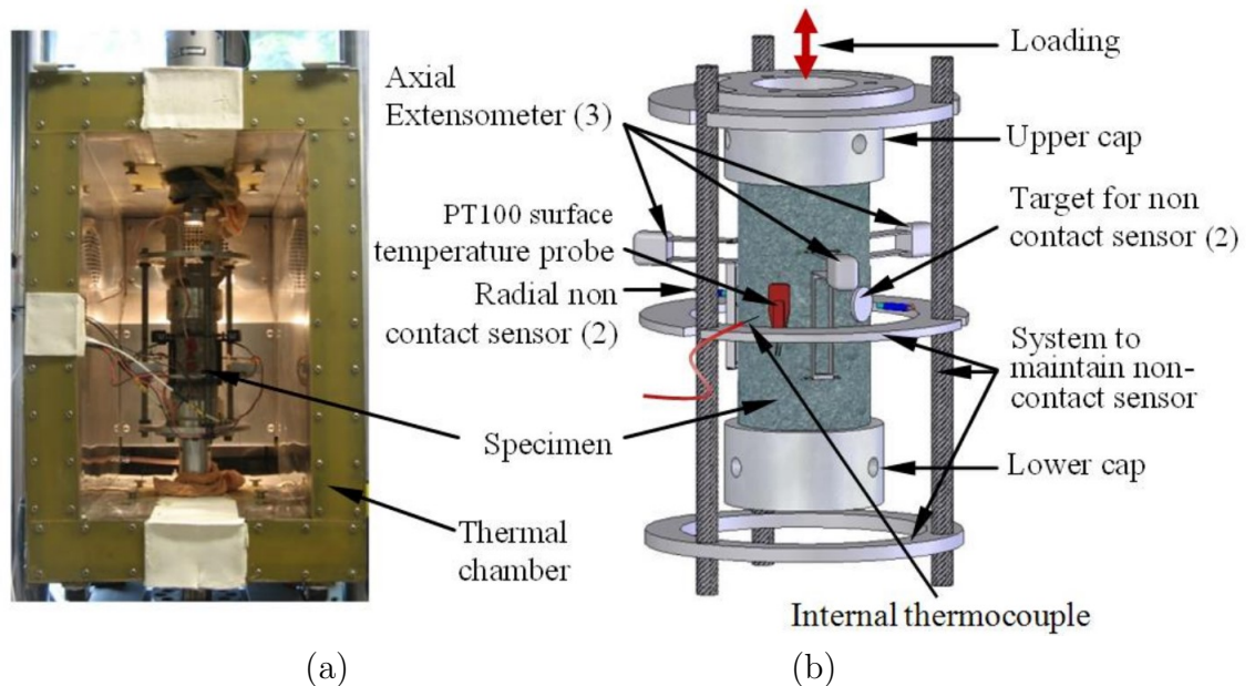
Figure 5.8: (a) Configuration of T-C test, and (b) details of test equipment. (Modified from [8])
