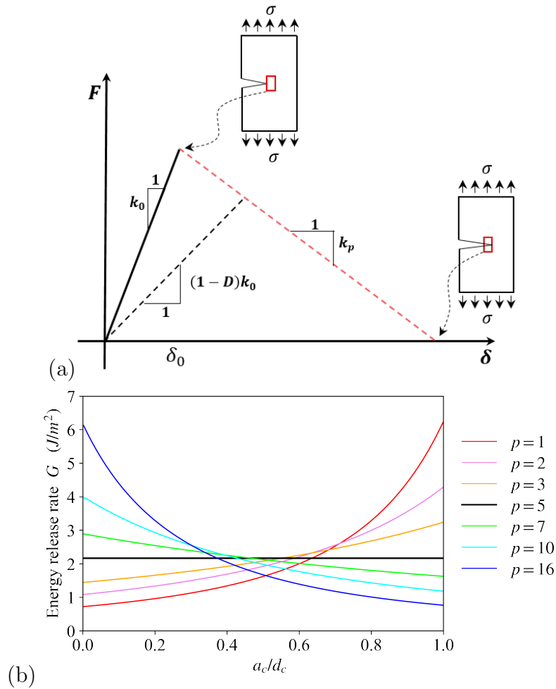
Figure 5.3: (a) Example of a contact in rupture with initial stiffness k_0 , when crack reaches its boundary, contact displacement is \delta_0 . During the rupture process, the measured slope ratio k_0/k_p = 5 . (b) Corresponding values of energy release rate G for different values of parameter p adopted in Equations 3.23 and 3.24.
