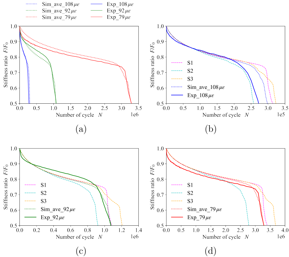
Figure 5.12: T-C fatigue tests simulation results, (a) comparison of average simulation results (three samples) and experimentation [1] with different test strain levels, and fatigue evolution of all three samples (S1, S2 and S3) with strain levels respectively (b) 108 \mu\epsilon , (c) 92 \mu\epsilon and (d) 79 \mu\epsilon .
