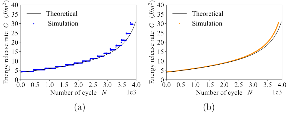
Figure 5.4: Simulations of a symmetric edge cracked plate with square packed samples and comparison with theoretical results of the energy release rate G under stress controlled fatigue loading for particle size d = 2 \text{ mm} (a) p is measured cycle by cycle, generally p \approx 2.85 and (b) p is imposed as a parameter, p = 2.6 .
