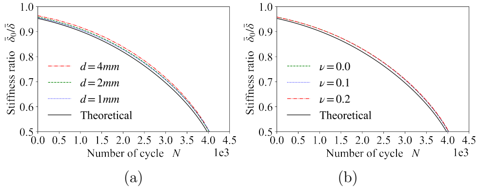
Figure 4.3: Simulations of a symmetric edge cracked plate under stress controlled fatigue loading with hexagonal packed samples and comparison with theoretical results of the stiffness ratio as a function of the number of loading cycles N for (a) different particle size (Poisson's ratio \nu = 0 ) and (b) different Poisson's ratios (and d = 2mm ) in controlled stress conditions.
