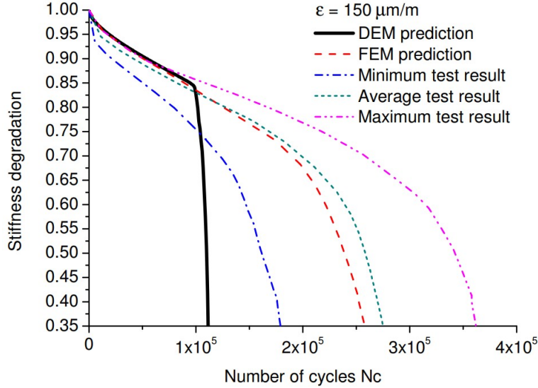
Figure 2.19: 4PB test simulation in DEM by Gao [101], experimental results and simulations in FEM by Arsenie [3, 102, 103].
