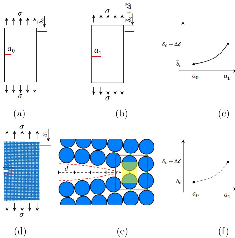
Figure 3.4: (a) Elastic plate with initial crack a_0 under stress \sigma , resulting displacement \bar{\delta}_0 (b) effect of a crack growth (from a_0 to a_1 ) over the displacements versus crack length, (c) evolution of the displacement. (d) DEM corresponding sample, (e) zoom of the propagated length (d), and (f) the corresponding evolution of the displacements versus crack length.
