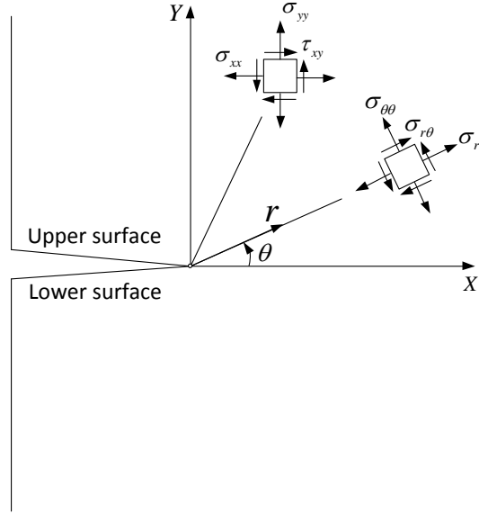
Figure 2.22: The rectangular and polar coordinate components of stress field around the crack tip (Modified from [107]).
