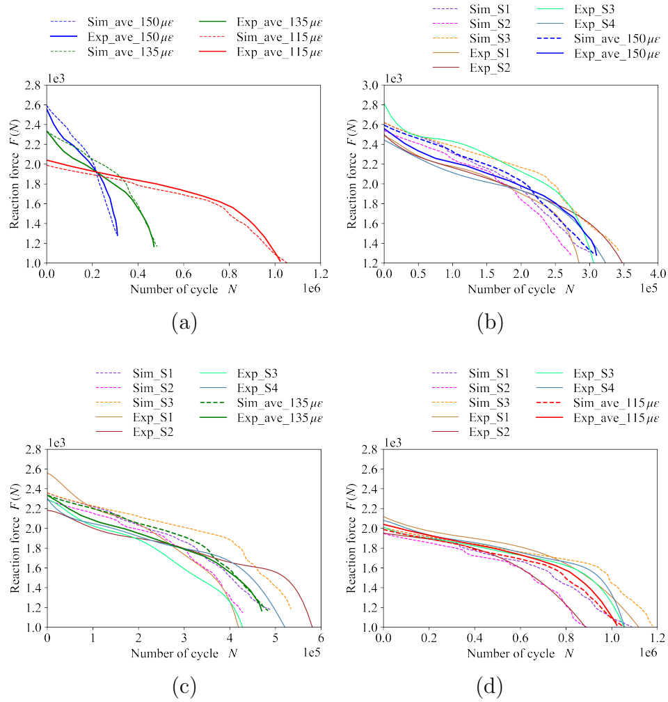
Figure H.2: Comparison of reaction force evolution between 4PB fatigue tests simulation and that of experimentation [150], (a) average curves for different test strain levels, (b) average and all curves for test strain level 150 \mu\epsilon , (c) 135 \mu\epsilon and (d) 115 \mu\epsilon .
