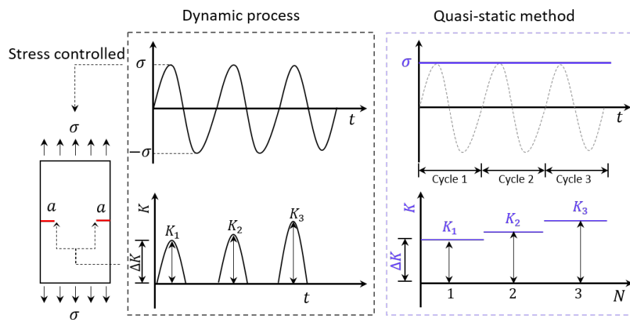
Figure 3.21: Quasi-static loading and extraction of the values of stress intensity range \Delta K at crack tips.
