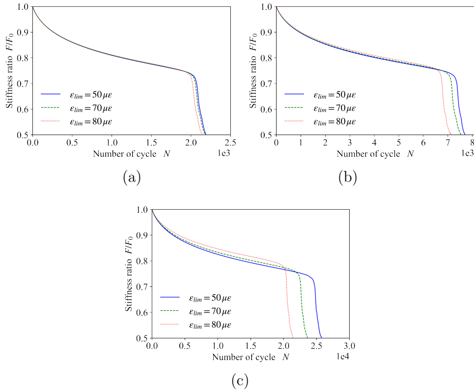
Figure 5.11: Comparison of results for different levels of contact endurance limit \varepsilon_{lim} , for test strain levels respectively (a) 108 \mu\varepsilon , (b) 92 \mu\varepsilon and (c) 79 \mu\varepsilon .
