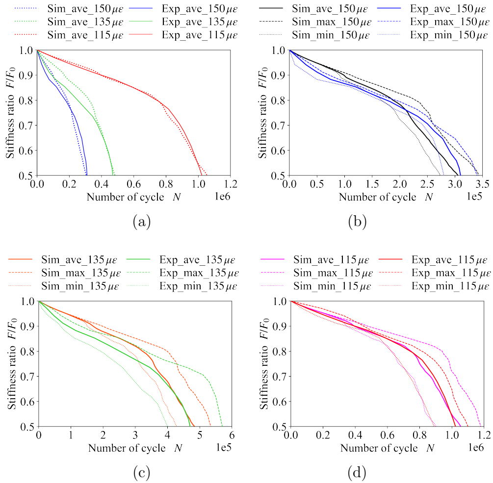
Figure 5.16: Comparison between 4PB fatigue test simulations and experiments [150], (a) average curves for different test strain levels, (b) average and envelop curves for test strain level 150 \mu\epsilon , (c) 135 \mu\epsilon and (d) 115 \mu\epsilon . For example, Sim_ave_115 \mu\epsilon is the average curve of simulation of all three samples at test strain level 115 \mu\epsilon , Sim_max_115 \mu\epsilon is the maximum boundary of the envelop of all simulations at test strain level 115 \mu\epsilon , and sign of min for the minimum boundary of the envelop of all simulations. So that for experimental results with sign Exp.
