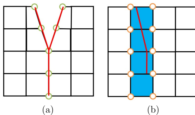
Figure 2.34: Schematic of crack propagation modeling: (a) nodes and crack in FEM with cohesive zone elements (a) and (b) enriched nodes and crack in XFEM, (Modified from [136]).
