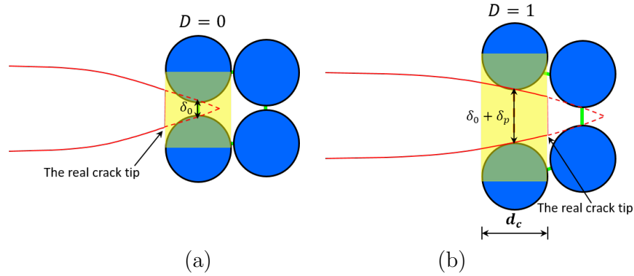
Figure 3.7: Schematic description of the position of crack and contact displacement. (a) Crack tip at the boundary of the contact domain, where \delta_0 is the contact displacement, and (b) crack totally through the contact domain.
