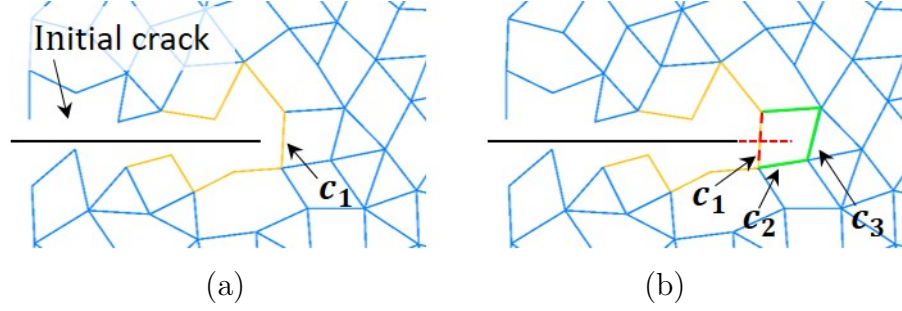
Figure F.2: (a) Initial crack tip identification, yellow contacts shows crack surface near crack tip, and (b) schematic for the effective width of contact domain d_c detection.
