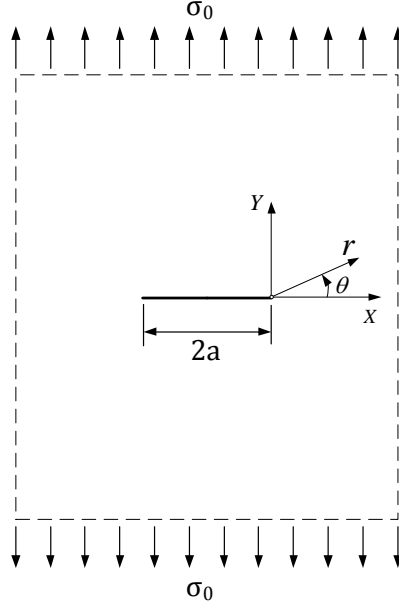
Figure 2.21: A center cracked infinite plate subjected to uniform remote tension [101].
