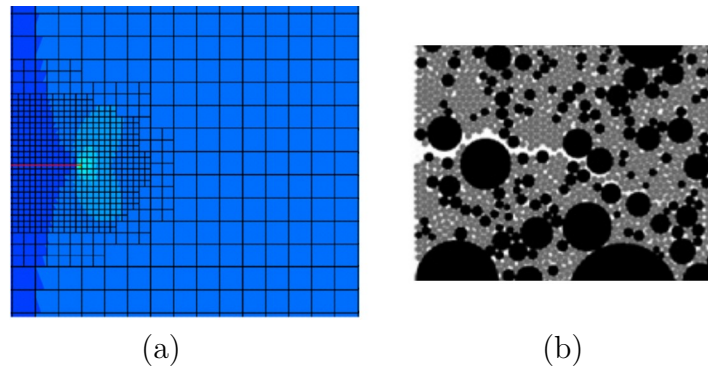
Figure 2.17: (a) Finite element mesh refinement for crack propagation, (Modified from [84]) and (b) discrete element particles detachment for crack propagation, (Modified from [78]).
