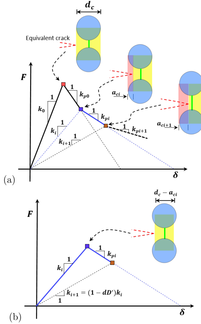
Figure 3.20: (a) Description of the contact and force-displacement evolution during a propagation event, (b) a certain state in (a).
