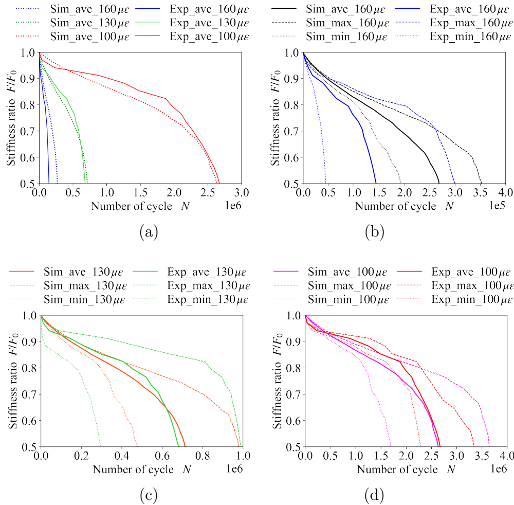
Figure 5.21: Comparison between 2PB fatigue tests simulation and experimentation [150], (a) average curves for different test strain levels, (b) average and envelop curves for test strain level 160 \mu\epsilon , (c) 130 \mu\epsilon and (d) 100 \mu\epsilon . For example, Sim_ave_160 \mu\epsilon is the average curve of simulation of all three samples at test strain level 160 \mu\epsilon , Sim_max_160 \mu\epsilon is the maximum boundary of the envelop of all simulations at test strain level 160 \mu\epsilon , and sign of min for the minimum boundary of the envelop of all simulations. So that for experimental results with sign Exp.
