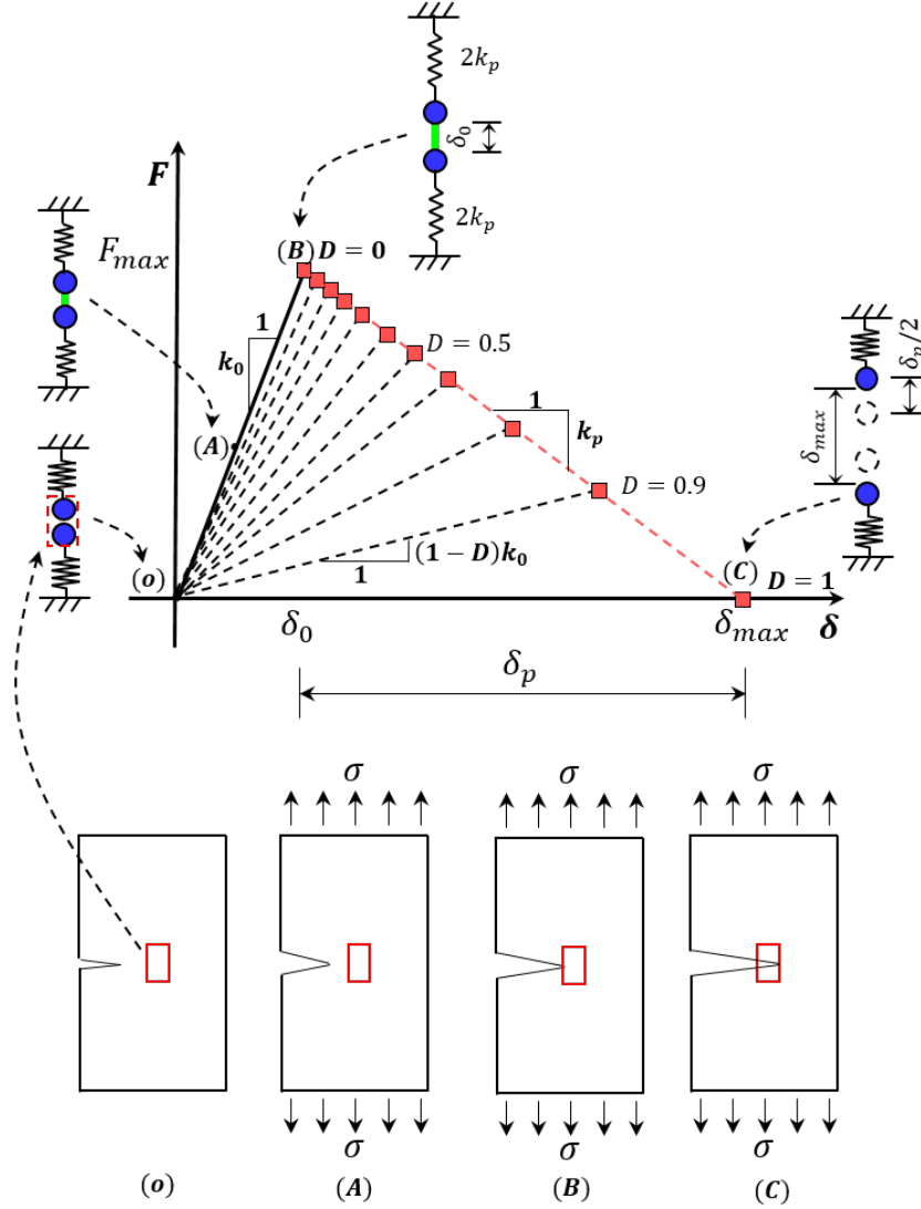
Figure 3.6: Description of the evolution of a contact for the whole process from crack near to crack through this contact. At the bottom of figure, (o) a pre-cracked plate in which a red rectangular represents the contact whose behavior is described by both spring systems and the evolution of contact force F and displacement \delta in the coordinate system, (A) plate subjected to a constant stress \sigma , (B) crack propagates till the boundary of the contact domain, (C) crack totally through the contact domain. From (B) to (C), crack growth within the contact domain is represented by the process of the contact stiffness degradation, for (0 \leq D \leq 1) , where k_0 is the initial contact stiffness, and (1 - D)k_0 is its degraded value.
