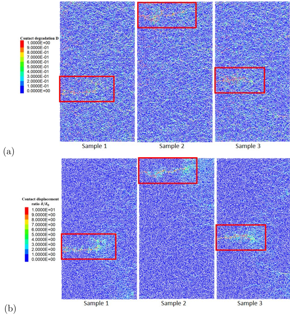
Figure 5.13: Crack distribution maps of all three samples, (a) contact degradation map (where red is totally broken and blue is intact), and (b) contact opening map representing by the ratio of the contact displacement \delta at stiffness ratio F/F_0 = 0.5 to the contact displacement at test beginning ( F/F_0 = 1 ) \delta_0 (where red means \delta/\delta_0 \geq 10 and blue means \delta/\delta_0 = 0 ), for simulation with strain level 108 \mu\epsilon .
