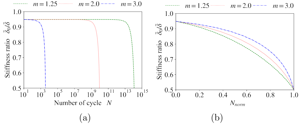
Figure 4.11: Fatigue evolution (a) versus number of cycles N and (b) versus number of cycles N_{norm} for different values of parameter m .
