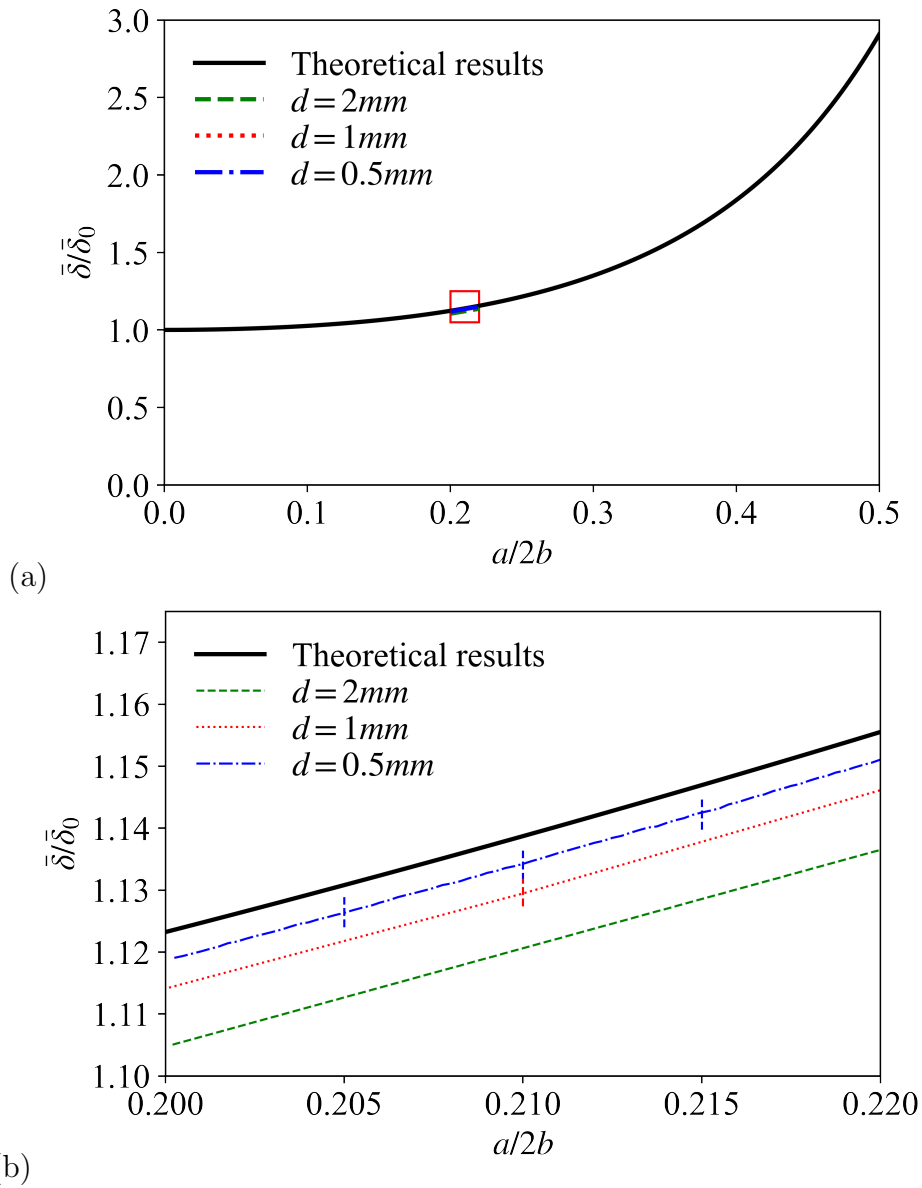
Figure 3.17: (a) Comparison of the ratio of displacement \bar{\delta}/\bar{\delta}_0 between theoretical results and simulation results and (b) a zoom for 0.2 \leq a/2b \leq 0.22 .
