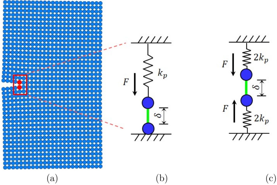
Figure 3.5: Schematic description of the mechanical relation between the contact at the crack tip and the neighboring particles. (a) Pre-cracked plate and (b) its simplified elastic behavior near the crack tip, where k_p represents the stiffness of material surrounding the crack tip, F and \delta are contact force and displacement, (c) a more intuitive description of (b).
