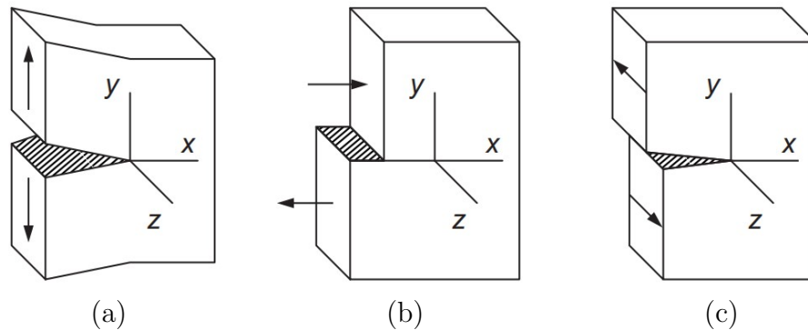
Figure 2.20: Schematic of the basic fracture modes: (a) Mode I (opening), (b) Mode II (sliding) and (c) Mode III (tearing) [104].
