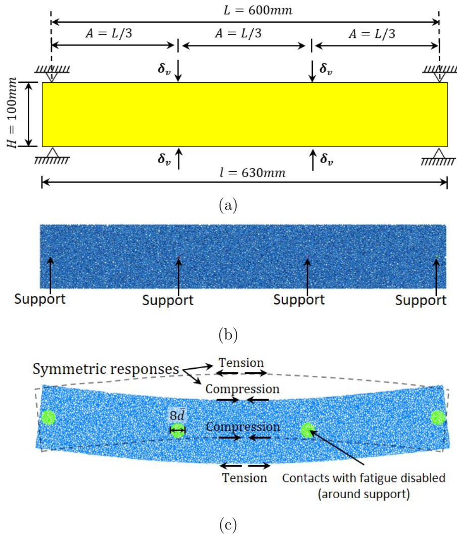
Figure 5.7: (a) Geometry of 4PB tests, (b) samples in DEM, and (c) simulation implementation.
