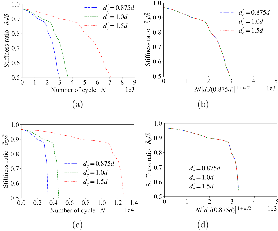
Figure 4.7: Stiffness ratio of a single edge cracked plate under stress fatigue for a random packed sample (a) as a function of the number of cycles N and (b) as a function of [d'_c/(0.875d)]^{1+m/2}N , for Paris's law parameters: C = 1.0 \times 10^{-12} (m/cycle/(Pa \sqrt{\text{m}} ) ^m ) and m = 1.25 , and that of (c) and (d) for C = 2.0 \times 10^{-22} (m/cycle/(Pa \sqrt{\text{m}} ) ^m ) and m = 3 .
