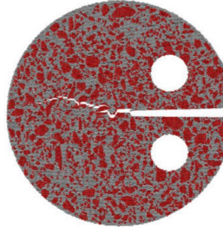
Figure 2.40: Crack trajectory resulting from CZM, (Modified from [140]).
