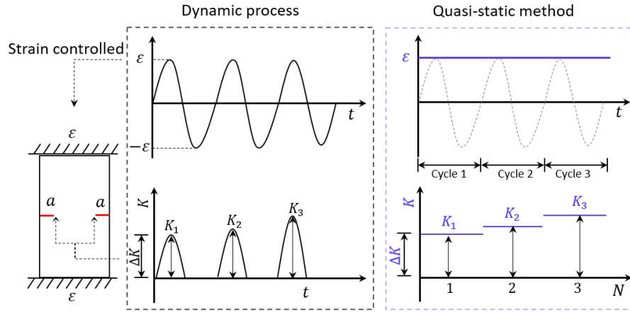
Figure D.2: Quasi-static process for strain controlled fatigue test.
