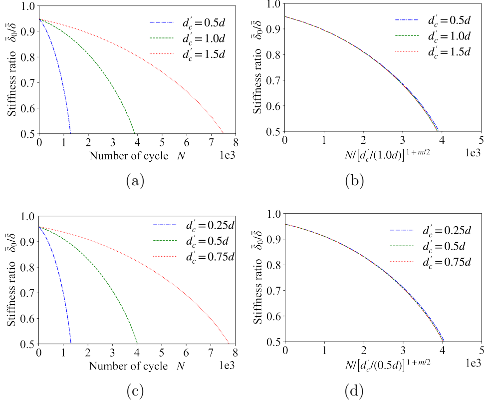
Figure 4.6: Stiffness ratio of a double edge cracked plate under stress fatigue: for a square packed sample (a) as a function of the number of cycles N and (b) as a function of [d'_c/(1.0d)]^{1+m/2}N ; for a hexagonal packed sample (c) as a function of the number of cycles N and (d) as a function of [d'_c/(0.5d)]^{1+m/2}N .
