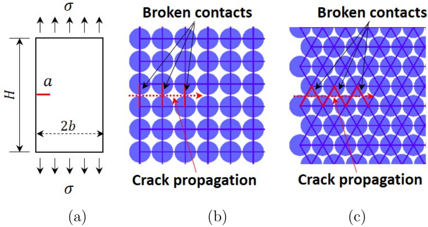
Figure 3.8: (a) Geometry of the plate, crack propagation modeling in (b) square and (c) hexagonal packed samples.
