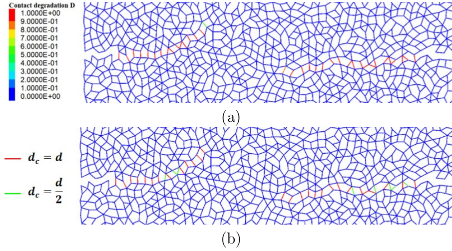
Figure F.3: (a) Crack path in contact degradation map, red to green corresponds to D = 1 to D = 0 , and (b) d_c of contacts on crack path, red contact means its d_c = d_{min} and green means d_c = \frac{1}{2}d_{min} .
