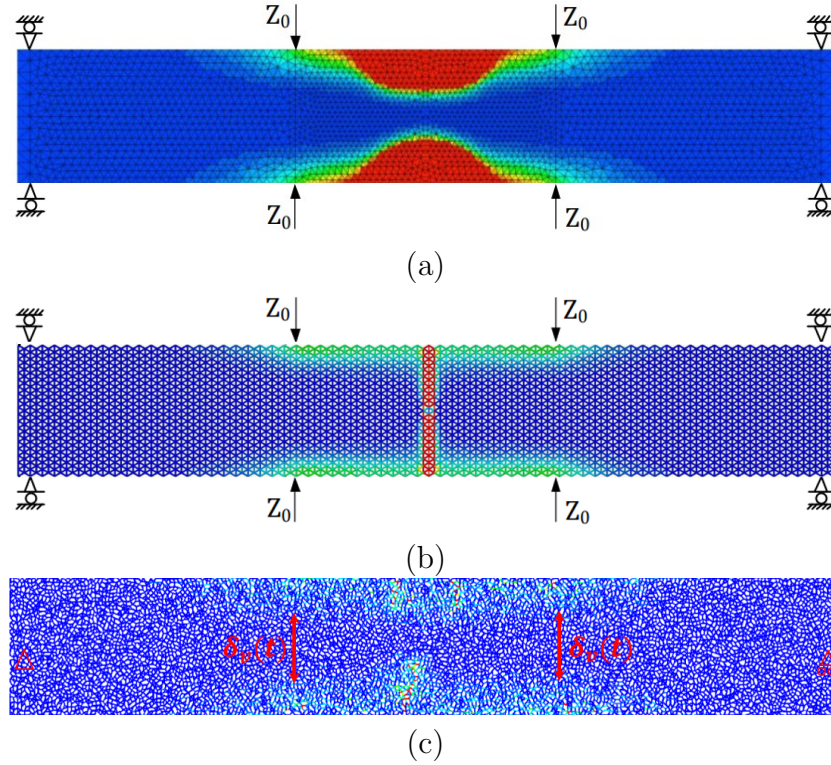
Figure 2.14: Damage maps (blue to red means D = 0 to D = 1 ) displaying different localization levels of 4-point bending fatigue test simulations by using damage model: (a) finite element method conducted by Arsenie [3], (Modified from [101]), (b) regular packing discrete element method conducted by Gao [101], (Modified from [101]), (c) randomly packing discrete element method conducted by Liu [4], (Modified from [4]).
