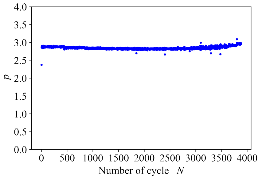
Figure E.14: The contact separation ratio p evolution from simulation results with balance level 1.0 \times 10^{-6} .
