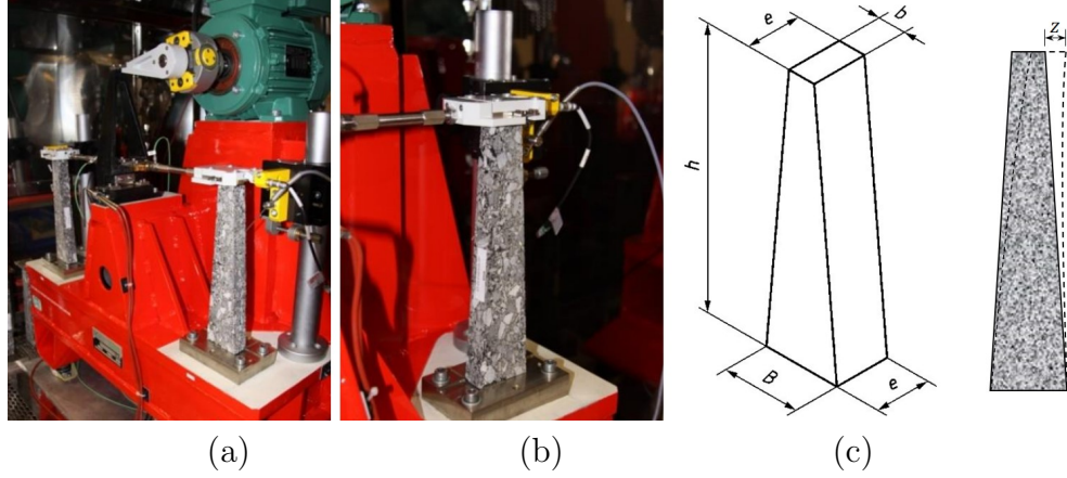
Figure 5.19: (a) Configuration of 2PB fatigue test, (b) details of test sample, and (c) sample dimension and test scheme. (Modified from [8, 151])
