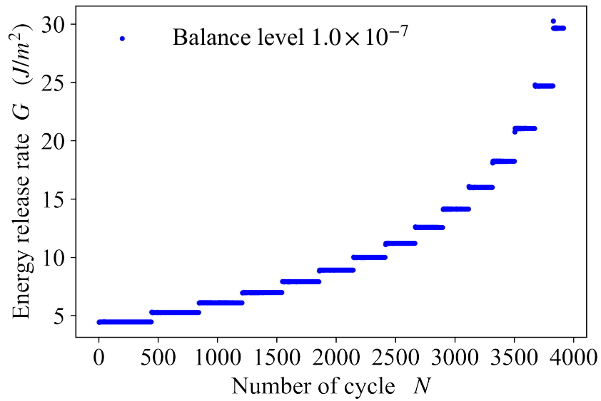
Figure E.15: Energy release rate from simulation results with balance level 1.0 \times 10^{-7} .
