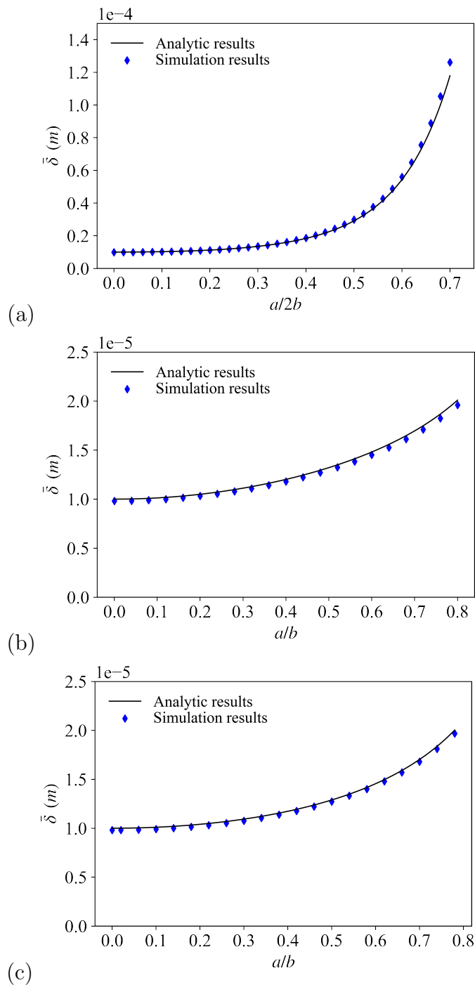
Figure C.3: Comparison of the average relative displacement \bar{\delta} between analytic results and simulation results, for (a) plate with edge crack, (b) plate with symmetric edge cracks, (c) plate with center crack.
