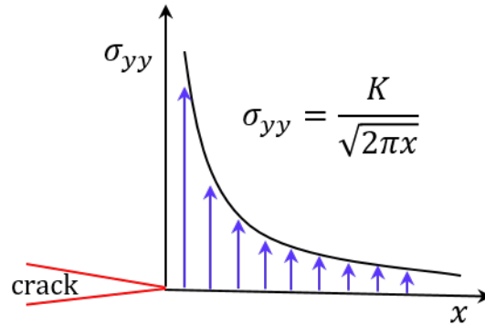
Figure 2.23: Scheme of the stress distribution near a crack tip as a function of the stress intensity factor K [105].
