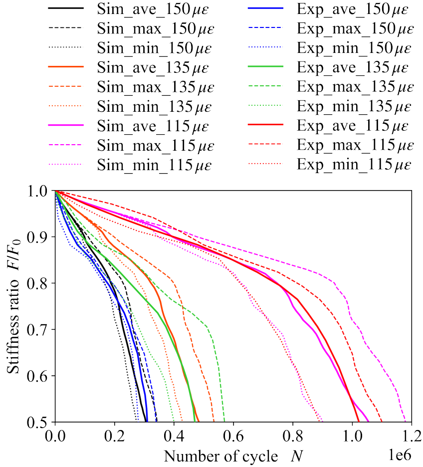
Figure 5.15: Comparison between envelop curves and average curves of 4PB fatigue test simulations and that of experiments [150], for different test strain levels. For example, Sim_ave_115 \mu\varepsilon is the average curve of simulation of all three samples at test stain level 115 \mu\varepsilon , Sim_max_115 \mu\varepsilon is the maximum boundary of the envelop of all simulations at test stain level 115 \mu\varepsilon , and sign of min for the minimum boundary of the envelop of all simulations. So that for experimental results with sign Exp.
