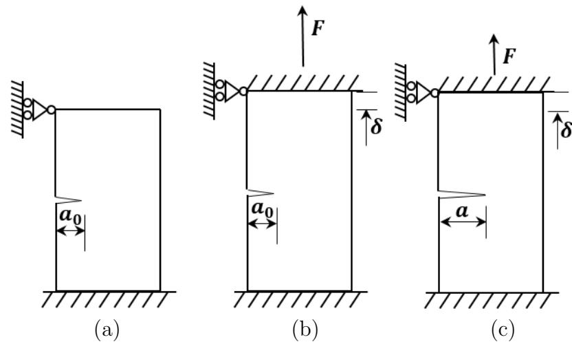
Figure 2.25: Case 2: after tension, plate displacement \delta is fixed, (a) original state, (b) loading state, (c) crack growth.
