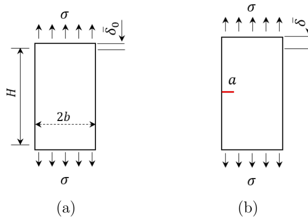
Figure 3.16: Plate under uniform stress and the associated boundary displacement for (a) intact and (b) cracked cases.
