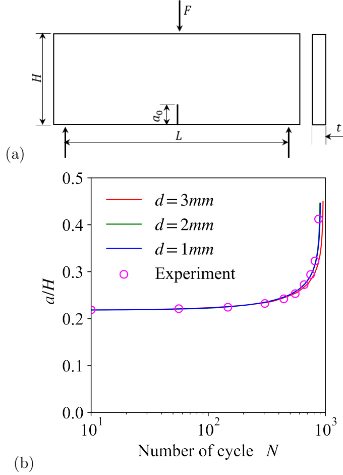
Figure 4.12: (a) Geometry of the three-point bending beam. (b) Evolution of the crack length ratio a/H as a function of the number of cycle N . Comparison between test results and DEM simulation.
