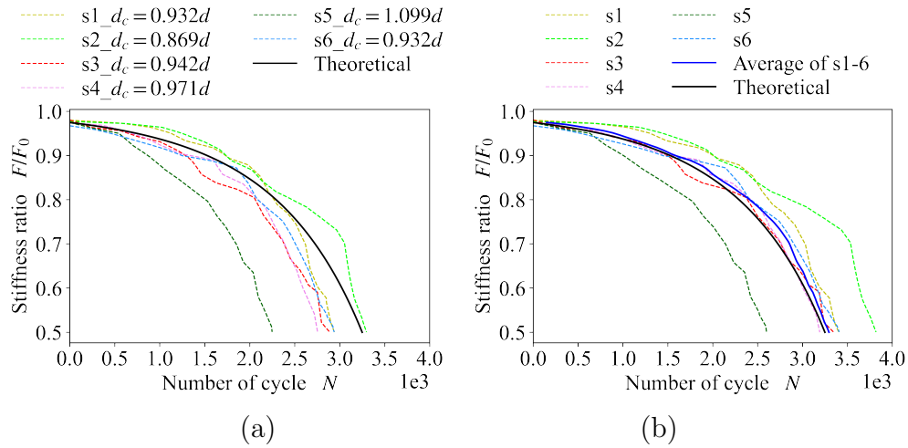
Figure 4.8: (a) Stiffness ratio of a double edge cracked plate under stress fatigue for random packed sample s1 to s6, as a function of the number of cycles N . And each calibrated value of d_c , based on Equation 4.3 and theoretical results for Paris's law parameters: C = 1.0 \times 10^{-12} (\text{m/cycle}/(\text{Pa}\sqrt{\text{m}})^m) and m = 1.25 . (b) Comparison of simulations with d_c = 0.958d and the theoretical results.
