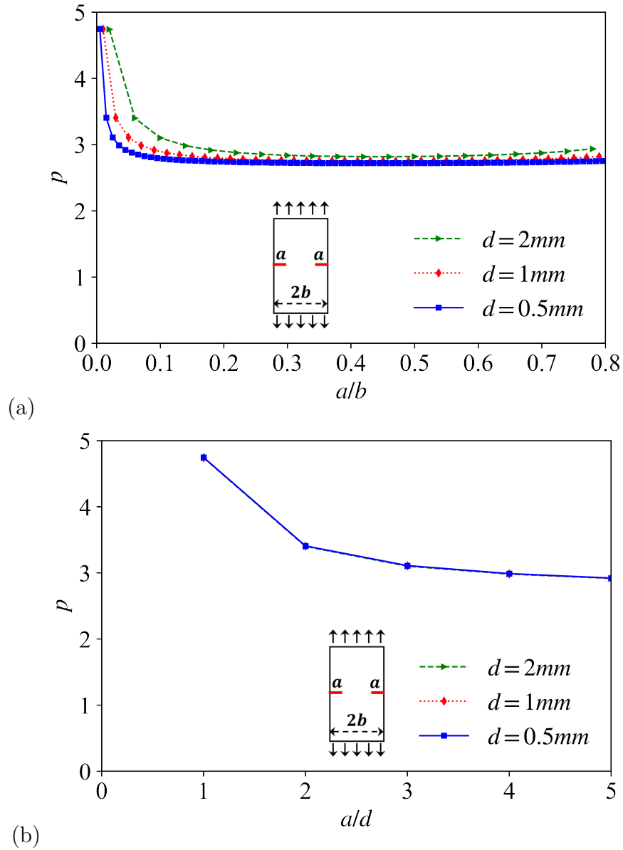
Figure 3.9: (a) Value of the slope ratio p as a function of the length to plate width ratio a/b for different particle diameters ( 0.5\text{ mm} \leq d \leq 2\text{ mm} ) of a plate with symmetric edge cracks, simulated by square packed samples and (b) a zoom of the values of p as a function of the crack to diameter ratio a/d during crack initiation a/d \leq 5 .
