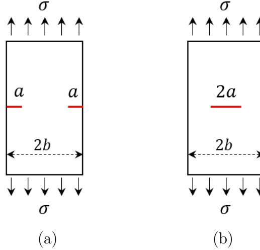
Figure C.2: (a) Finite plate with symmetric edge cracks, (b) finite plate with center crack.
