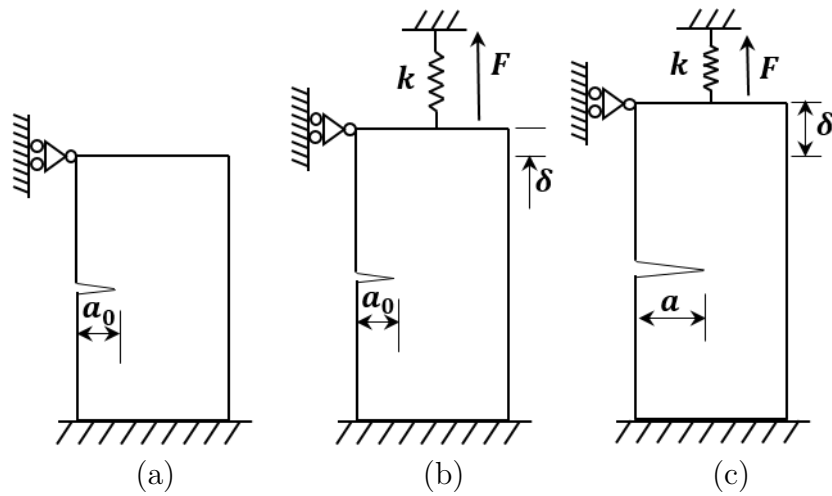
Figure 2.26: Case 3: after tension, plate top is restrained by elastic constraint with stiffness k , (a) original state, (b) loading state, (c) crack growth.
