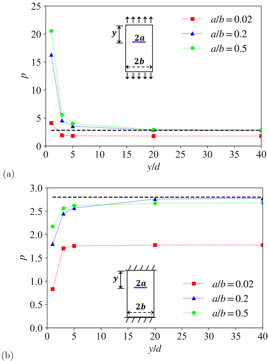
Figure 3.12: Value of the slope ratio p for crack at different vertical positions ( y/d , where y is the distance from loading boundary and d = 2 \text{ mm} is particle diameter) and with different crack length ( a/b ), (a) with imposed stress and (b) with imposed strain ( \varepsilon = 100 \mu\varepsilon ). The black dashed line represents p = 2.8 in both (a) and (b).
