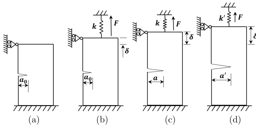
Figure 2.27: Case 4: after tension, plate top is restrained by elastic constraint with varying stiffness k and position, (a) original state, (b) loading state, (c) crack growth, (d) after elastic constraint stiffness and position change, crack continually grows.
