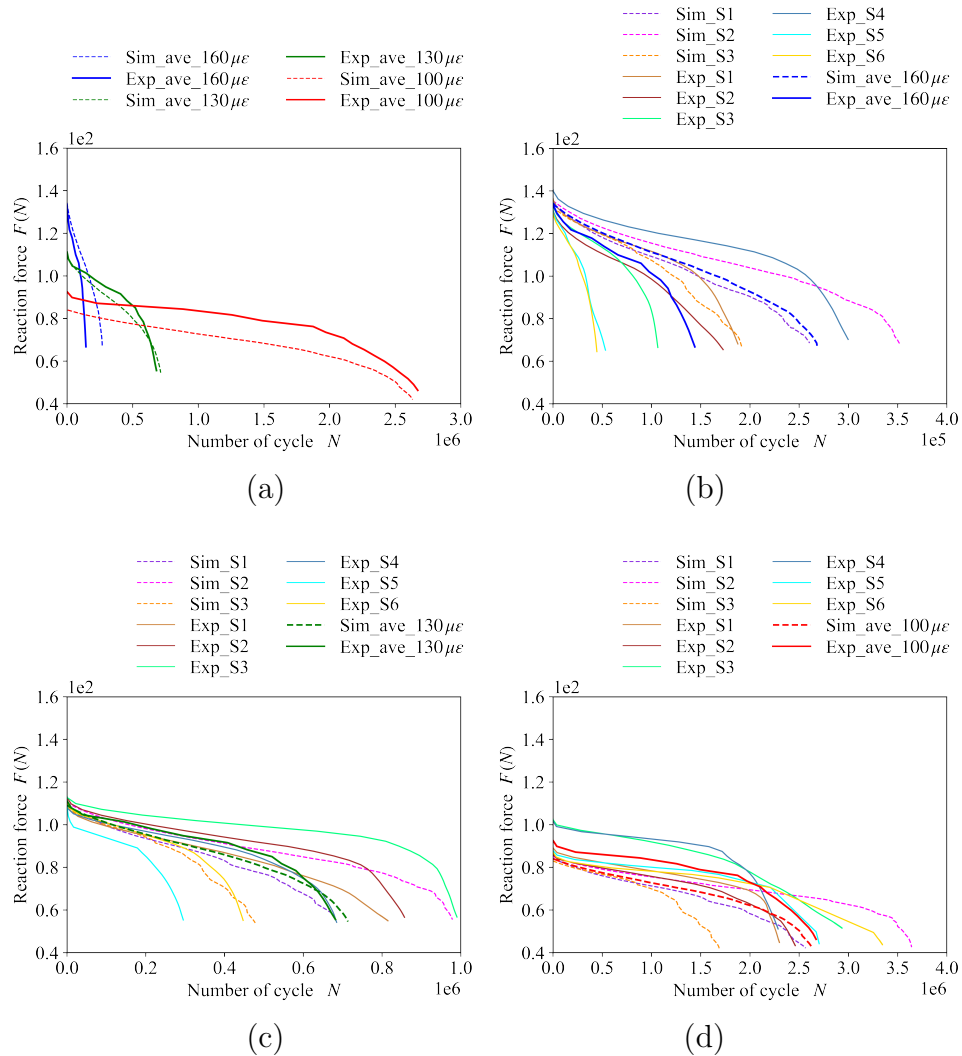
Figure H.3: Comparison of reaction force evolution between 2PB fatigue simulation and experimentation [150], (a) average curves for different test strain levels, (b) average and all curves for test strain level 160\mu\epsilon , (c) 130\mu\epsilon and (d) 100\mu\epsilon .
