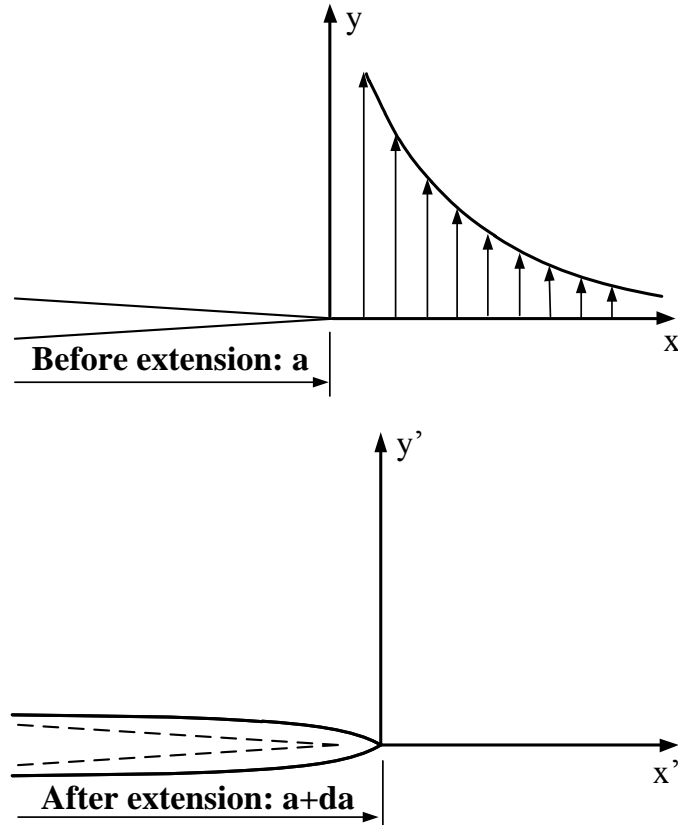
Figure 2.29: Stress distribution before extension and surface opening after extension [101].
