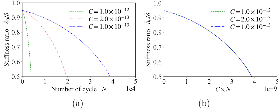
Figure 4.10: Fatigue evolution (a) versus number of cycles N and (b) versus C \times N for different values of parameter C .
