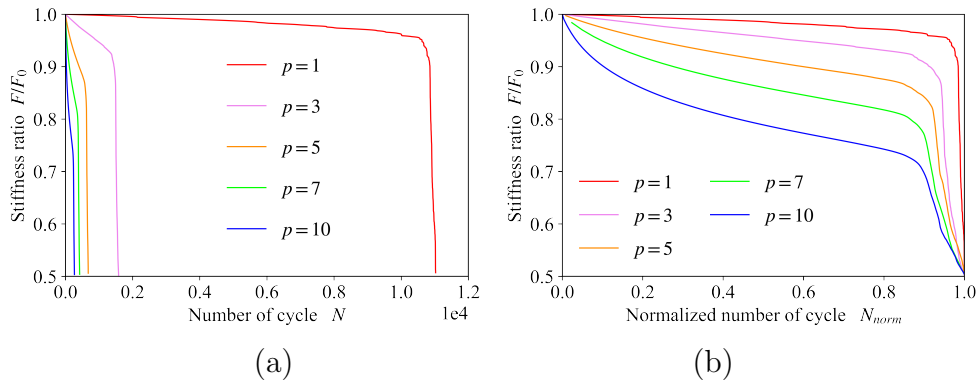
Figure 5.9: (a) Fatigue evolution expressed by the stiffness ratio (represented as the ratio of the reaction force to the initial reaction force, F/F_0 ) as a function of the number of cycle N for different values of parameter p , and (b) stiffness ratio versus the normalized number of cycle.
