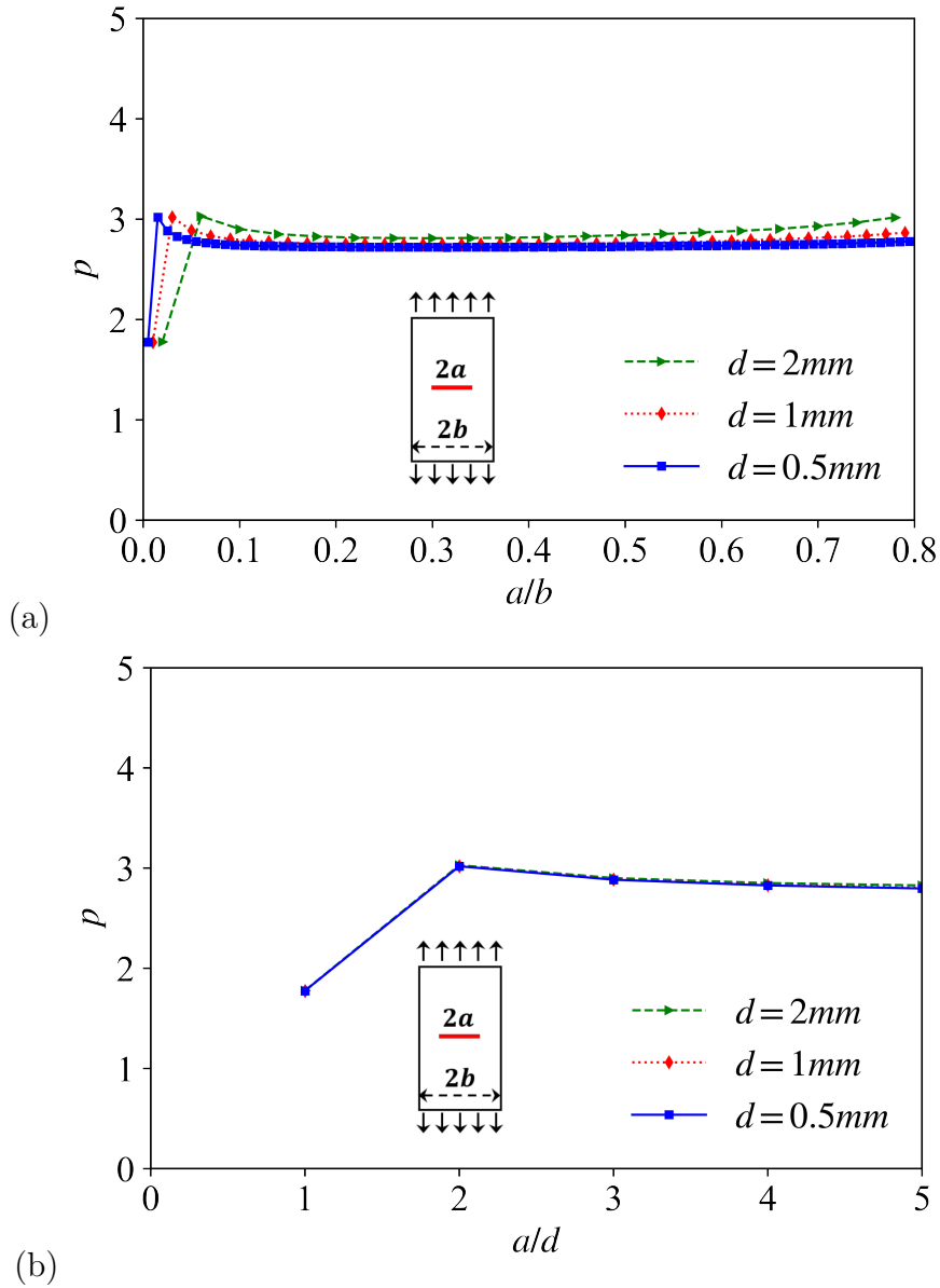
Figure 3.10: (a) Value of the slope ratio p as a function of the crack length to plate width ratio a/b for different particle diameters ( 0.5\text{ mm} \leq d \leq 2\text{ mm} ) of a plate with center crack, simulated by square packed samples and (b) a zoom of the values of p as a function of the crack to diameter ratio a/d during crack initiation a/d \leq 5 .
