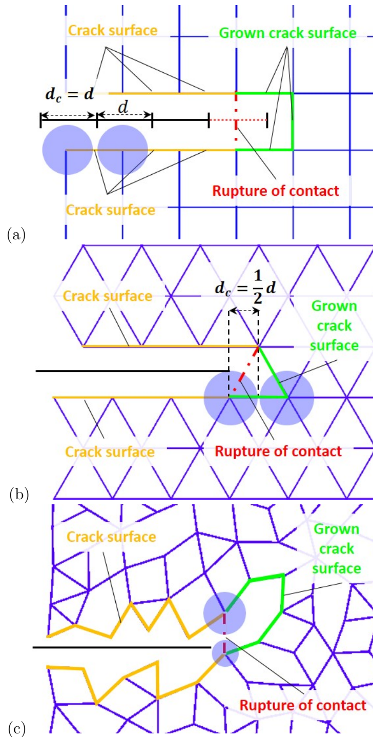
Figure 4.1: Definition of a crack for (a) square, (b) hexagonal and (c) randomly packed samples. Identification of the crack domain d_c for square and hexagonal packed samples.
