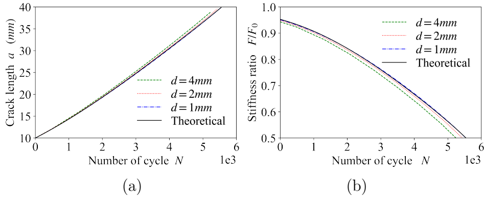
Figure 4.4: Simulations of a symmetric edge cracked plate under strain fatigue loading with square packed samples for different particle sizes and comparison with theoretical results of (a) crack growth and (b) the stiffness ratio as functions of the number of cycles N in controlled strain conditions.
