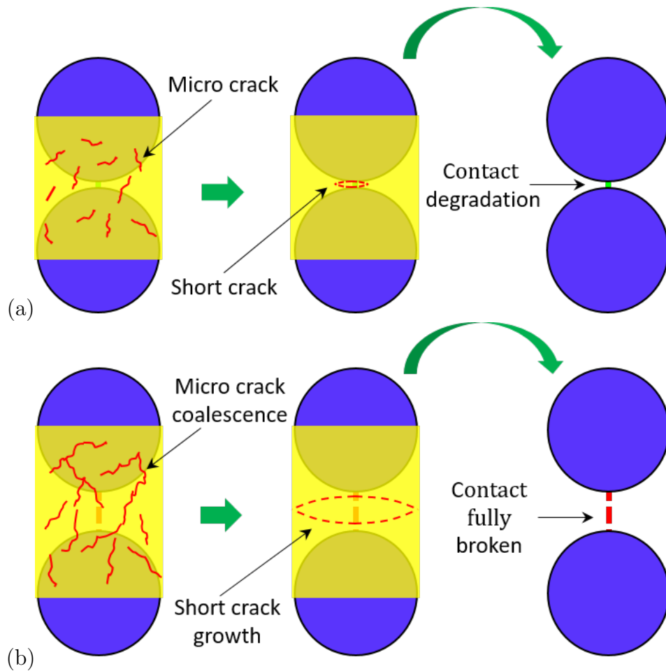
Figure 5.5: Scheme of the equivalent propagated length for an initially microcracked contact: (a) initial state of material, and (b) progressive coalescence of cracks.
