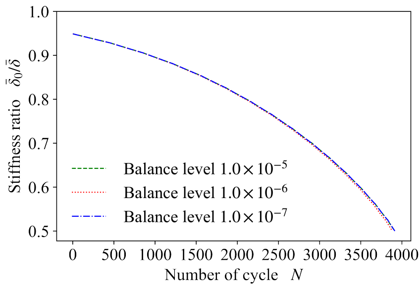
Figure E.17: Fatigue evolution from simulation results with different balance level.
