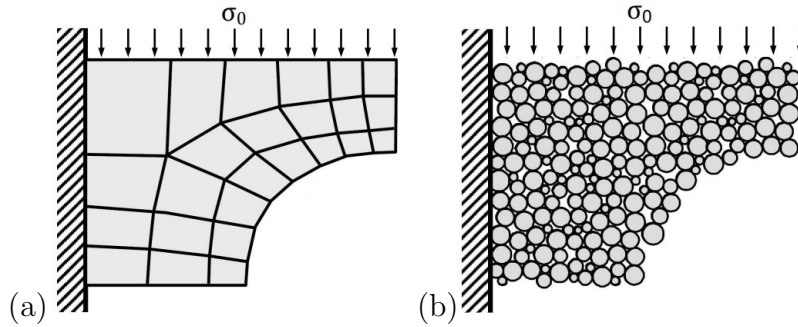
Figure 2.16: (a) Finite element mesh and (b) discrete element mesh, (Modified from [83]).
