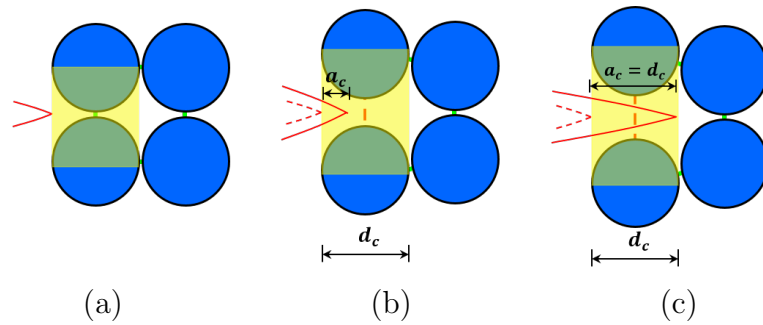
Figure 3.3: (a) Crack tip at vicinity of a contact and with crack propagation from (a) to (b) then to (c), its trajectory during the rupture of the contact described by the variable a_c ( 0 \leq a_c \leq d_c ).
