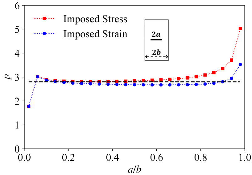
Figure 3.13: Comparison of the slope ratio p as a function of the crack length to plate width ratio a/b , for center crack, (a) with imposed stress and (b) with imposed strain ( \varepsilon = 100 \mu\varepsilon ). The black dashed line represents p = 2.8 .
