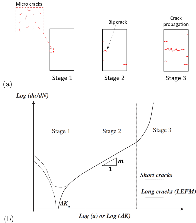
Figure 5.1: (a) Scheme of the three fatigue stages and (b) its effect on the propagation of cracks per cycle da/dN as a function of crack length a or stress intensity range \Delta K , solid line for long crack (except a is too small or too large, crack propagation complies with Paris' law), and dotted lines indicate two possibilities of the unknown law for short crack (modified from [114]).
