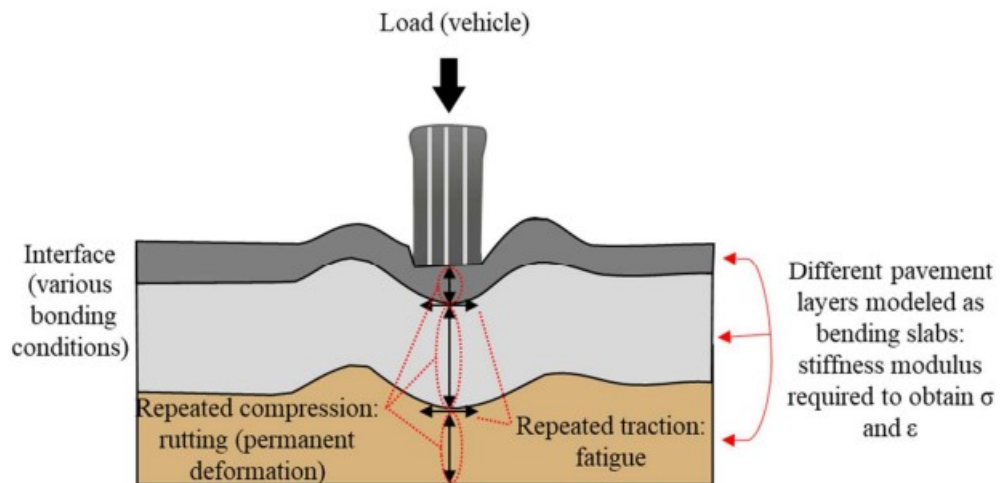
Figure 2.2: Schemes of vehicle loading and pavement layer response [1].
