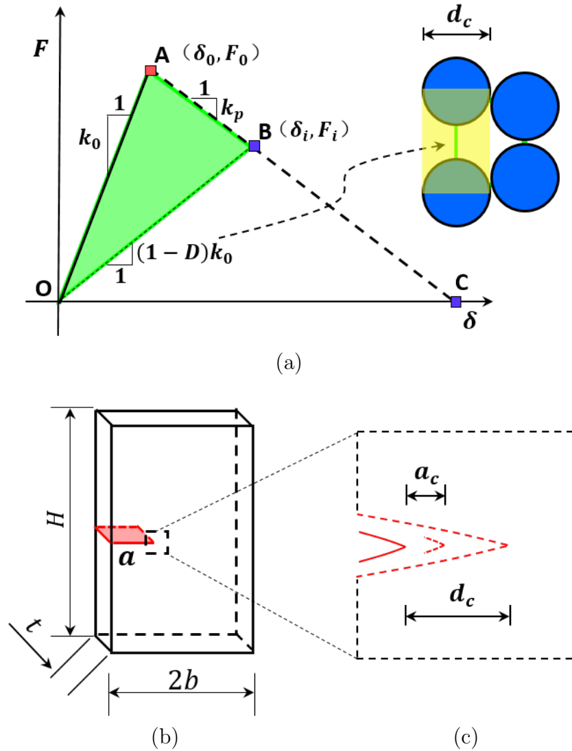
Figure 3.15: (a) Released energy during contact degradation. (b) Cracked plate, and (c) zoom of the crack propagation at the scale of one contact.
