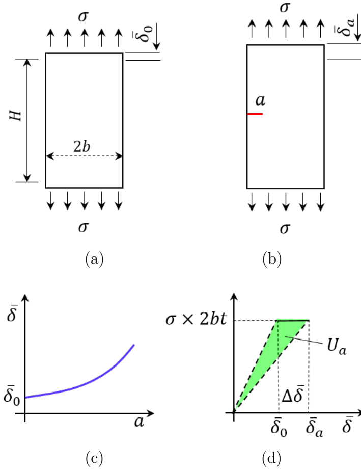
Figure C.1: (a) Plate deformation without crack, (b) plate deformation with crack, (c) the average relative displacement at plate ends versus crack length in the plate, (d) the external force versus the average relative displacement, describing the released energy during plate cracking.
