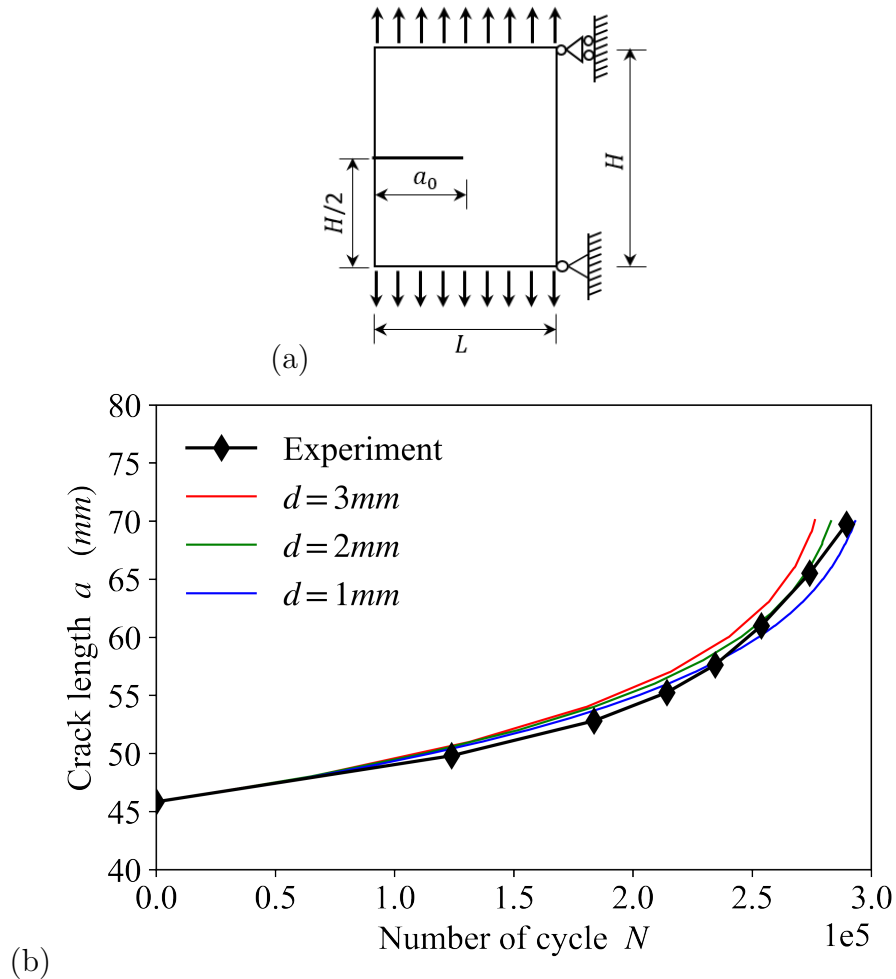
Figure 4.13: (a) Geometry of the single edge notch tension fatigue test. (b) Evolution of the crack length a as a function of the number of cycle N . Comparison between test results and DEM simulation.
