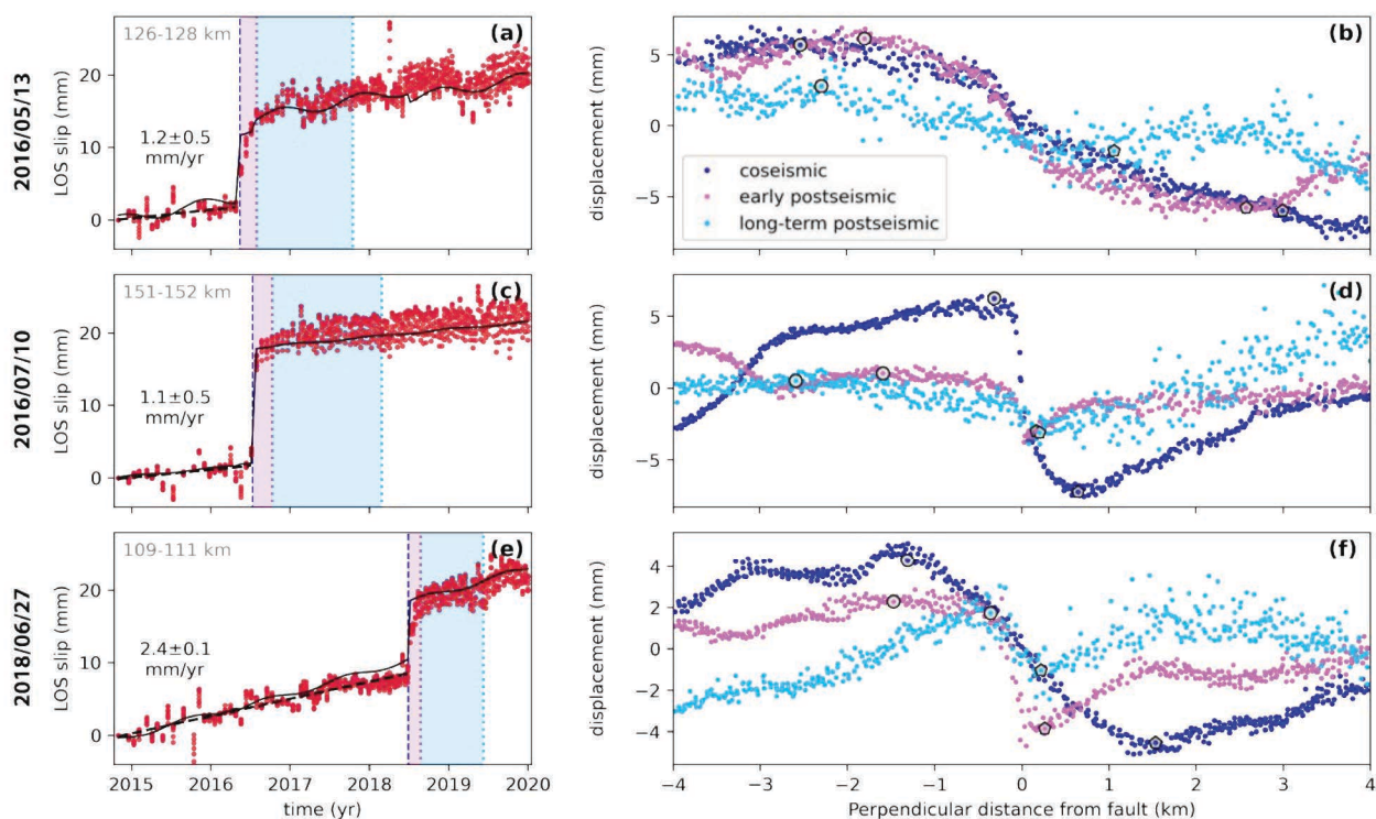
Figure 3.9: Temporal and spatial footprint of coseismic and postseismic deformation according to track 42 for earthquakes on the Chaman fault. Left : time series of differential displacement across the fault in LOS at the earthquake location on a 1-2 km long fault segment. The distance in the upper left corner refers to the distance along the fault to Nushki (Figure 3.4). Displayed velocities refer to the best-fitting slip rate before the earthquake. The differential parametrised model from KFTS on each side of the fault is the black line. The dark blue vertical dashed line indicates the timing of the earthquake and shaded regions corresponds to the periods over which the displacement in the plots on the right are measured. Right : Profiles of displacement in LOS reflecting the spatial distribution of slip during the coseismic phase as well as during the immediate and longer postseismic phases. Coseismic deformation is taken as the displacement recorded between the two SAR acquisitions framing the earthquake occurrence (dark blue). The local extrema used to compute peak-to-peak displacement are marked by white symbols outlined in black (pentagones for minima, circles for maxima). Profiles cover contiguous but mutually exclusive periods.
