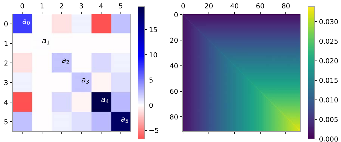
Figure A.2: Graphical representation of the final Covariance matrix (P_{91}) in the reference synthetic test (Section 2.3.1) for the same selected pixel than in Figure 2.3 and 2.5. Elements characterizing the variance-covariance of model parameters, a_n , (left) are represented separately from the variance-covariance of phase estimates, \phi_k , (right). A striking feature on the left subplot, is how well the velocity a_1 is constrained with this optimally parametrized inversion. For other parameters, inter-dependency is strong, especially with the initial offset a_0 . This is why we recommend to store out of the state vector parameters that have already converged (i.e. those for which new data is not informative). Notice the very small uncertainty and significant temporal correlation of phase estimates.
