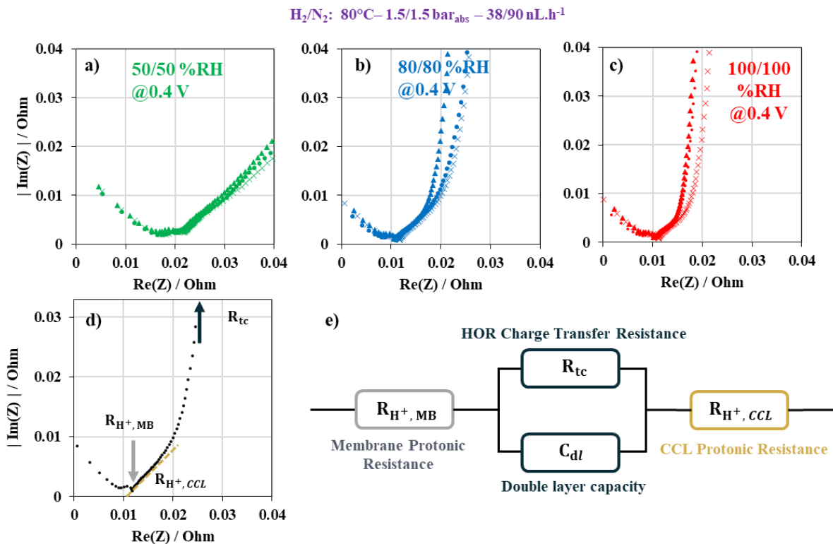
Figure III-20: Reproducibility of initial impedance spectra at 0.4 V in differential cell for three fresh MEA samples under H_2/N_2 at 50, 80 and 100% RH (a, b and c respectively) with (d) qualitative representation of resistances according to (e) equivalent electrical circuit under H_2/N_2 condition
