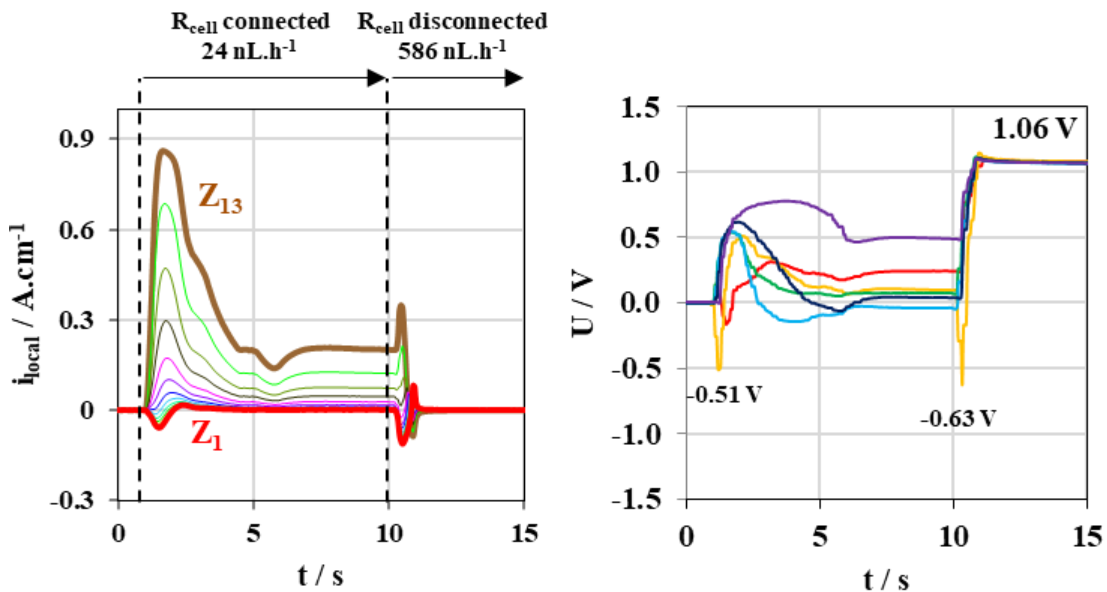
Figure V-12: Local current density profiles along the cathode channel and individual cell voltage profiles during the start-up phase and the following 15 s at the BoT of the test with R_{cell} configuration
