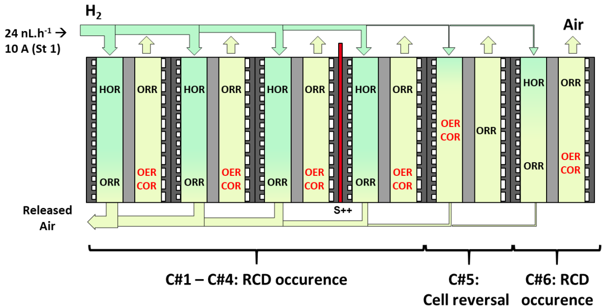
Figure V-10: Schematic representation of the short-stack in terms of individual gas supply and local possible reactions according to cell voltages and CDDM data during the SU phase (at t = 1.15 \text{ s} ) in open-circuit configuration
