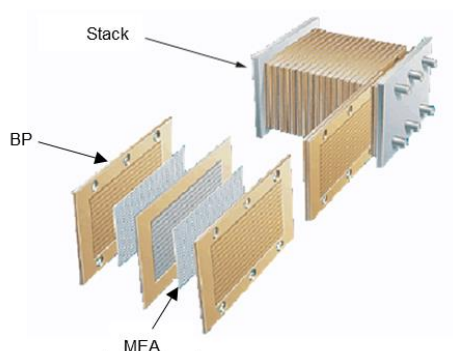
Figure I-6: PEMFC stack assembly [5]
