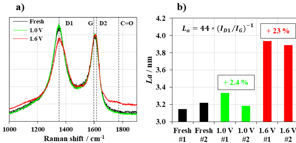
Figure IV-19: a) Normalized Raman spectra and b) deduced average crystallite size for fresh and aged MEA at 1.6 V and 1.0 V
