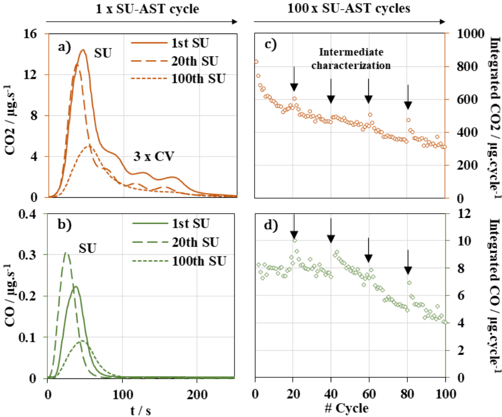
Figure IV-3: Detailed CO_2 (a) and CO (b) emission profiles during the 100 cycles in reference SU-AST; Integrated (c) CO_2 and (d) CO gas emission per cycle along reference SU-AST. Single cell operating conditions: H_2/N_2 - 60^\circ C - 80/80\% RH - 1.0/1.0 bar_{abs} (out) -300/800 nL.h^{-1}
