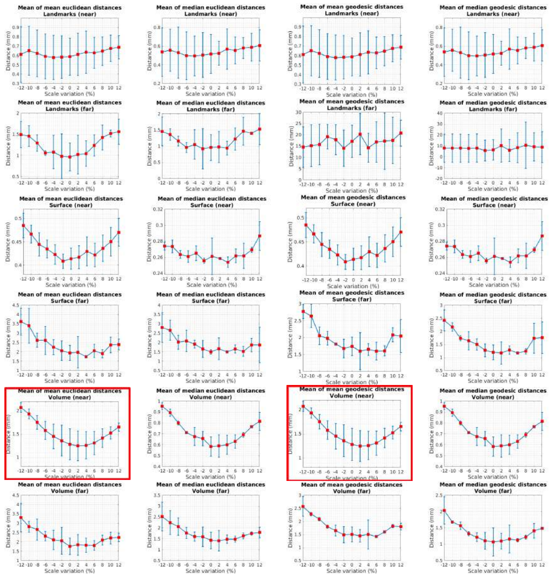
Figure 5.4: Behaviours of the 24 anisotropy measures for 2 phantoms, using 10 combinations of 8 views per phantom. Two anisotropy measures have a convex behaviour: They are highlighted in red and correspond to the near volume mean euclidean anisotropy, and the near volume mean geodesic anisotropy.
