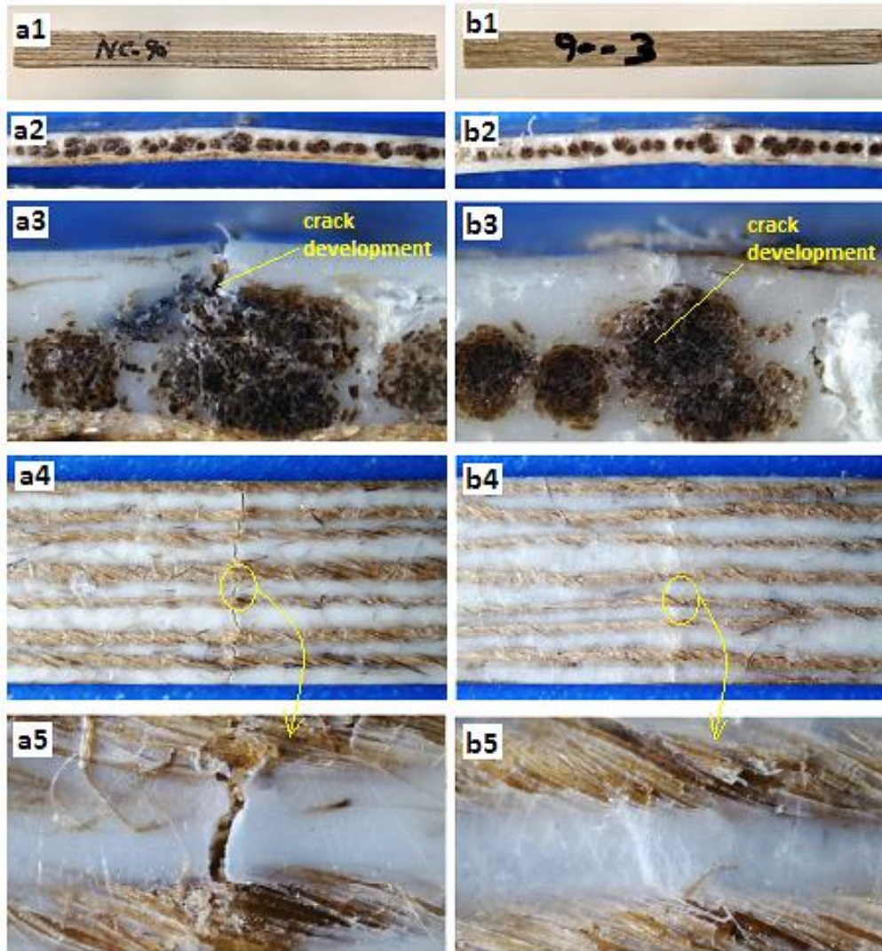
Figure 3-8. Tested samples of non-broken 3-point bending, (a1, b1) non-commingled and commingled specimens before test, (a2, b2) side view of tested specimens, (a3, b3) side zoomed in view of tested specimens with crack propagation, (a4, b4) tension sides of the specimens (a5, b5) tension side with zoomed view
