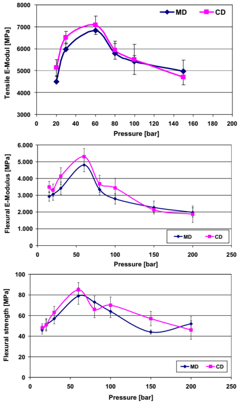
Figure 1-26. Mechanical properties of kenaf fibers vs. processing pressure, (a) tensile modulus, (b) flexural modulus, (c) flexural strength. The maximum values are at about 60bars. MD and CD are machine and cross directions. [112]
