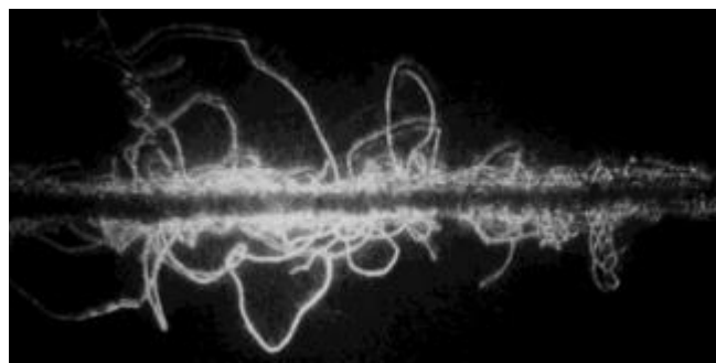
Figure 2-7. Method for measuring hairiness 'H' by the Uster-hairiness tester as a measure of amount of light transmitted by the protruding fibers and detected by a light sensor[141]
