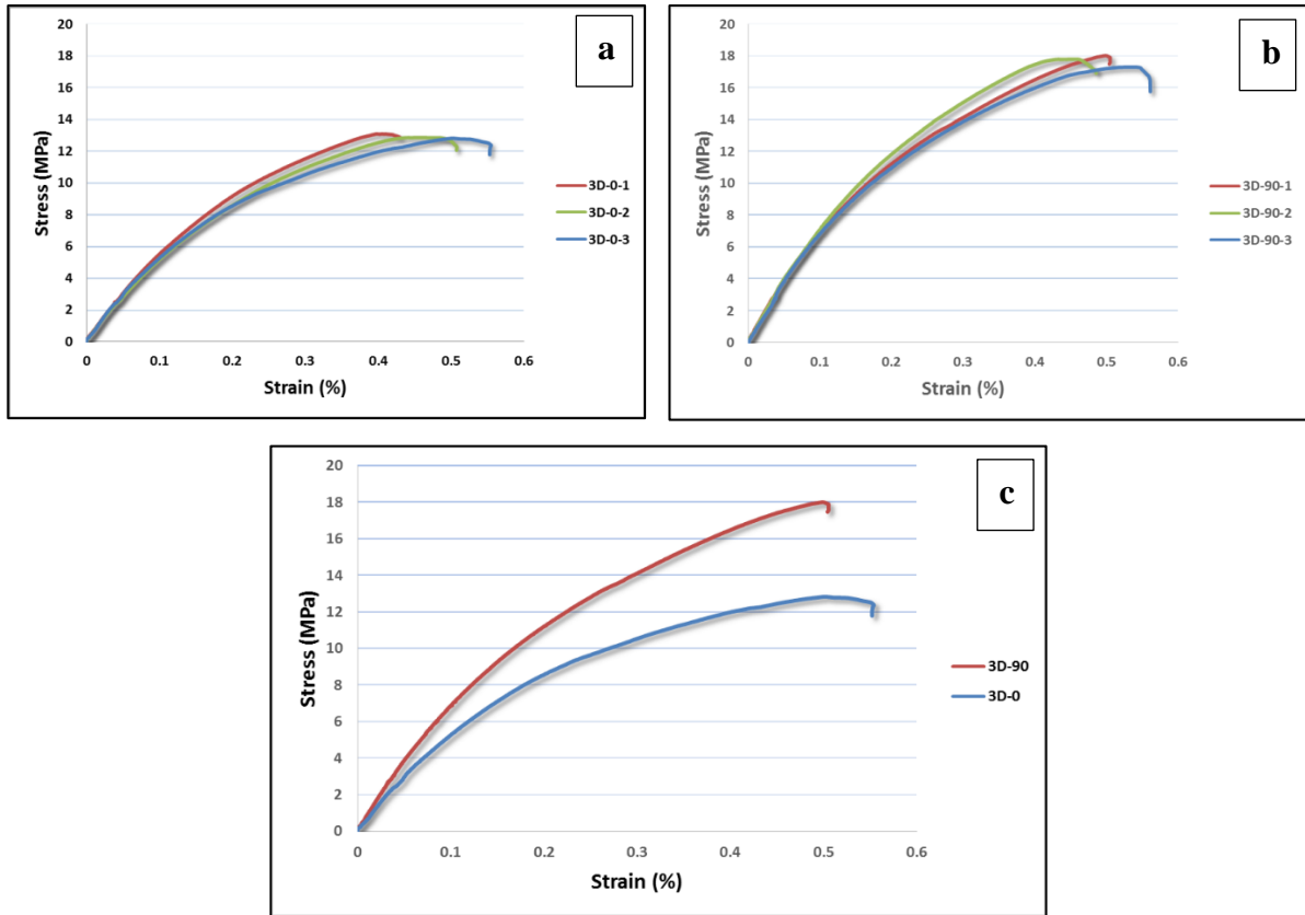
Figure 6-2. Stress-strain curves of 3D warp ( 0^\circ ) and weft ( 90^\circ ) composite specimens, (a) three curves for 3D warp ( 0^\circ ), (b) three curves for 3D weft ( 90^\circ ), (c) average curves of warp and weft specimens, tensile strength in weft direction is 35.4% higher than warp
