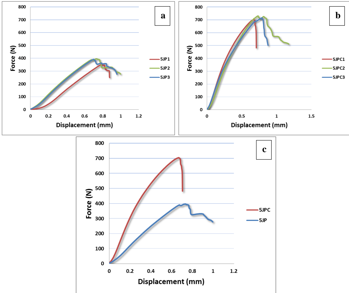
Figure 4-17. SBS curves of 5-layered non-commingled and commingled 2D composites, (a) three dispersion curves of 5-layered non-commingled (5JP) composites, (b) three dispersion curves of 5-layered commingled (5JPC) composite, (c) a comparison of 5JP and 5JPC, 5JPC 81% stronger
