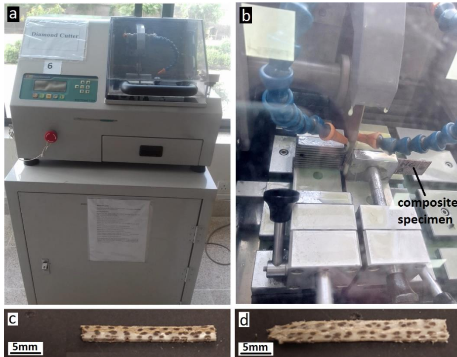
Figure 5-5. (a) Besttom T200 diamond cutting machine, (b) close-up view of composite specimen cutting, (c), (d) thin slices (<0.5mm thickness) of instant and gradual specimens respectively
