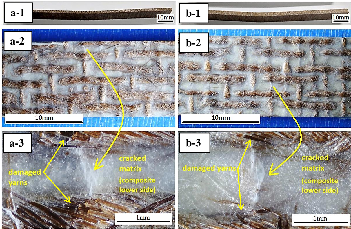
Figure 5-10. Tested samples of non-broken 3-point bending (a-1, a-2, a-3) instant and (b-1, b-2, b-3) gradual loaded tested specimens
