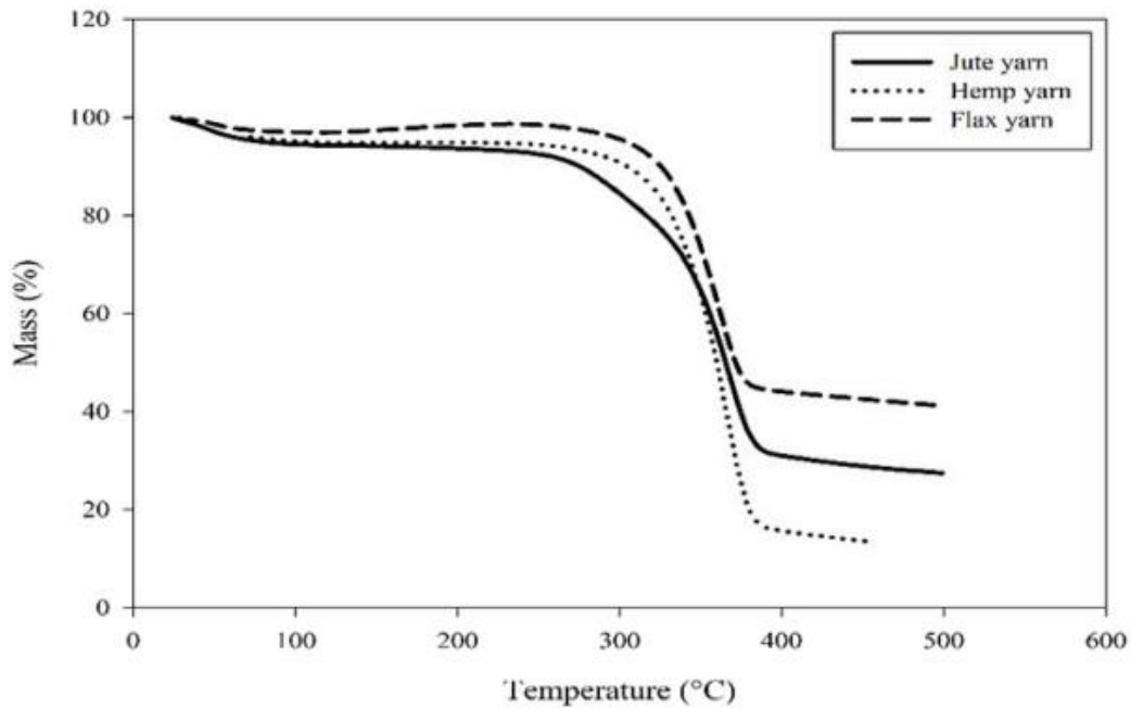
Figure 1-12. TGA curve for hemp, jute and flax fibers showing stability of these fibers upto 200^{\circ}\text{C} , initial weight loss under 100^{\circ}\text{C} is due to moisture evaporation[75]
