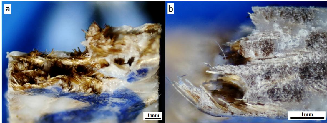
Figure 6-9. Microscopic image of Charpy impact tested samples of 3D orthogonal commingled specimens, (a) fracture face (b) side view
