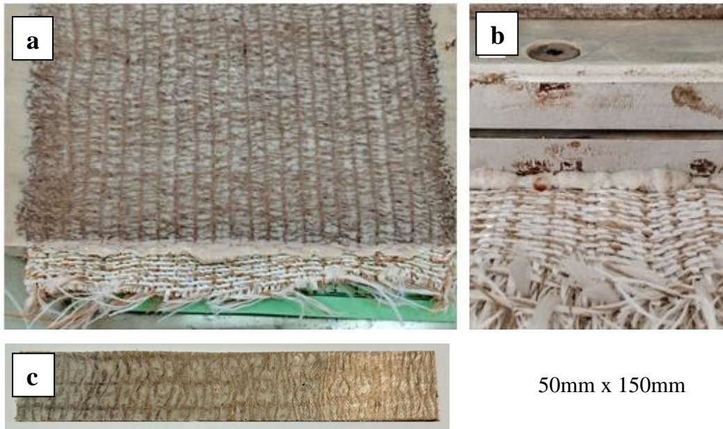
Figure 2-23. (a) The 3D woven commingled jute/PP composite sample after fabrication, (b) zoomed-in view during fabrication, (c) tensile sample ready for testing
