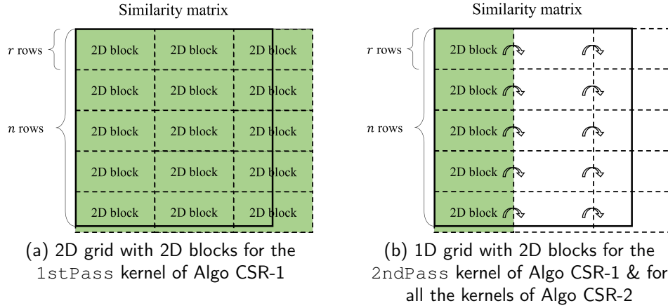
Figure C.1: Grid and block configuration of the CUDA kernels for CSR format similarity matrix construction
