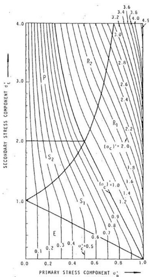
FIGURE I.29 – Diagramme de O'Donnell Porowski [O'Donnell and Porowski, 1979]
