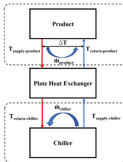
Figure 12: Physical emulation of the heat load in the test bench heat exchanger
