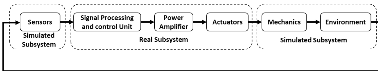
Figure 3: Power Hardware-In-the-Loop(PHIL)[20]
