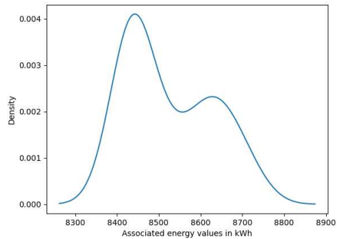
Figure 154: Distribution of energy used for space heating
