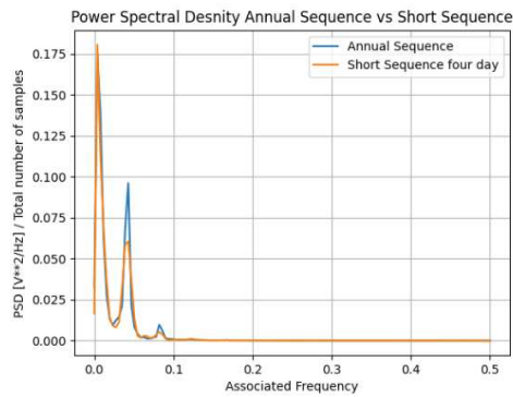
Figure 107: PSD heating season vs 4-days short sequence
