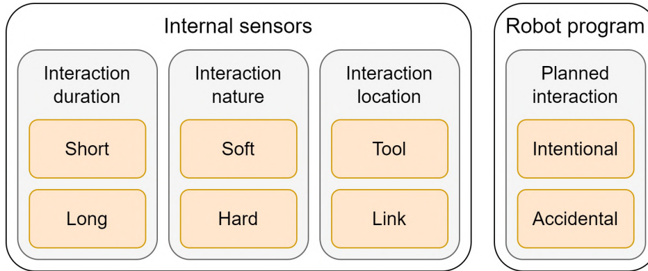
Figure 5.2: Diagram of interaction classes. By using the robot internal sensors only it is possible to determine interaction duration, nature, and location. The possibility of intentional or accidental interaction could be predefined by the robot program.
