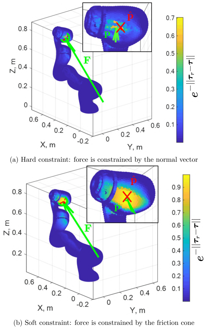
Figure 2.8: Estimation of the interaction force application point using different constraints. In the first step, the hard constraint is used to find an initial estimation, which is further replaced by the soft constraint to obtain the desired interaction parameters. The green arrow denotes the real interaction force; the red cross shows the obtained force application point.
