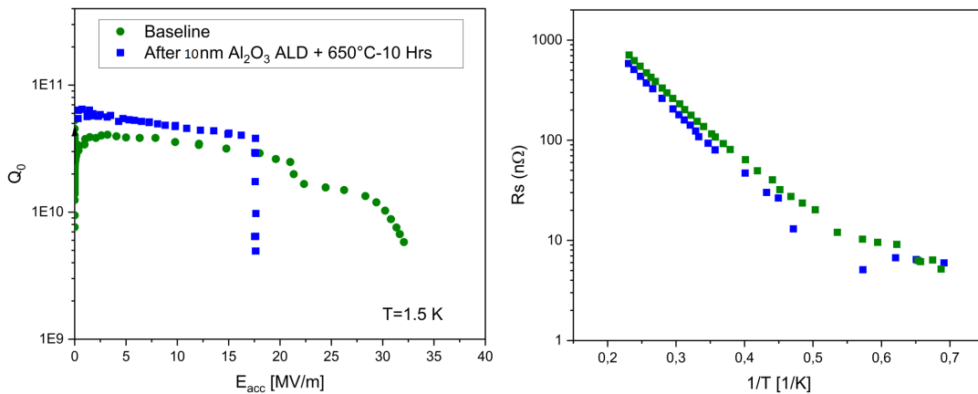
Figure 5.20: Summary of the RF tests done on Al 2 O 3 coated Nb cavity after annealing at 650°C during 10 hours in UHV
