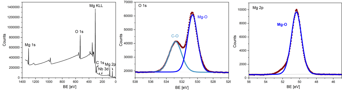
Figure 5.6: XPS analysis of 8.5 nm thick MgO film on niobium substrate
