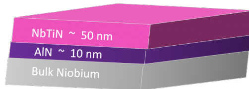
Figure 7.2: the multilayer structure studied in this project
