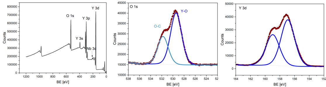
Figure 5.7: XPS analysis of 7.5 nm thick Y_2O_3 film on niobium substrate
