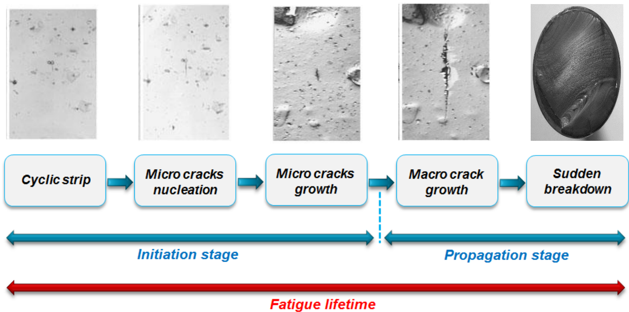
Figure I. 4. Stages of the Fatigue failure (After (Dowling, 2007))
