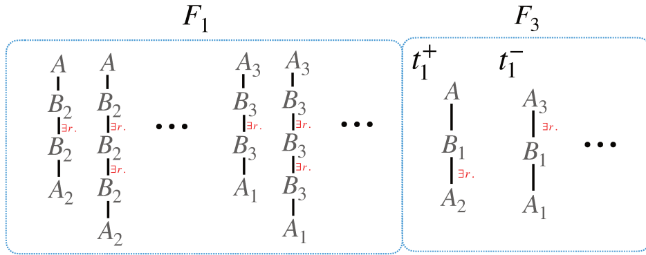
Figure 4.5: some trees in F_1 and F_3
