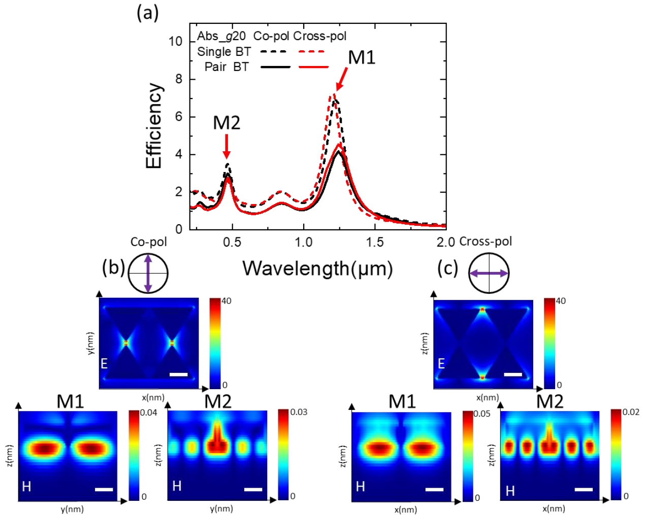
Figure 2. 9. Far-field and near-field comparison between a single and a pair of BT, having a gap of 20nm, under both polarized light (a) Absorption cross-section efficiencies are plotted. On the low-energy side, an additional red-shift of M1 is remarked for the pair of BT regardless of the polarization and the responses appear at the same energetic position even for the mode on the high-energy side. In the near-field, the (b) co- and (c) cross-polarization influence on manipulating the E-field distribution is studied. A similar E-field magnitude is presented in the xy -plane at \lambda= 1.243 \mu\text{m} regardless of the polarization direction (b, c). H-field magnitudes within the spacer are illustrated in the cross-sectional yz -plane for the tip-to-tip area (b) and cross-sectional xz -plane for the corner-to-corner area (c), respectively at \lambda= 1.243 and 0.472 \mu\text{m} (red arrows) showing the presence of 2 different modes (lobes formation). All scale bars are 100 nm long.
