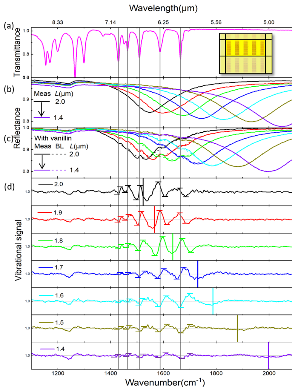
Figure 5. 4. Resonant SEIRA sensing demonstration of vanillin using Al-BT. (a) Transmittance spectrum of vanillin (50mg/ml) normalized to the one of cleaned KBr platelet, shown as a reference. Gray vertical lines eye-guide the IR absorption lines of vanillin. The inset shows an FPA image of the 5 zones of Al-BT selected by a manual knife-edge covering 230 \mu\text{m} \times 90 \mu\text{m} . Reflectance spectra of the Al-BT of different side lengths L varying from 2.0 to 1.4 \mu\text{m} with a step of 0.1 \mu\text{m} , covering accordingly a wide spectral range from 1 400 to 2 100 \text{cm}^{-1} are acquired before (b) and after (c) the deposition of vanillin. The dashed curves are the corresponding baseline (BL) fitted using Euler's smoothing algorithm, excluding the vibrational features (Fano-type). 131 (d) Vibrational signals normalized by the BL for each BT array (side length L given in microns). The plasmonic resonance positions \omega_{res} are marked with thick colored vertical lines. The signal strengths of the enhanced molecular vibrational modes (S-shape) are obtained as a peak-to-peak value, delimited by the horizontal ticks. Note the signal strength and the line shape of a given vibrational mode change depending on its frequency compared to \omega_{res} .
