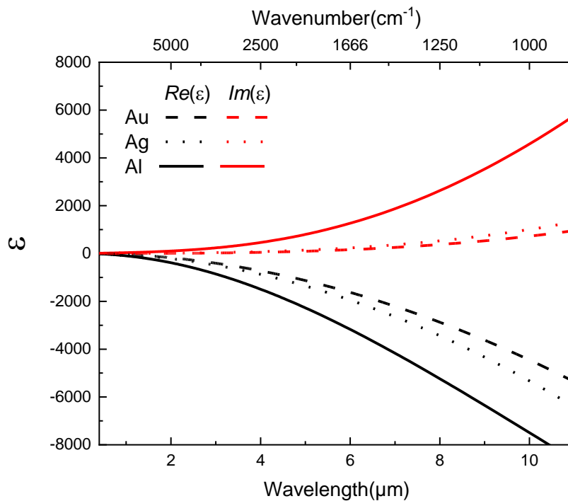
Figure 1. 10. Real ( Re ) and imaginary ( Im ) parts of the dielectric function ( \epsilon ) for Au, Ag and Al along the IR range, provided by CRC Handbook of Chemistry & Physics by E. Shiles. 62
