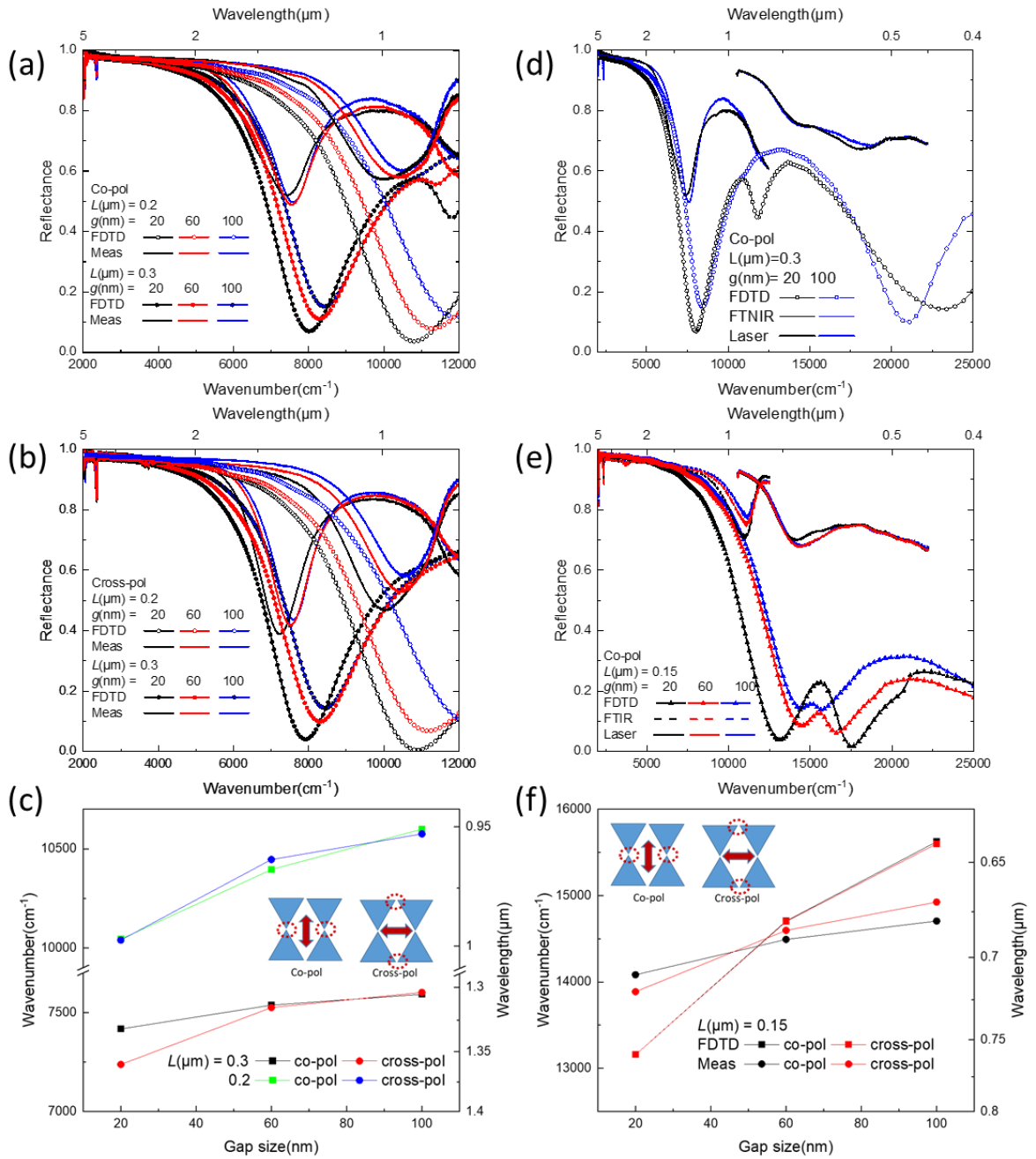
Figure 4. 2. The reflectance measurements of Al BT covering (a) the NIR with L = 0.2 and 0.3 μm under a co-pol and (b) under a cross-pol. The spectral tendency to red-shift is revealed in (c) for the respective L and g variations, regardless of the light polarization. The numerical and experimental results are in good agreement. The inset shows the light polarization as well as the activated sites of the occurring coupling. The measurements are extended to the visible for L = 0.3 μm in (d) and for L = 0.15 μm in (e). The reflectance spectra which are presented in the visible are also background corrected. The spectral influence of g on the LSPR for L = 0.15 μm is shown in (f) and further studies are continuing on these results in the visible range.
