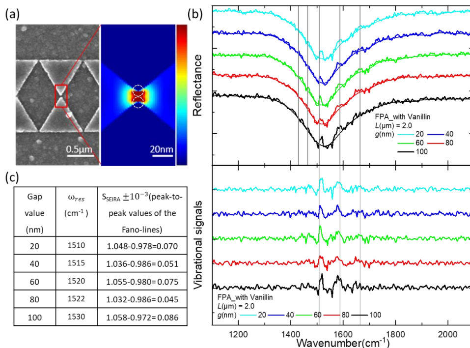
Figure 5.3. Gap influence on the SEIRA analysis. (a) SEM image of the fabricated BT NA with a gap of 20 nm and the resulting near E-field localization and enhancement under a co-polarized light. The dotted circles (radius = 8 nm) give a better visualization of the activated zones where the molecules are strongly coupled. (b) FPA results show the gap spectral influence on the \omega_{res} of BT arrays with L = 2.0 \mu\text{m} during the SEIRA sensing, and (c) the resulting background-corrected vibrational signals for each vanillin vibrational mode vertical line. \omega_{res} are defined for each gap value and S_{SEIRA} is calculated for \omega_{vib} = 1509 \text{ cm}^{-1} .
