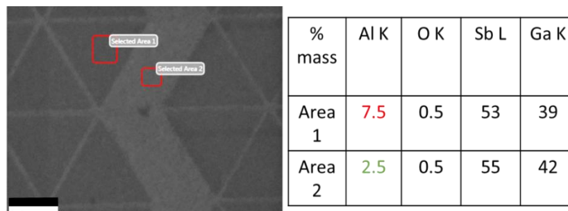
Figure.A.3. 9. EDX analysis of the SEM image of the physically etched HC transferred to the Al layer (area 1) and surrounded by the doped GaSb layer (area 2) grown on an undoped GaSb substrate. The scale bar is 10 \mu\text{m} long. As detailed in the associated table, Area 2 is revealing a considerable percentage of Al due to insufficient etching time.
