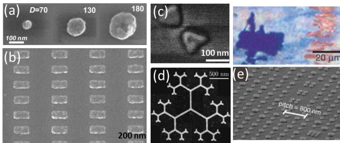
Figure 1. 11. State-of-art Al nanostructures fabricated by EBL. (a) Nanodisks on \text{SiO}_2 for UV-Vis coverage. 61 (b) Nanorods on \text{KTaO}_3 for transmittance measurements from UV to IR. 66 (c) Bowtie on silica formed by two equilateral triangles of 100nm side length with 20nm apex to apex gap distance, for benzene detection using UV-SERS. 69 (d) Caylee tree on \text{Si}_3\text{N}_4 promoting a wide range of applications. 75 (e) Nanopillars on Al for plasmonic painting application in the UV as for Monet's impression, Soleil levant. 76
