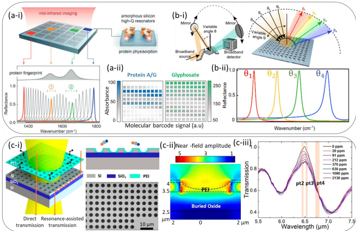
Figure 1. 15. All-dielectric-based platforms for spectroscopy. Tittl et al. proposed (a-i) Two tilted amorphous Si ellipses, designed as pixelated metasurfaces, having high-Q resonances, used for spatially encoding the spectral absorption fingerprint information of molecules. (a-ii) Imaging-based read out of this information produces a molecular barcode signal suitable for chemical identification in a target analyte, as for protein A/G and glyphosate. 102 An extra tunability degree is proposed by Leitis et al. (b-i) Angle variation achieved by a simple moving mirror system, combined with the spectral selectivity of high-Q resonances of germanium ellipsoids, permits a broadband activation and an angle-to-plasmonic resonance correlation, for better control of the detection selectivity. 103 A promising sensing capability is stated by Chang et al. for gas sensing using (c-i) a Si-based photonic crystal slab covered with polyethylenimine (PEI) sustaining guided resonances for carbon dioxide sensing. (c-ii) Strong surface sensitivity is numerically confirmed by the calculated electromagnetic near-fields. (c-iii) Experimental investigation of CO 2 detection in the ppm range. 104
