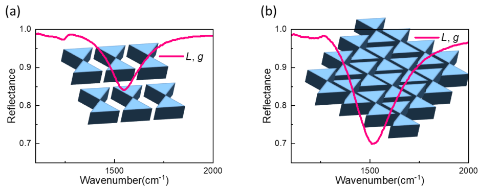
Figure 4.9. The arrangement influence on the reflectance of (a) the BT and (b) the HC NA (insets), illuminated under a co-pol light source. In both cases, L and g are respectively fixed at 2.0\mu\text{m} and 100 \text{ nm} . For a compact arrangement, the LSPR is more pronounced in terms of amplitude and it is slightly red-shifted compared to the one of the BT, as more resonators are interacting.
