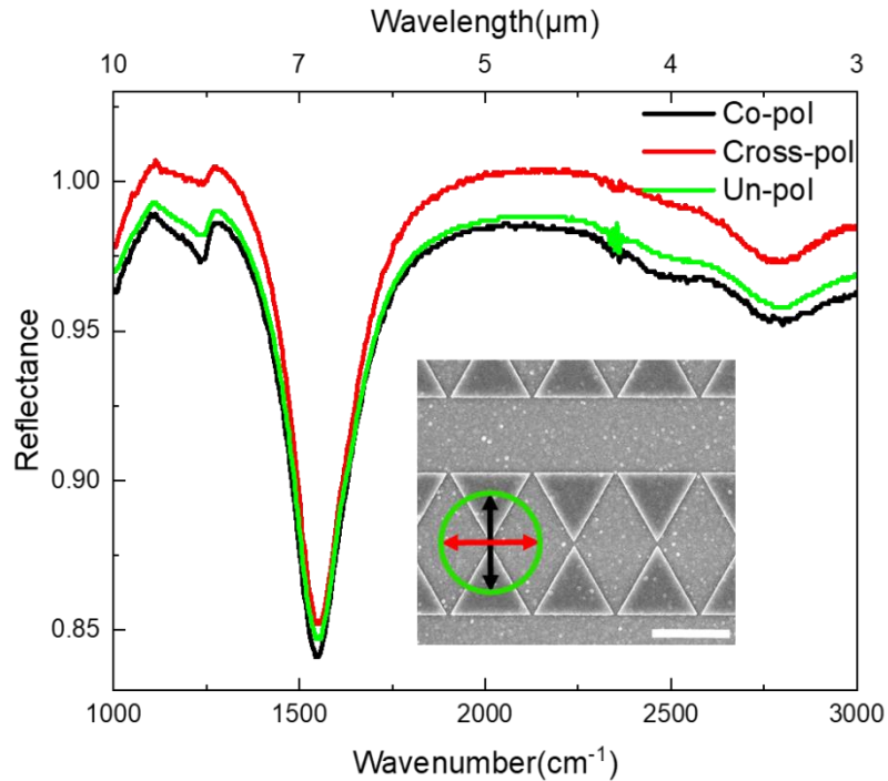
Figure 4. 5. Polarization influence on the reflectance spectra of the BT NA illuminated under a co-pol, cross-pol, and un-pol light source. The inset shows the SEM image of the fabricated BT with L = 2.0\ \mu\text{m} and g = 100\text{ nm} , as well as the direction of the E-field in each case. The scale bar is 2.0\ \mu\text{m} long.
