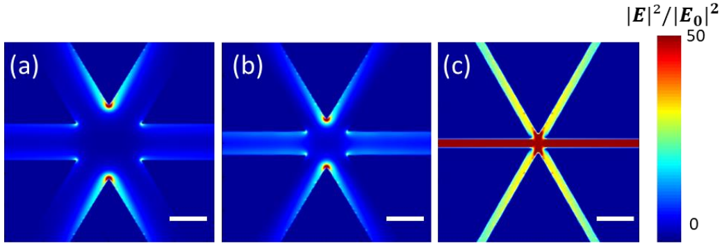
Figure 2.19. Gap value influence on the local field enhancement and intensity for L = 0.8 \mu\text{m} with g equal to 100, 60, and 20 nm. Under a co-polarized light, the enhanced electric field mapping is collected in the xy -plane (a) for g = 100 nm calculated at \lambda = 3.3 \mu\text{m} , (b) for g = 60 nm calculated at \lambda = 3.37 \mu\text{m} , (c) for g = 20 nm calculated at \lambda = 3.5 \mu\text{m} . The color scale ranging from blue to red indicates the minimum to maximum field intensity |E|^2/|E_0|^2 , \max(|E|^2/|E_0|^2) equals 250, 233, 216 while decreasing the g value. For better contrast, the maximum color scale is fixed at 50. All scale bars are 100 nm long.
