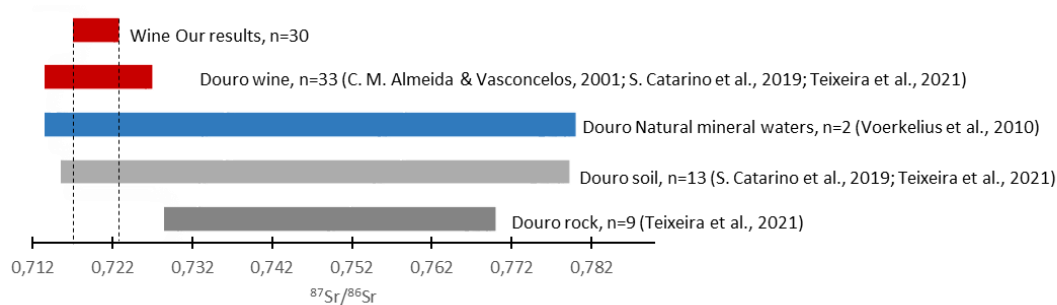
Figure 20. Range of values of ^{87}\text{Sr}/^{86}\text{Sr} for wines, soil, rocks and water from Portugal, as reported in literature. References: ( Almeida & Vasconcelos, 2001) (Teixeira et al., 2021) ( Catarino et al., 2019) (Voerkelius et al., 2010) (Ribeiro, Azevedo, Santos, Medina, & Costa, 2014)
