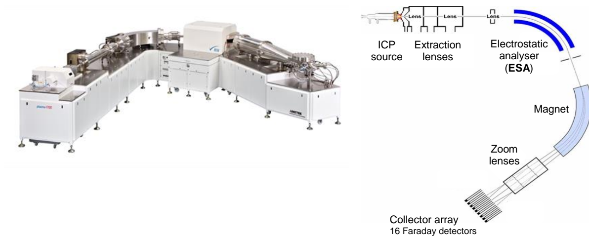
Figure 7. Nu Plasma 1700 and schematics of an MC-ICP-MS instrument. Adapted from (Yang, 2009)
