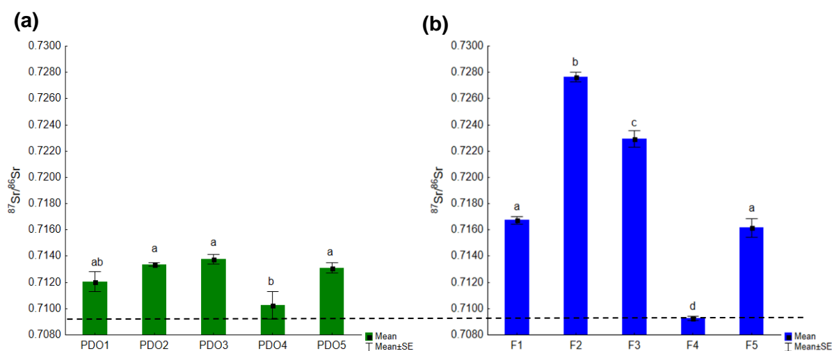
Figure 17. Characterization of the ^{87}\text{Sr}/^{86}\text{Sr} isotope ratio in Rocha pears ( n=50 ). (a) represents the PDO region and (b) the region of Fundão. Producers are identified by numbers from 1 to 5. (----) modern seawater Sr isotope values ^{87}\text{Sr}/^{86}\text{Sr} = 0.70918 (Jones, 2001).
