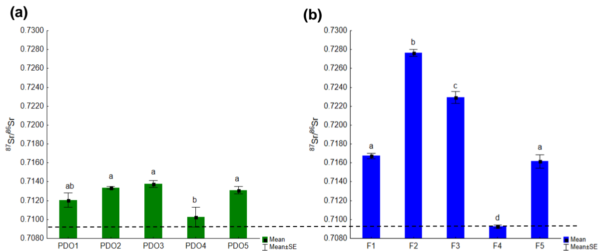
Figure 17. Characterization of the ^{87}\text{Sr}/^{86}\text{Sr} isotope ratio in Rocha pears (n=50). (a) represents the PDO region and (b) the region of Fundão. Producers are identified by numbers from 1 to 5. (----) modern seawater Sr isotope values ^{87}\text{Sr}/^{86}\text{Sr} = 0.70918 (Jones, 2001).
