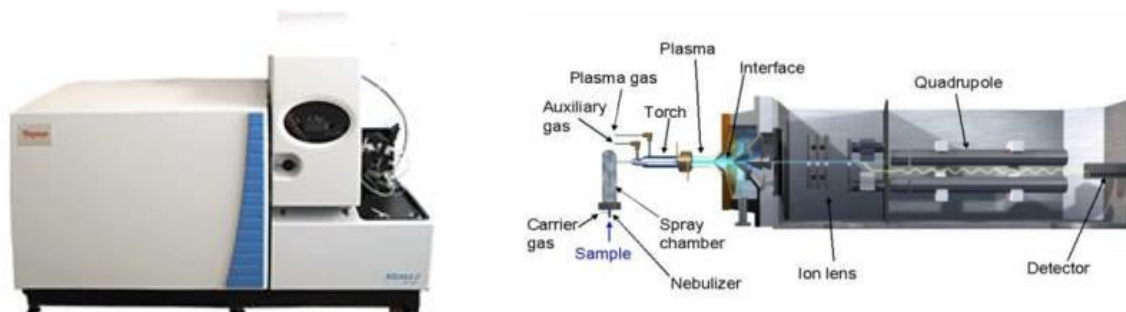
Figure 5. Thermo X Series II and schematics of a quadrupole ICP-MS (UC Davis, 2020).
