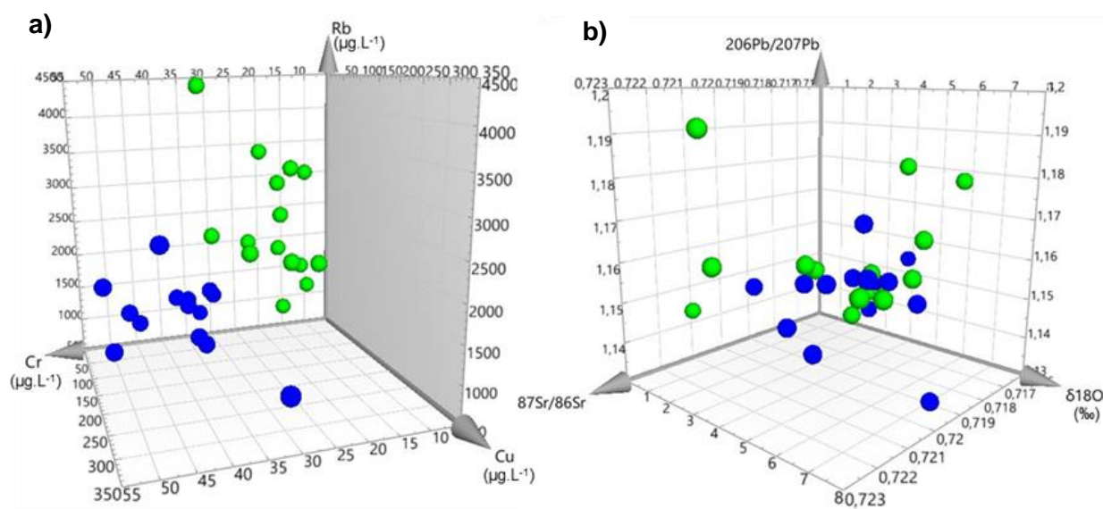
Figure 24. A 3-D plot of (a) discriminant parameters process-oriented by type of wine and (b) non-discriminant isotope ratios.
