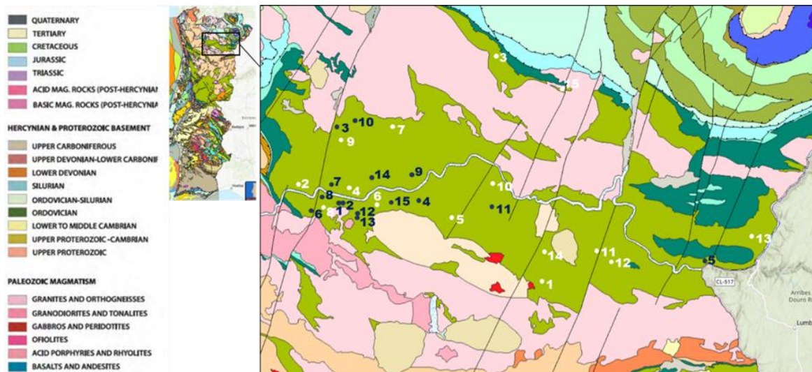
Figure 18. Geological map of Portugal highlighting the Douro Demarcated Region with the location of the selected Quintas . Blue numbers represent samples of Port wine (n=15). White numbers represent samples of Douro wine (n=15). Adapted from (LNEG, 2021)
