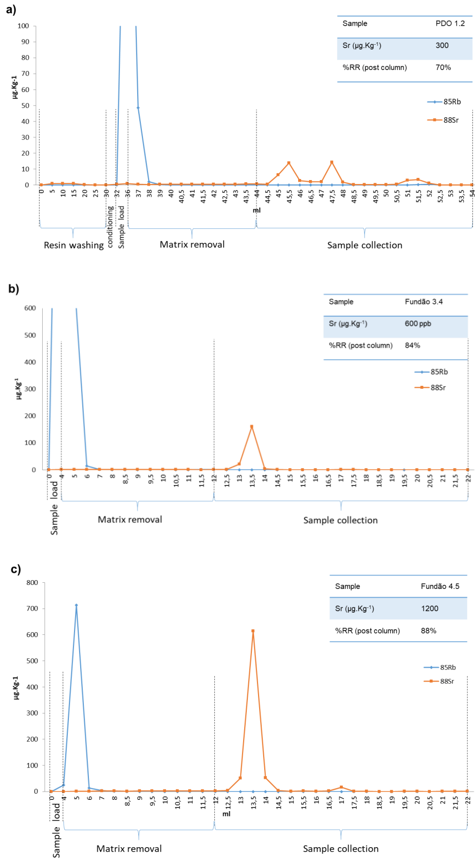
Figure 15. Elution Profiles of pear samples, using Sr-selective resin Eichron® with (a) low, (b) medium and (c) high concentrations of Sr.
