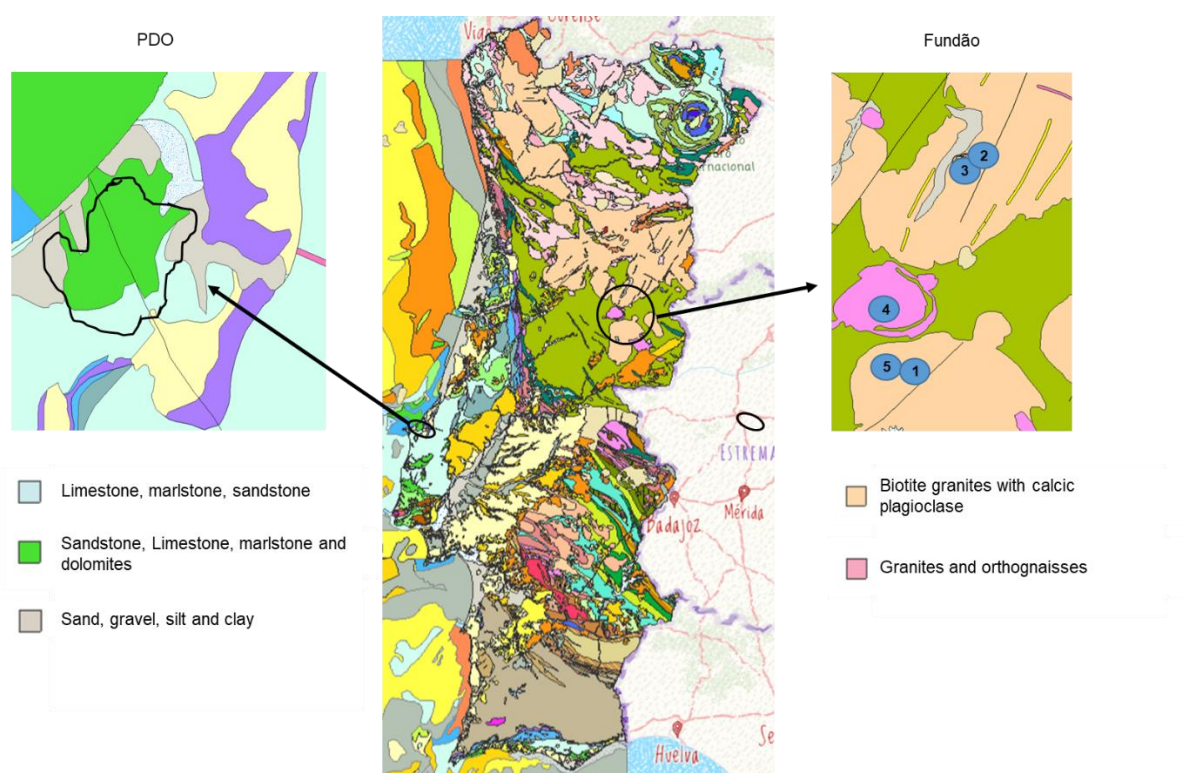
Figure 16. Geological map of the sampling areas of pears. Adapted from (LNEG, 2021).
