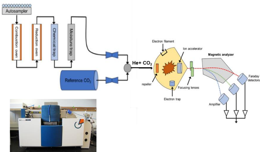
Figure 6. GV instruments isotope ratio mass spectrometer and schematics of an equipment. Adapted from (Won, Yun, Lee, & Shin, 2021).
