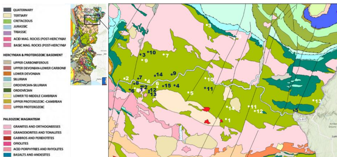
Figure 18. Geological map of Portugal highlighting the Douro Demarcated Region with the location of the selected Quintas . Blue numbers represent samples of Port wine (n=15). White numbers represent samples of Douro wine (n=15). Adapted from (LNEG, 2021)
