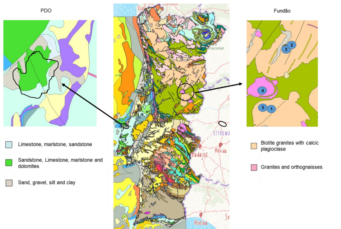
Figure 16. Geological map of the sampling areas of pears. Adapted from (LNEG, 2021).
