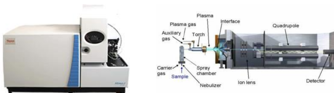
Figure 5. Thermo X Series II and schematics of a quadrupole ICP-MS (UC Davis, 2020).
