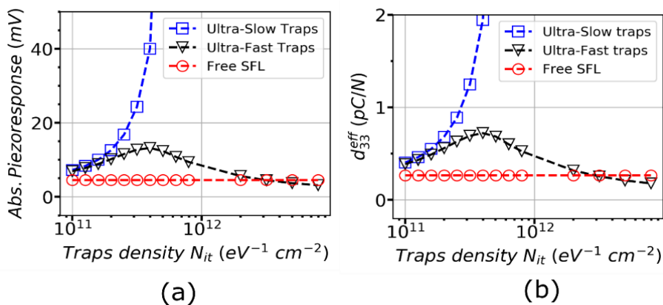
Figure II-10 (a) Piezoresponse in “Press action” mode obtained under three different assumptions at ZnO surface. (b) Comparison of the d_{33}^{eff} piezoelectric coefficient considering ultra-slow traps and ultra-fast traps as a function of trap density in “Press” action mode. In these graphs we considered: ultra-slow traps ( \square ) and ultra-fast traps ( \triangle ). The free SFL (no traps) is plotted for reference ( \odot ). Everything was made for doping concentration N_d = 10^{17} cm -3 and force applied of 126 nN (1 MPa).
