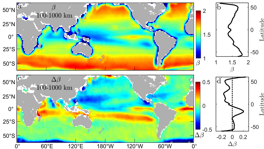
Figure 3.23 (a) The global distribution of \beta measured from ten-year QuikSCAT collected U_{10} (100-1000 km). (b) The meridional variations of \beta inside the Pacific Ocean. (c) The global distribution of \Delta\beta = \beta_s - \beta_w , where \beta_s is the summer (June, July, and August) scaling exponent and \beta_w is the winter (December, January, and February) scaling exponent. (d) The meridional variations of \Delta\beta inside the Pacific Ocean. The dashed line indicates a reference with the value of 0.
